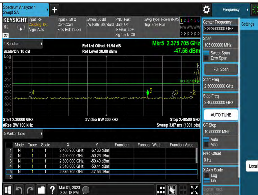
DH5-Ant1-Low-Hop_2402--6.13
