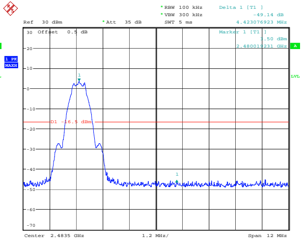
BLE_1M_High_Channel
