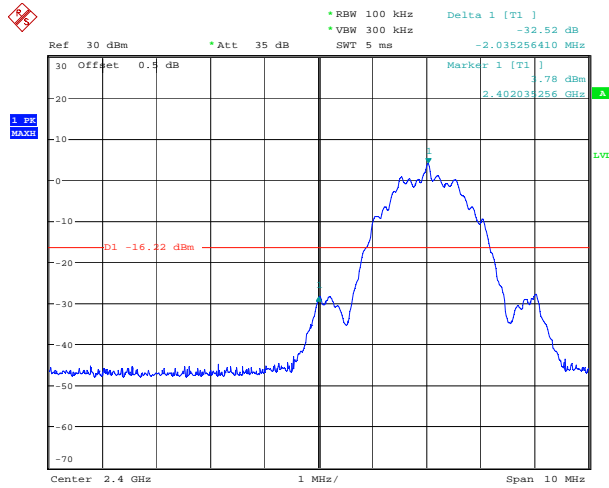
BLE_2M_Low_Channel
