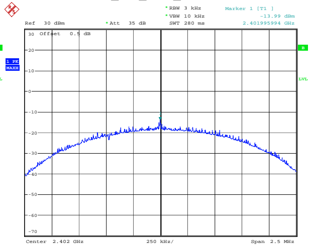
BLE_2M_Low_Channel
