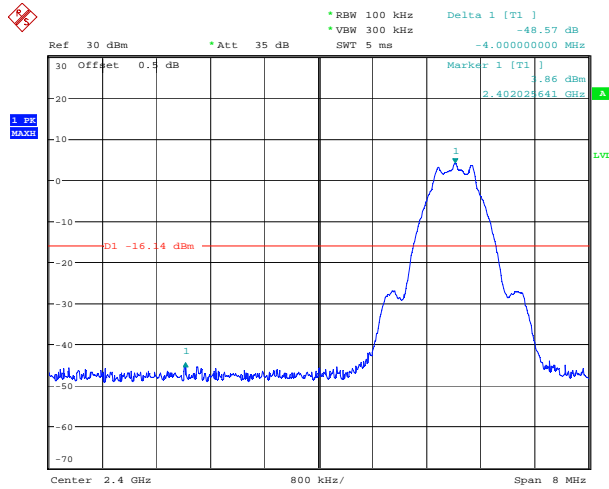
BLE_1M_Low_Channel
