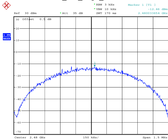
BLE_1M_High_Channel
