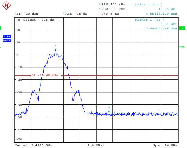
BLE_2M_High_Channel
