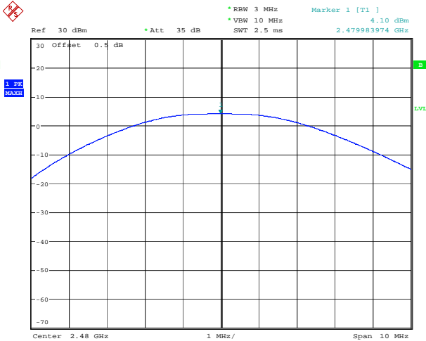
BLE_2M_High_Channel
