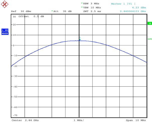
BLE_1M_Middle_Channel
