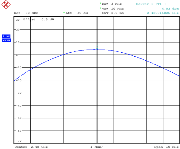
BLE_1M_High_Channel
