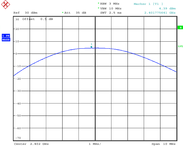
BLE_2M_Low_Channel
