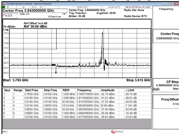
Band77-Part27_50MHz_DFT_s_OFDM_SCS30kHz_BPSK_RB1_132_CH656000
