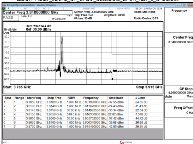
Band77-Part27_50MHz_CP_OFDM_SCS30kHz_QPSK_RB1_0_CH656000
