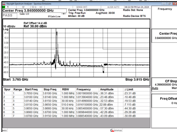
Band77-Part27_50MHz_DFT_s_OFDM_SCS30kHz_BPSK_RB1_0_CH656000
