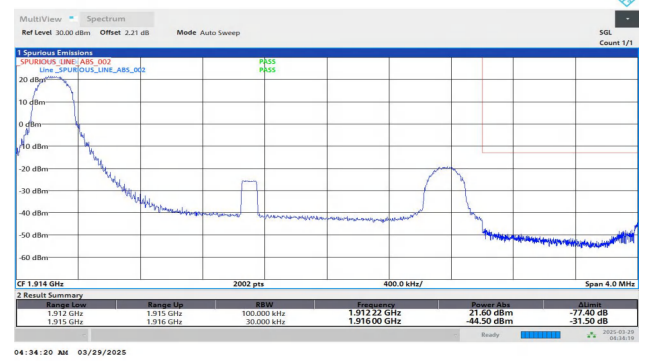
Band25-3MHz-QPSK-26675-1RB#0-PASS
