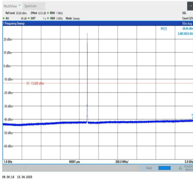
Band25-1.4MHz-QPSK-26365-1RB#5-1000~3000-PASS
