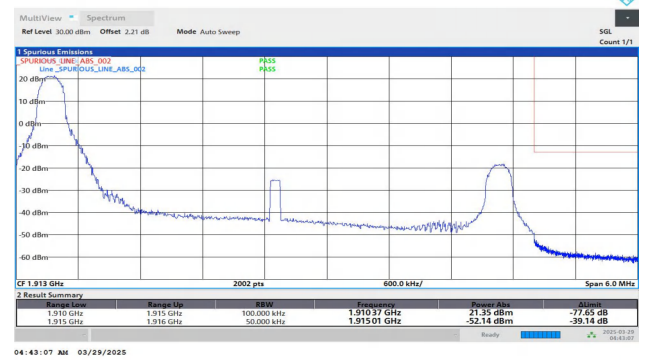
Band25-5MHz-QPSK-26665-1RB#0-PASS
