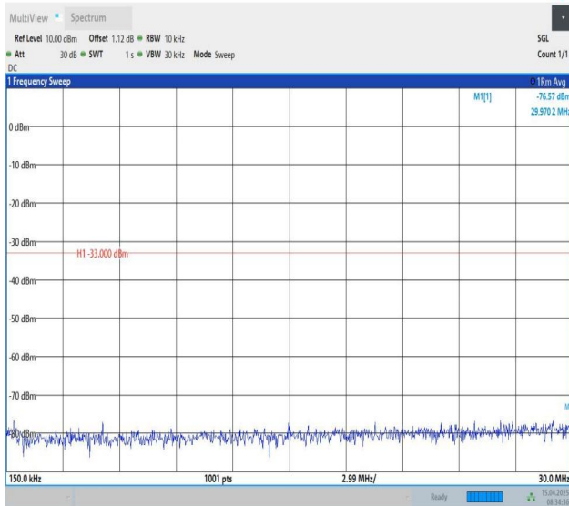
Band25-1.4MHz-QPSK-26047-1RB#5-0.15~30-PASS
