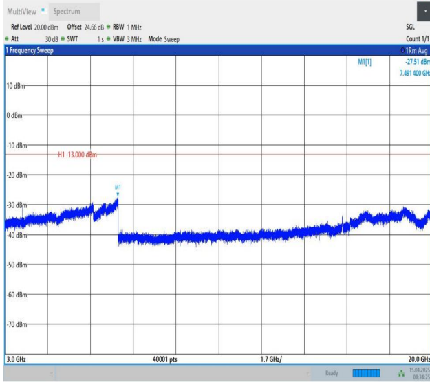
Band25-1.4MHz-QPSK-26047-1RB#0-3000~20000-PASS
