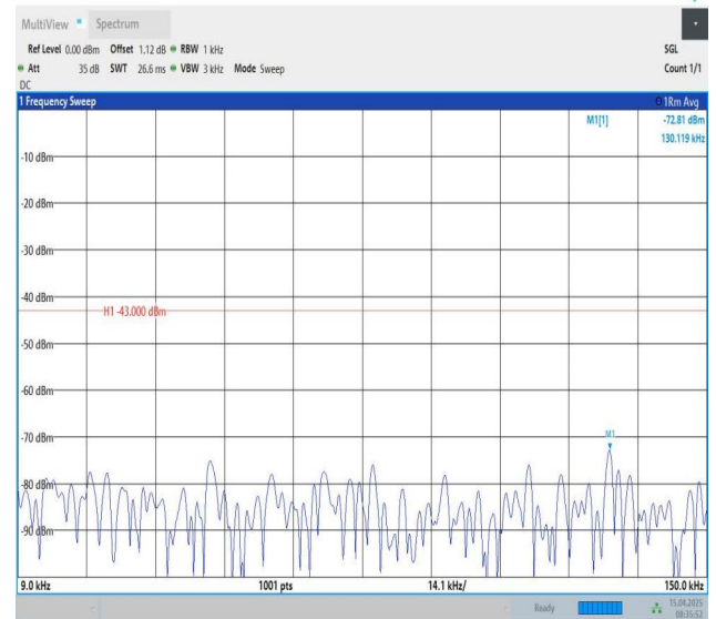
Band25-1.4MHz-QPSK-26365-1RB#5-0.009~0.15-PASS
