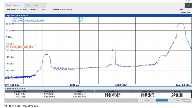
Band25-5MHz-QPSK-26065-1RB#24-PASS
