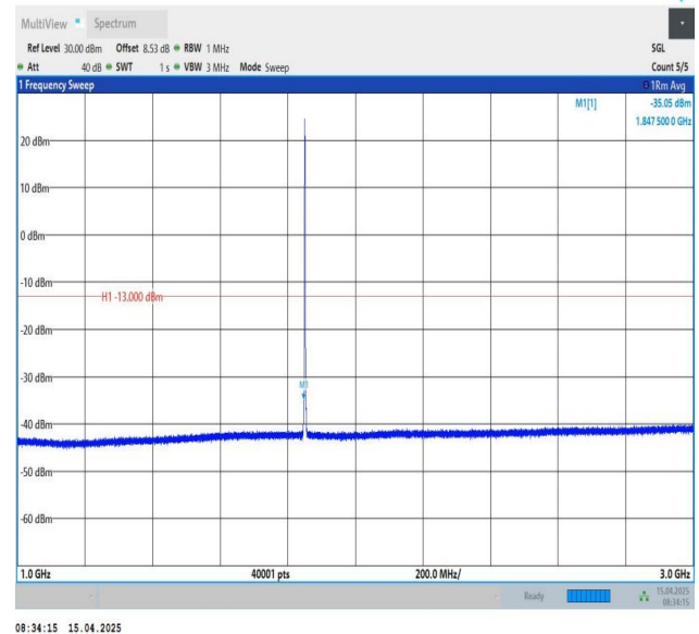
Band25-1.4MHz-QPSK-26047-1RB#0-1000~3000-PASS
