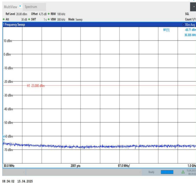
Band25-1.4MHz-QPSK-26047-1RB#0-30~1000-PASS
