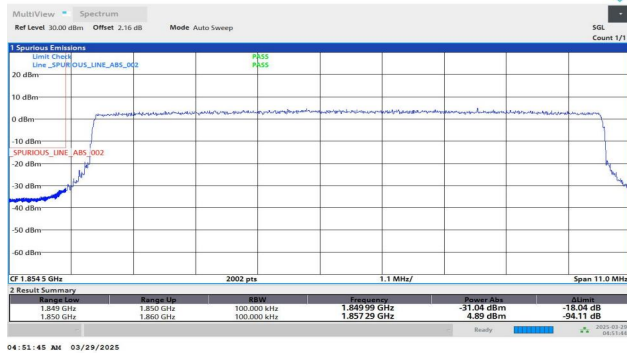
Band25-10MHz-QPSK-26090-50RB#0-PASS
