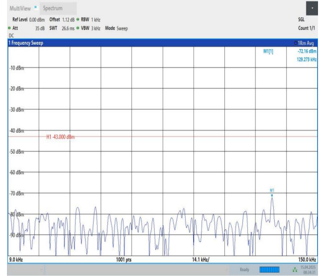
Band25-1.4MHz-QPSK-26047-1RB#5-0.009~0.15-PASS
