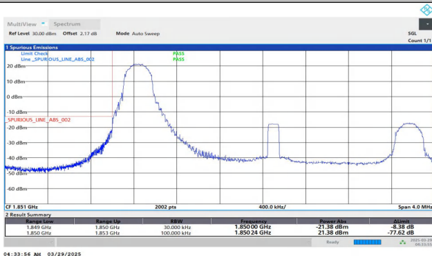
Band25-1.4MHz-QPSK-26047-1RB#0-PASS
