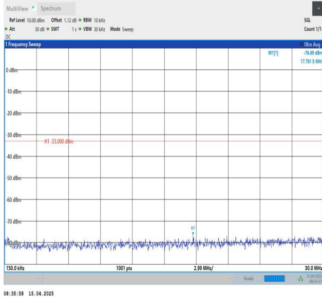
Band25-1.4MHz-QPSK-26365-1RB#5-0.15~30-PASS
