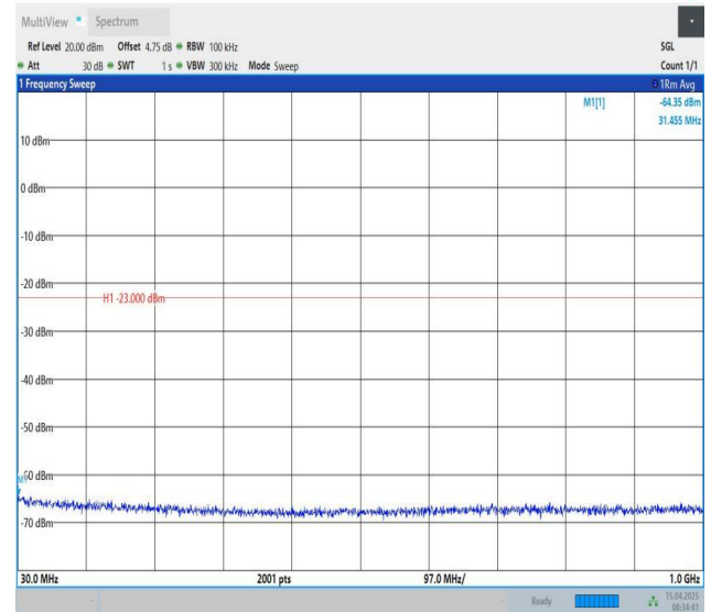
Band25-1.4MHz-QPSK-26047-1RB#5-30~1000-PASS
