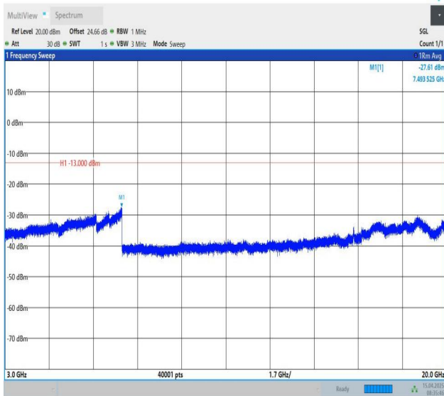
Band25-1.4MHz-QPSK-26365-1RB#0-3000~20000-PASS
