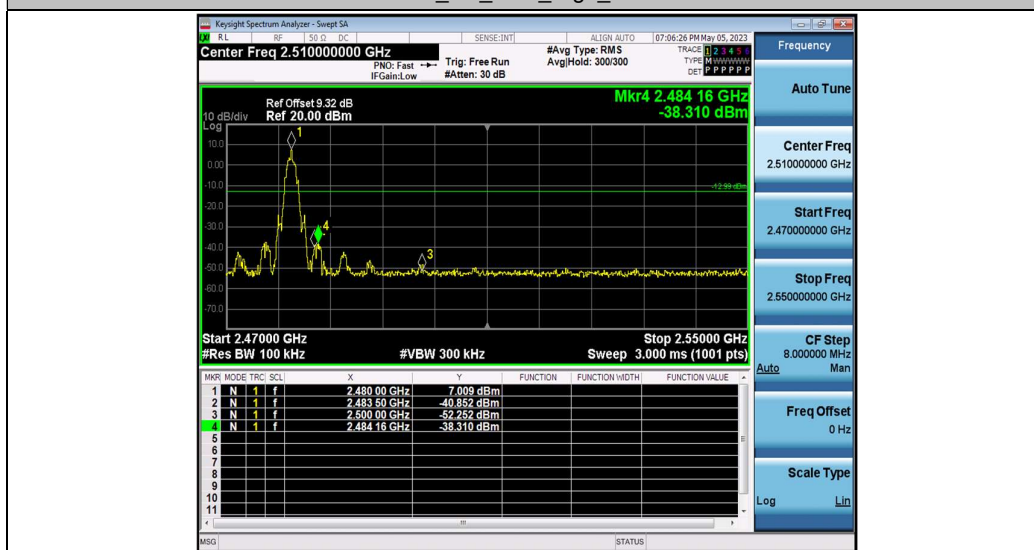
BLE_2M_Ant1_High_2480
