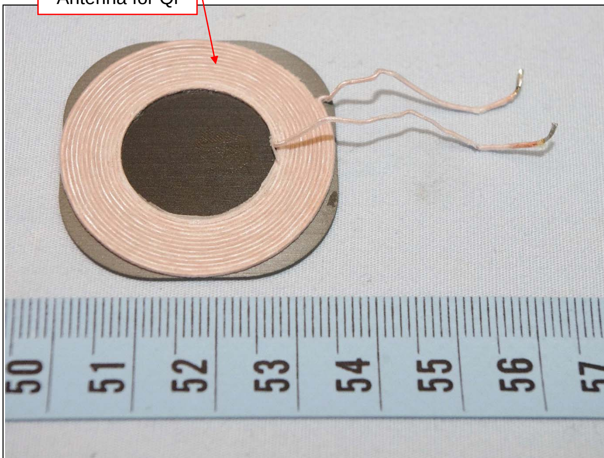
Antenna for Qi
