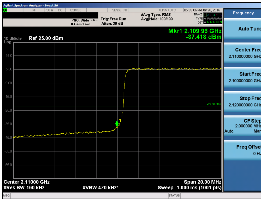
Plot 7-34. Lower Band Edge Plot (Band 4 – 15.0MHz QPSK – RB Size 75)
