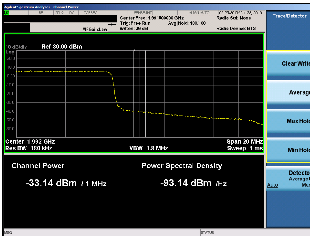
Plot 7-53. Upper Extended Band Edge Plot (Band 2 – 15.0MHz QPSK – RB Size 75)
