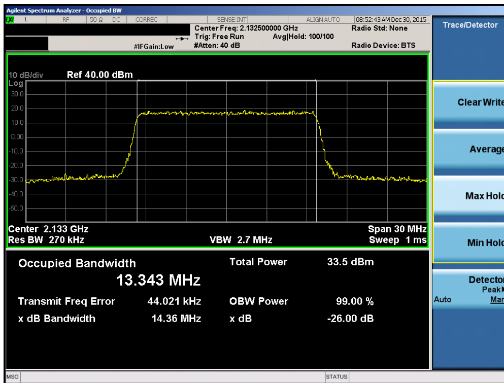
Plot 7-5. Occupied Bandwidth Plot (Band 4 – 15.0MHz QPSK – RB Size 75)
