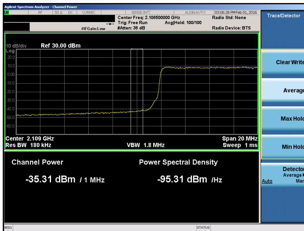
Plot 7-63. Lower Extended Band Edge Plot (Band 4 – 10.0MHz QPSK – RB Size 50)
