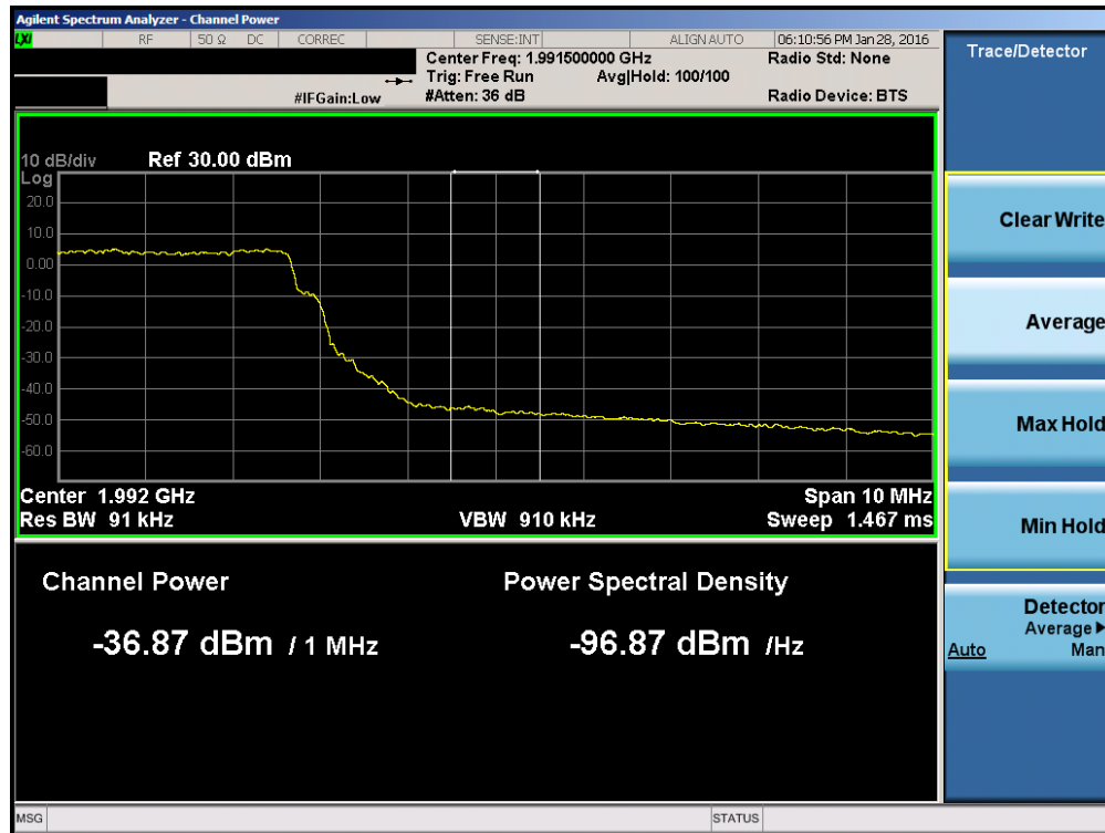
Plot 7-49. Upper Extended Band Edge Plot (Band 2 – 10.0MHz QPSK – RB Size 50)
