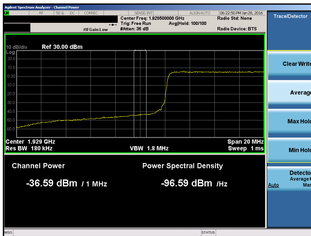
Plot 7-51. Lower Extended Band Edge Plot (Band 2 – 15.0MHz QPSK – RB Size 75)
