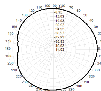
Total(H-XY), Max= -5.19dBi, CirD=9.10
