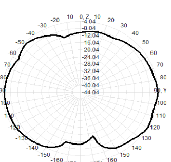
2410.0MHz Total(E2-YZ), Max= -4.77dBi
