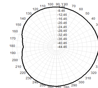
Total(H-XY), Max= -4.86dBi, CirD=9.64
