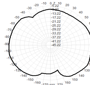
2480.0MHz Total(E2-YZ), Max= -5.22dBi
