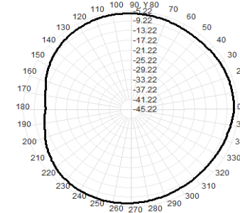
Total(H-XY), Max= -6.26dBi, CirD=7.35
