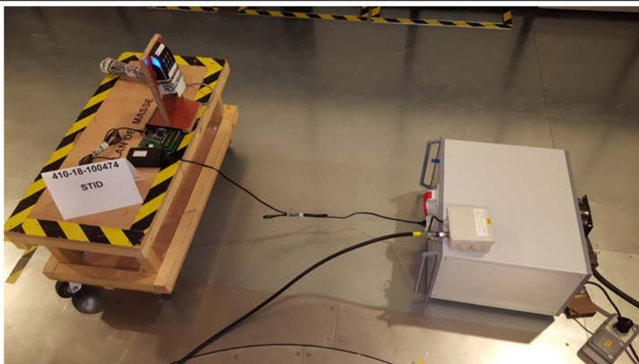
TEST SETUP PHOTO(S) - 110VAC/60HZ POWER SUPPLY / ARCS-I/BT2
