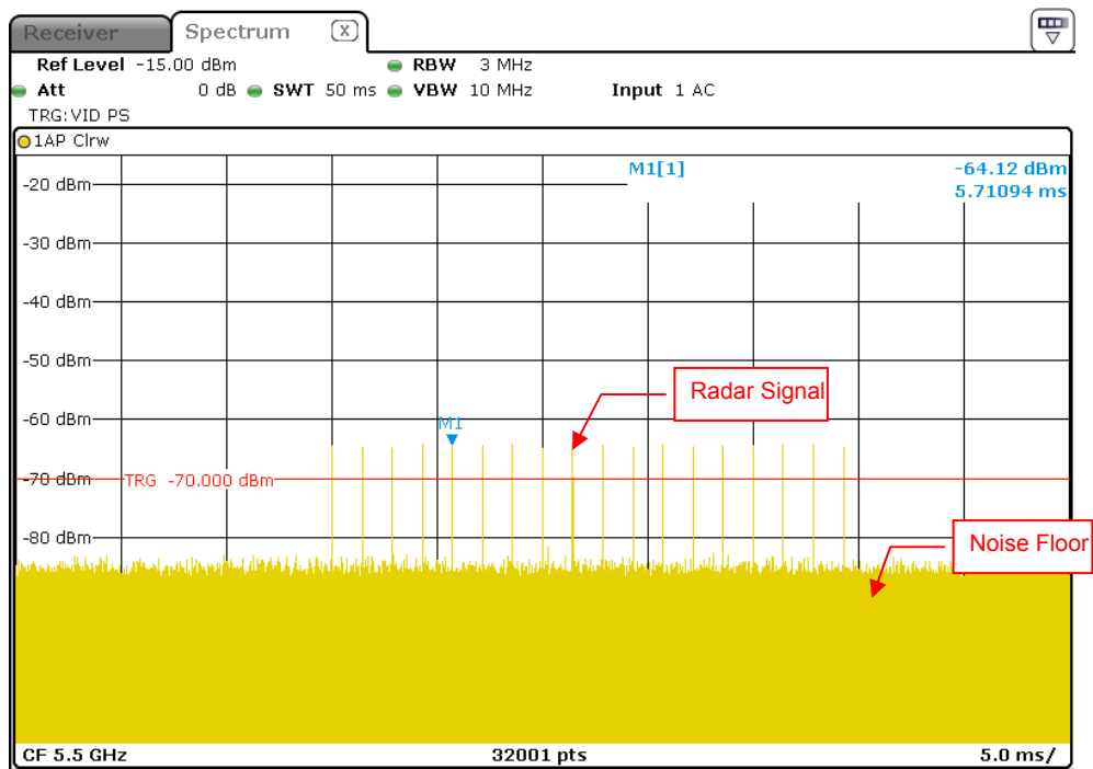
Radar Signal 0
