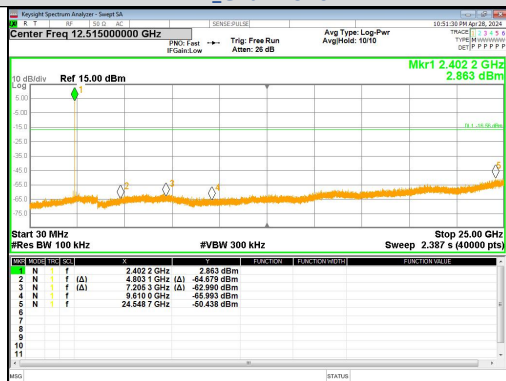
Spurious Emission LE_Channel 0
