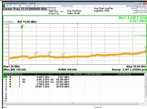
Spurious Emissions LE_Channel 19
