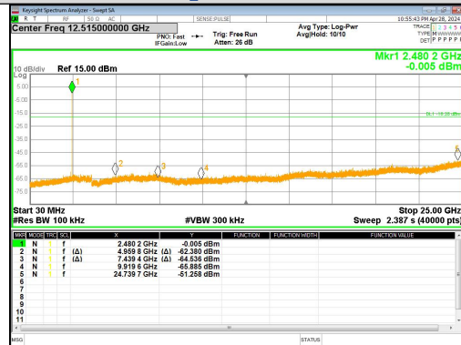
Spurious Emission LE_Channel 39
