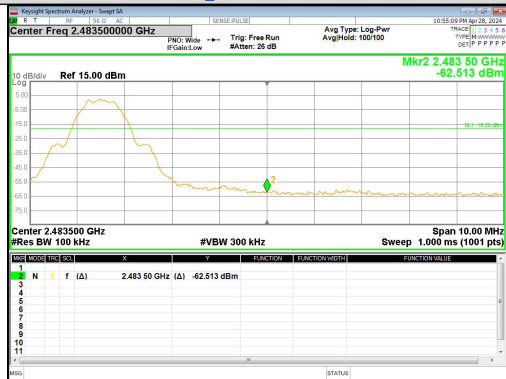
Out Of Band Emission LE_Channel 39
