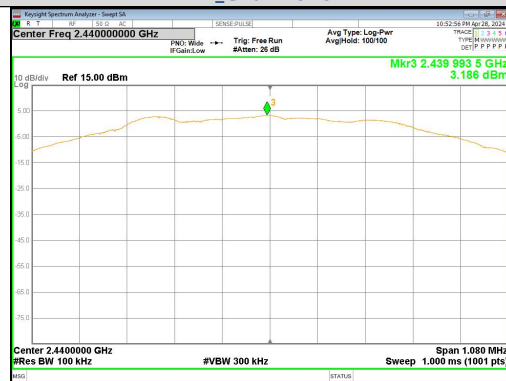
In-Band Reference Level LE_Channel 19
