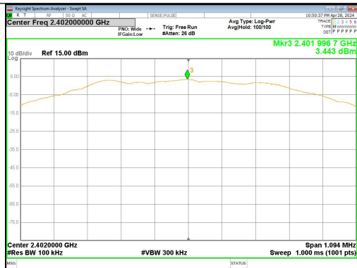
In-Band Reference Level LE_Channel 0
