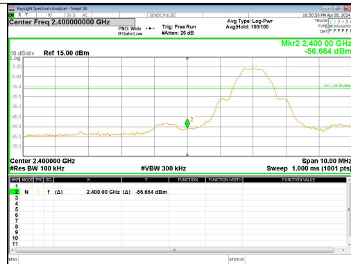
Out Of Band Emission LE_Channel 0
