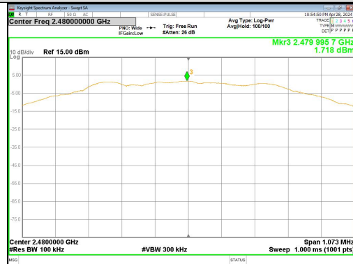
In-Band Reference Level LE_Channel 39
