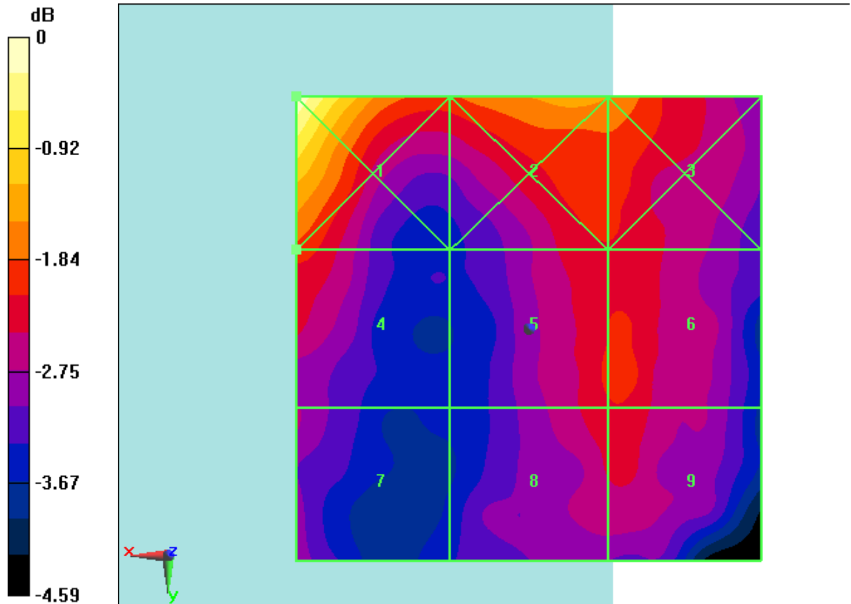
Fig B.24 HAC RF E-Field LTE Band41 Power Class 2 16QAM CH40185
