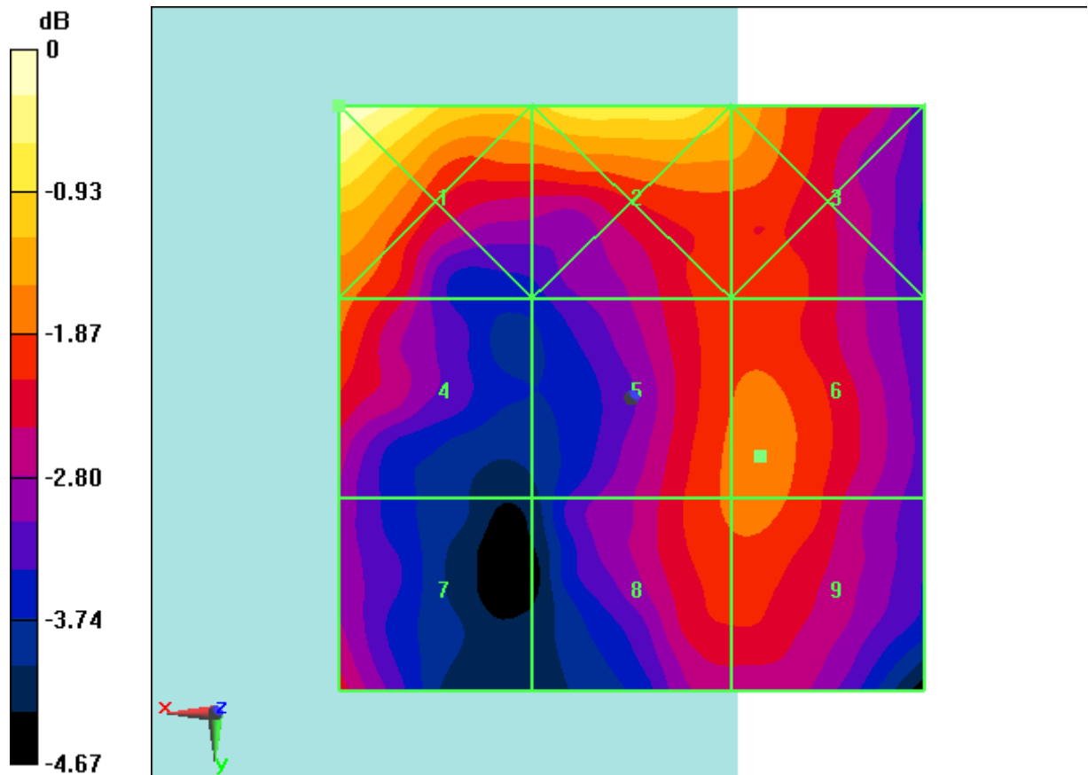
Fig B.26 HAC RF E-Field LTE Band41 Power Class 2 64QAM CH41490
