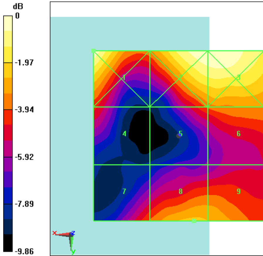
Fig B.19 HAC RF E-Field LTE Band41 Power Class 2 QPSK CH40185
