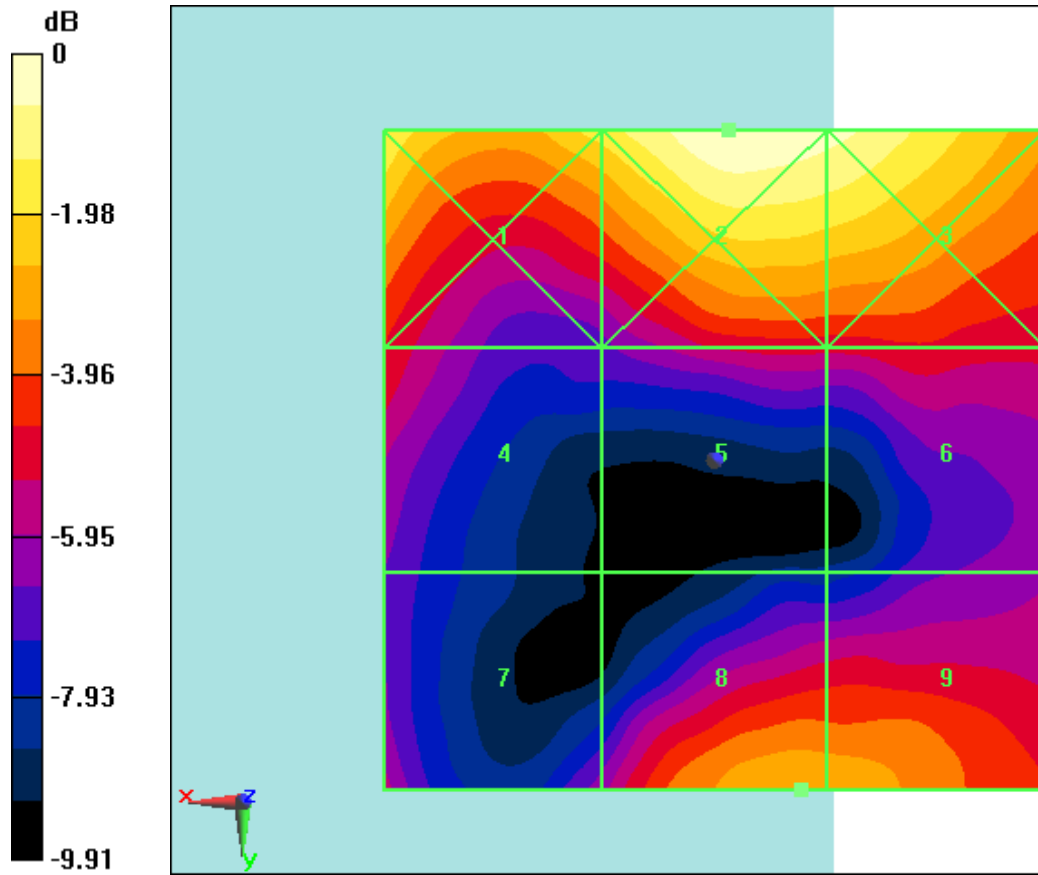
Fig B.43 HAC RF E-Field LTE Band41 Power Class 3 64QAM CH40620
