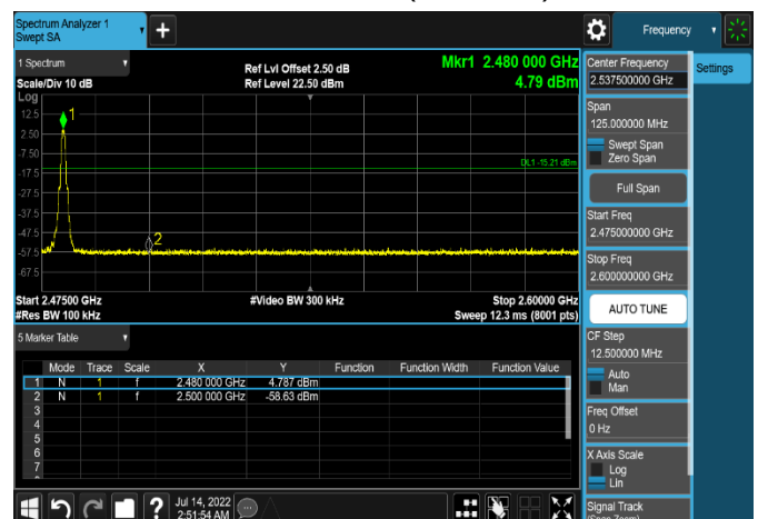
Mode 1 CH39 (2480MHz)
