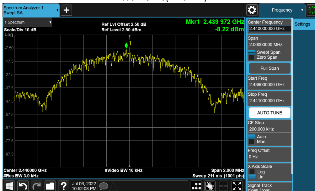
Mode 2 CH19(2440MHz)
