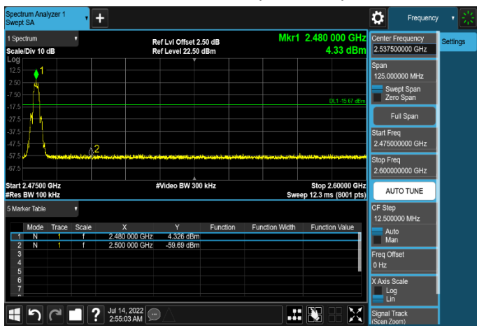
Mode 2 CH39 (2480MHz)
