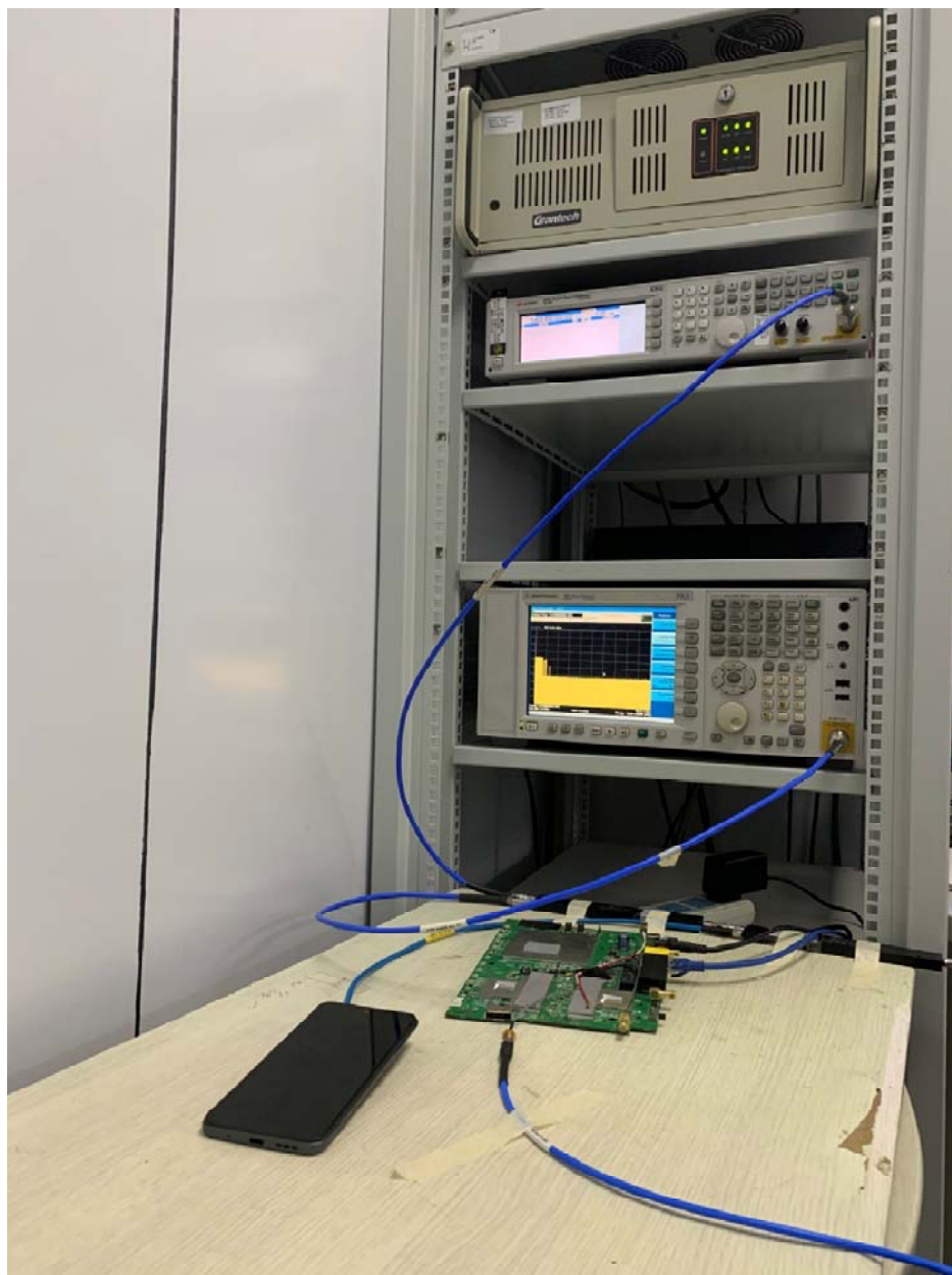
Picture 1 Test Setup
