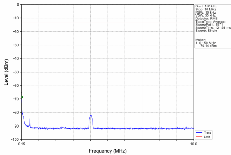
Band66_3MHz_16QAM_LCH_1711.5MHz_RB_1_0_NTNV
