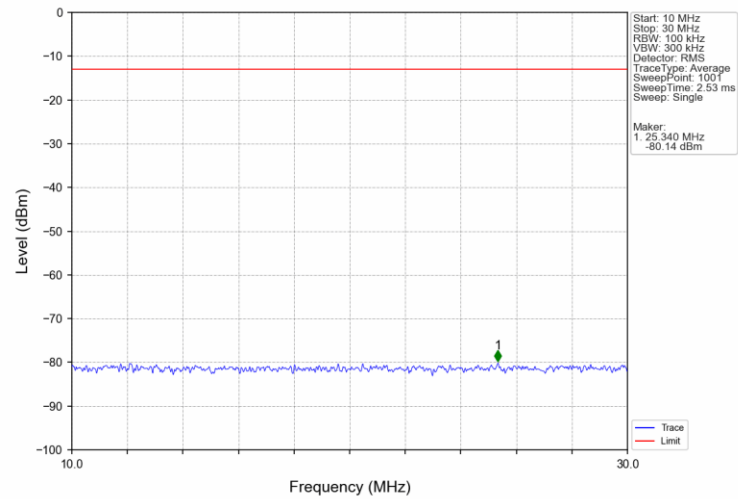
Band66_3MHz_16QAM_MCH_1745MHz_RB_1_0_NTNV
