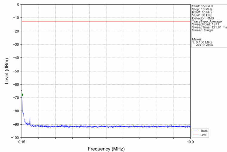
Band66_3MHz_QPSK_HCH_1778.5MHz_RB_1_0_NTNV
