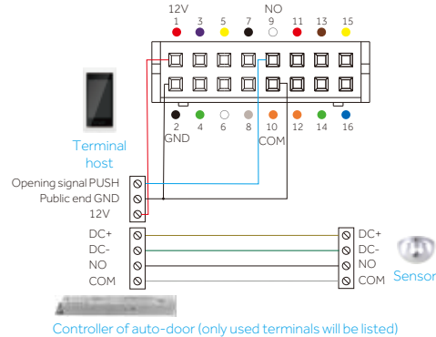
Wiring schematic drawing for sensor switch of automatic door
