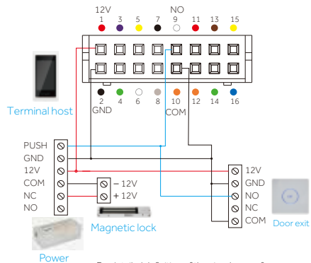
Wiring schematic drawing for touching switch of magnetic door
