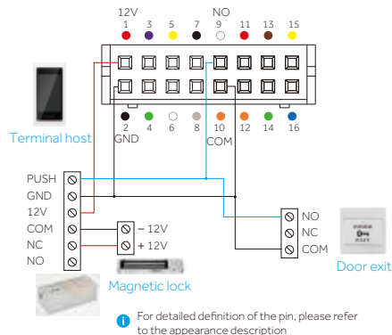
Wiring schematic drawing for mechanical switch of magnetic door
