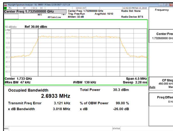
LTE B4 3MHz QPSK Middle Channel RB15-0
