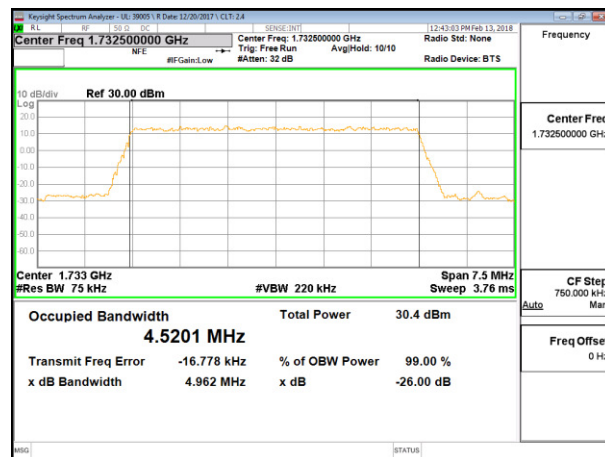
LTE B4 5MHz QPSK Middle Channel RB25-0
