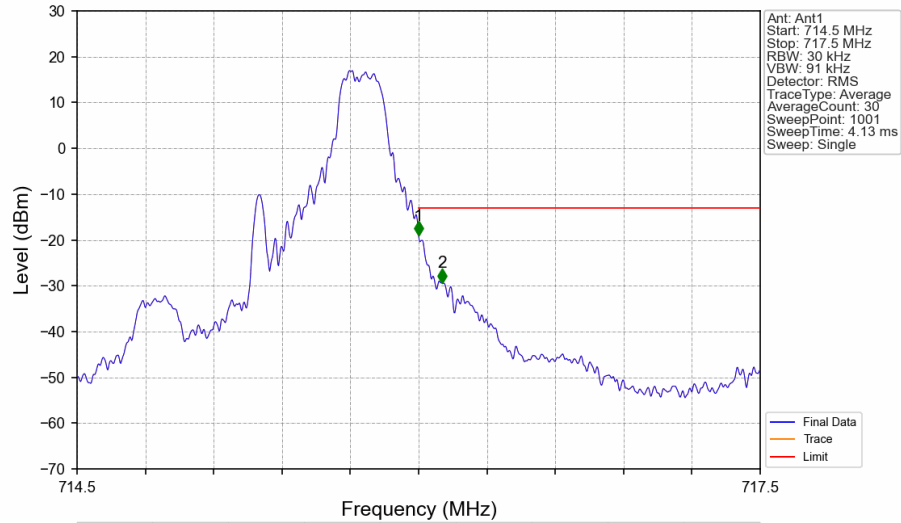
Band12 1.4MHz 16QAM HCH 715.3MHz RB_1_5 NTN
