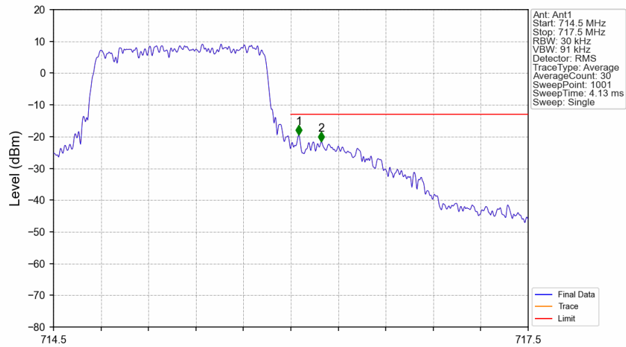
Band12 1.4MHz 16QAM HCH 715.3MHz RB_6_0 NTN
