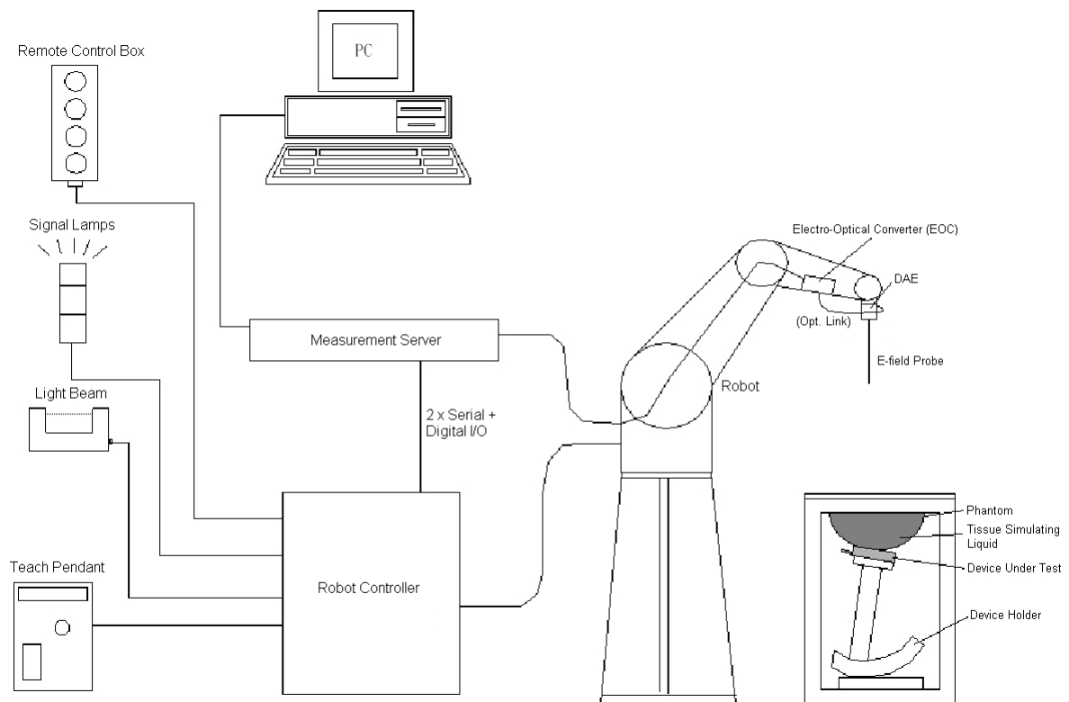
Fig-3.1 SPEAG DASY52 System Setup
