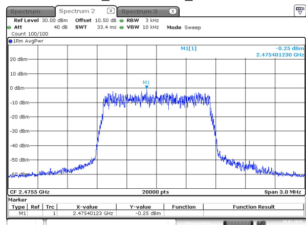
1.4M_2475.5 MHz_Chain 1
