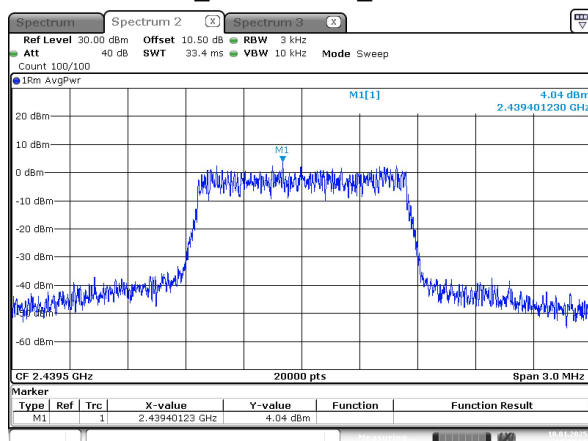
1.4M_2439.5 MHz_Chain 1
