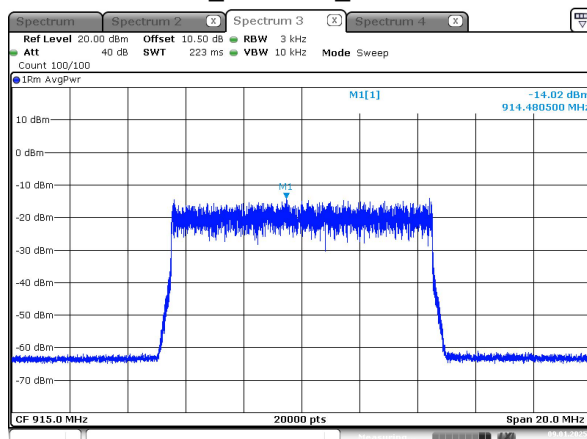
10M_915 MHz_Chain 0
