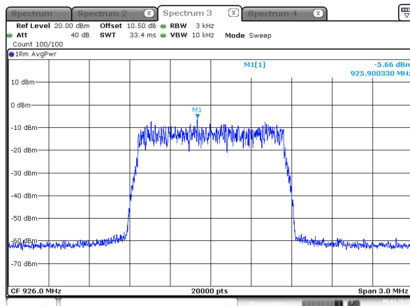
1.4M_926 MHz_Chain 0
