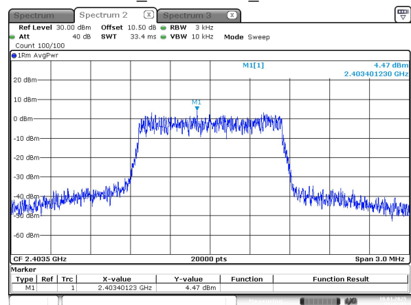
1.4M_2403.5 MHz_Chain 1
