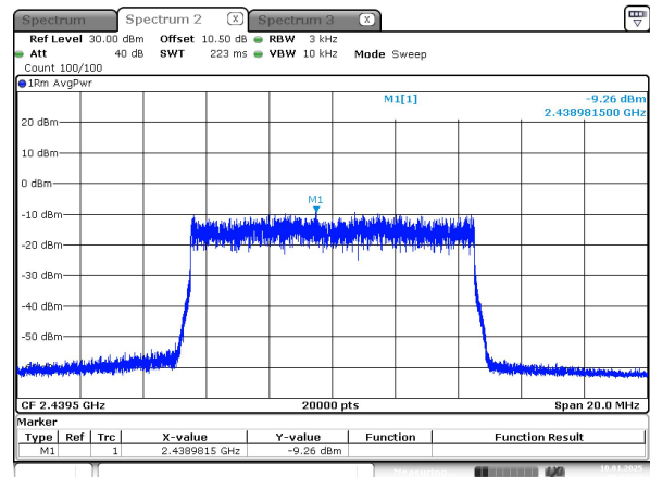
10M_2439.5 MHz_Chain 1
