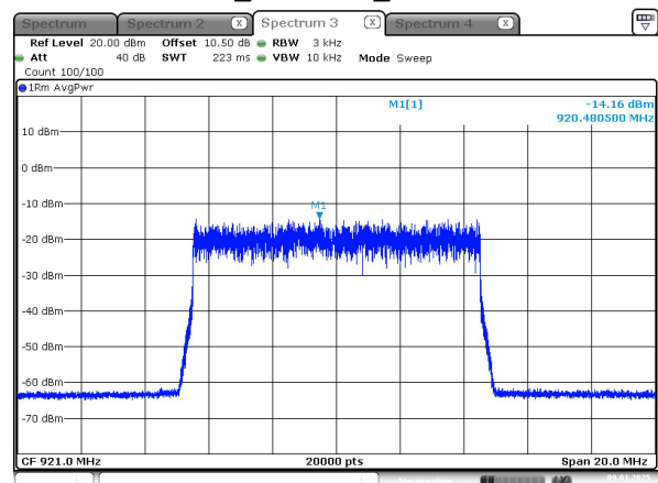
10M_921 MHz_Chain 0
