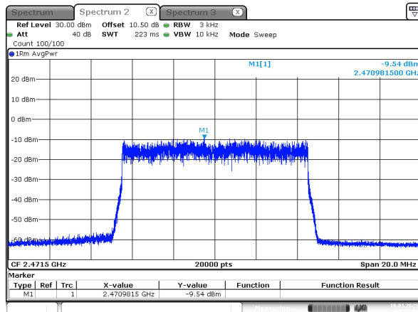
10M_2471.5 MHz_Chain 1
