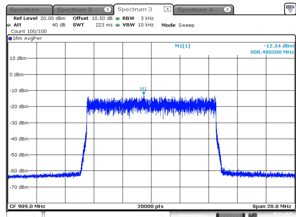
10M_909 MHz_Chain 0
