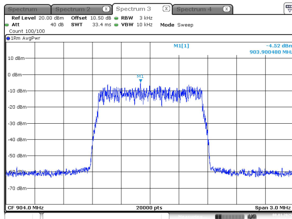
1.4M_904 MHz_Chain 0
