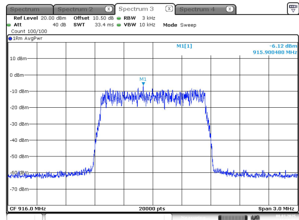
1.4M_916 MHz_Chain 0
