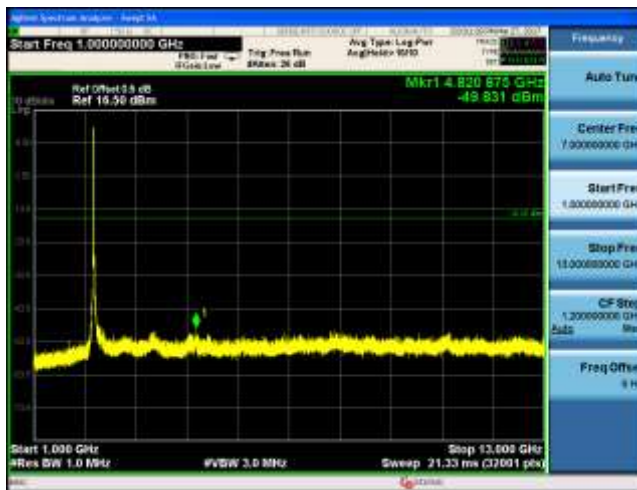
802.11g CH06 (2437MHz) -Ant 2
