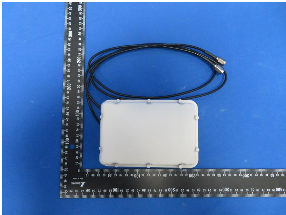
(12) EUT Photo (Directional Antenna)
