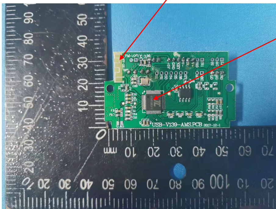
PCB Antenna
