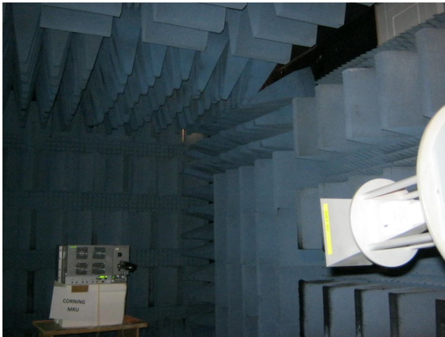
Figure 8. Radiated Emission Test 18-20.0GHz
