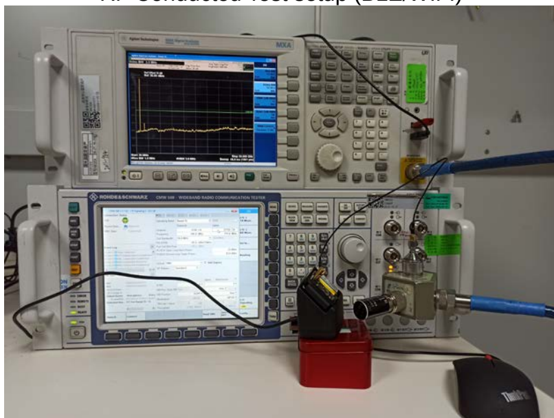
RF Conducted Test setup (LTE_CAT-M1)
