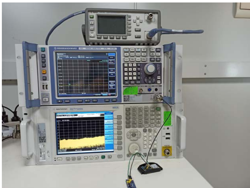
RF Conducted Test setup (BLE/WIFI)
