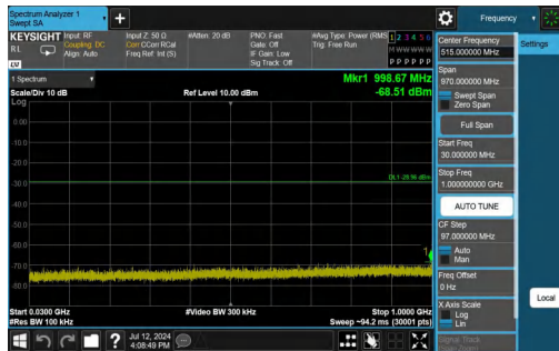
11AX40ISO-Ant1-2422-30~1000-PASS
