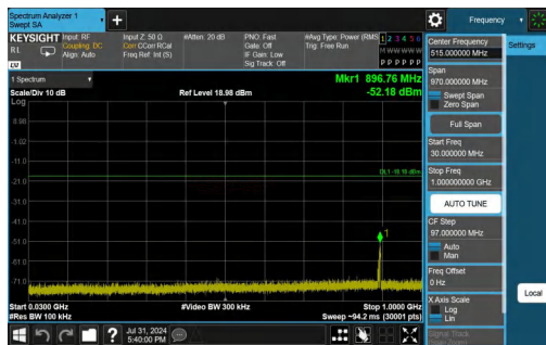
11AX20SISO-Ant1-2437-106Tone-RU53-30~1000-PASS
