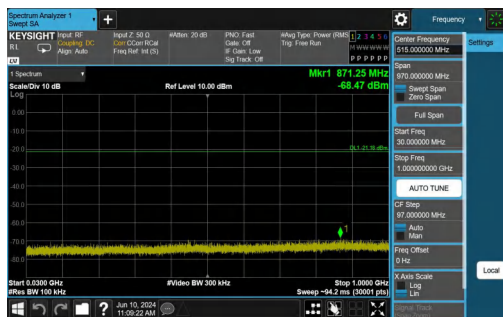
11B-Ant1-2462-30~1000-PASS
