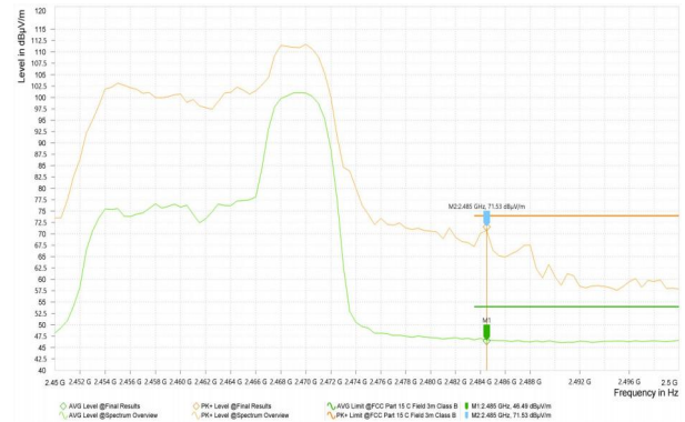
Wi-Fi 2.4G_11AX40_2452_242Tone_RU62
