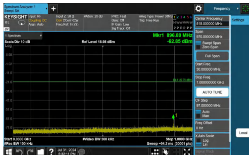
11AX20ISO-Ant1-2412-106Tone-RU53-30~1000-PASS
