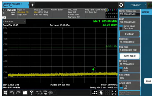
11N40SISO-Ant1-2422-30~1000-PASS
