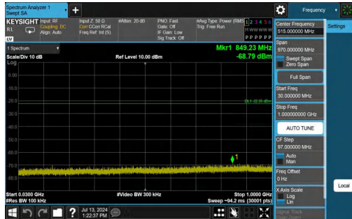
11B-Ant1-2437-30~1000-PASS
