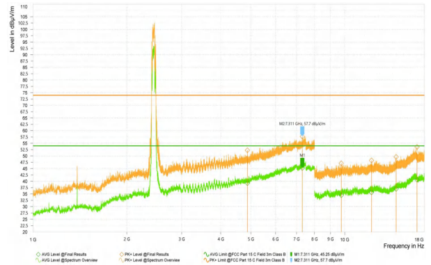
Wi-Fi 2.4G-11AX20_2412_High
