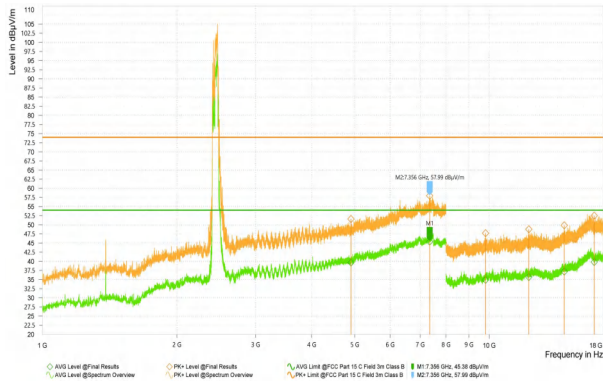
Wi-Fi 2.4G-11AX20_2437_High
