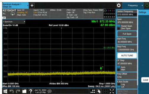
11N40SISO-Ant1-2452-30~1000-PASS
