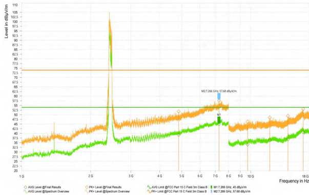
Wi-Fi 2.4G-11N40_2452_High
