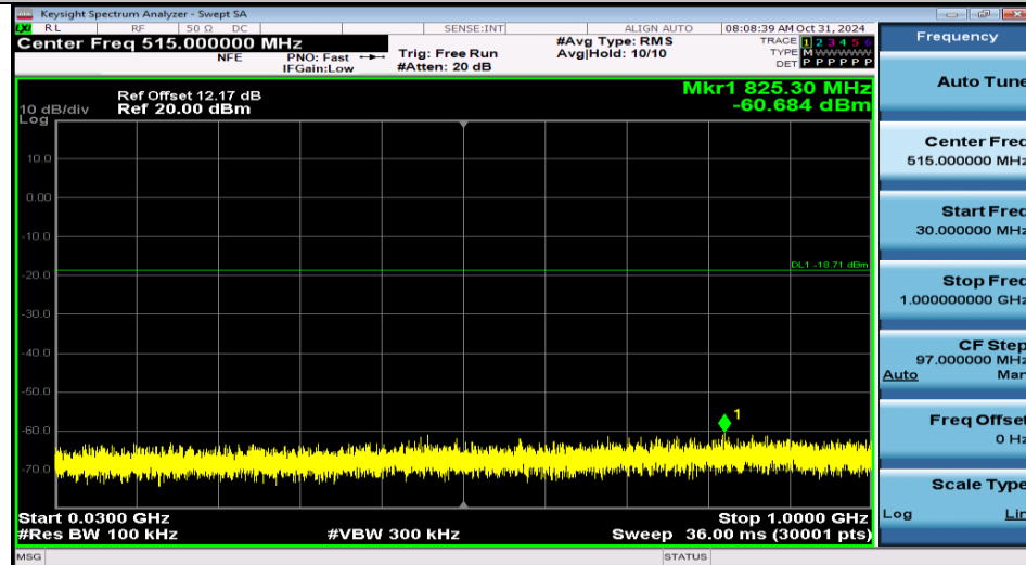
BLE_1M-Ant1-2480-30~1000-PASS
