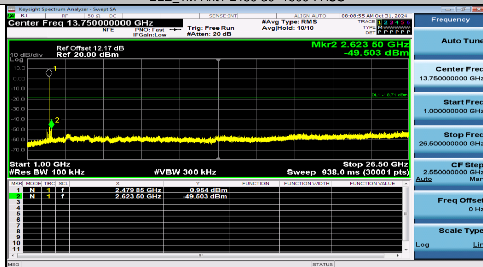
BLE_1M-Ant1-2480-1000~26500-PASS
