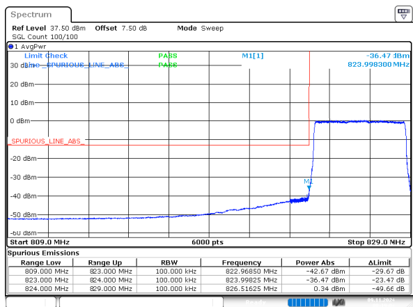
2_5MHz_Low_16QAM_25@0
