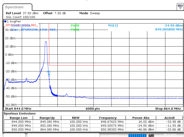
2_5MHz_High_QPSK_1@24
