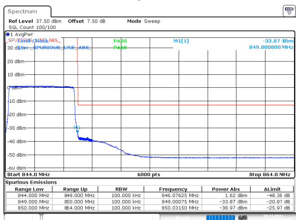
2_5MHz_High_QPSK_25@0
