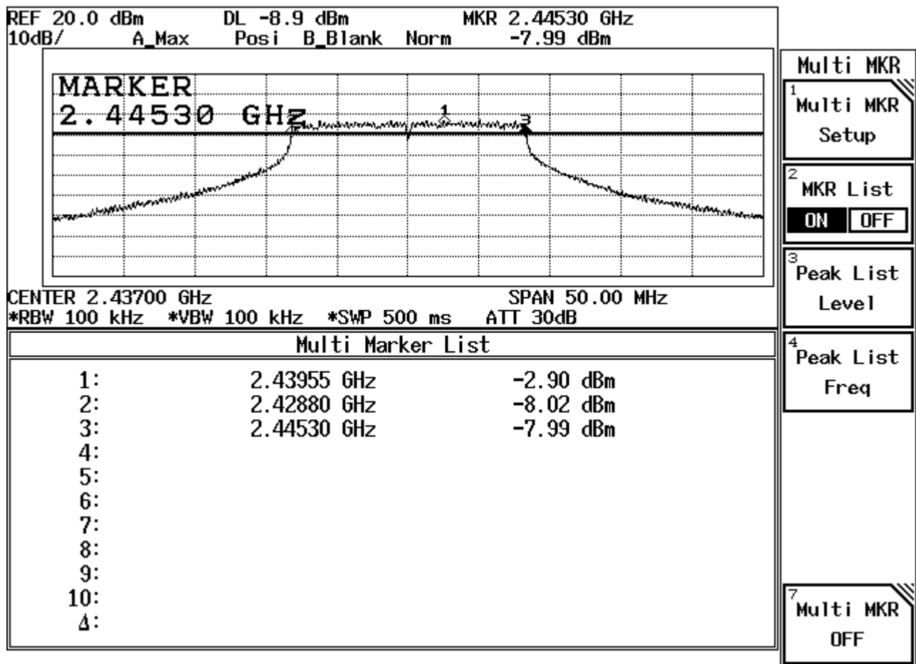
Figure Channel 6: 54Mbps
