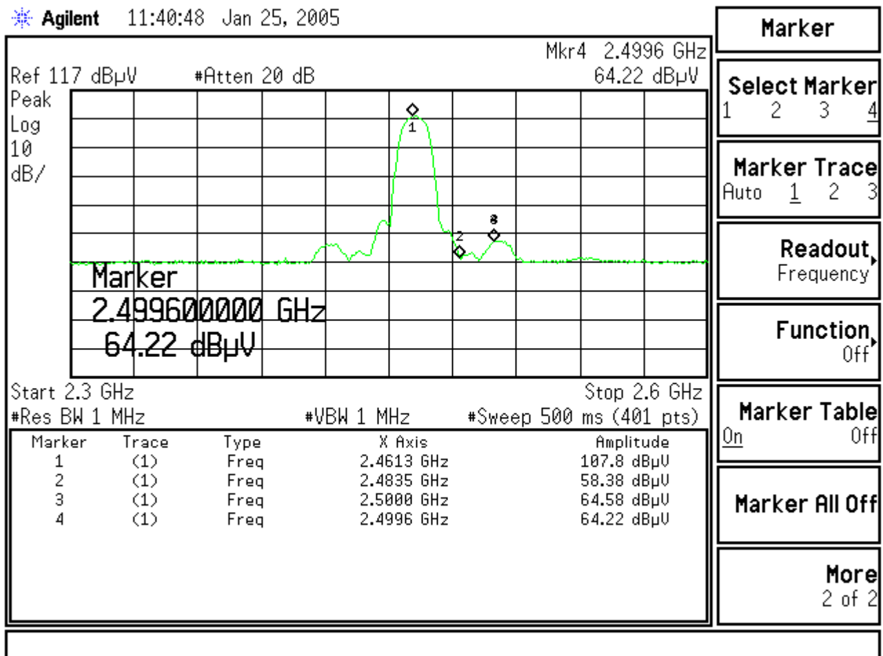
Figure Channel 11: (Vertical)
