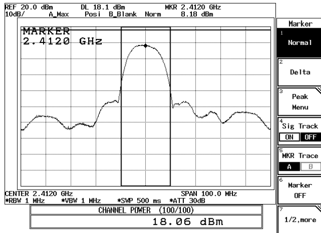
11Mbps-Ch01
