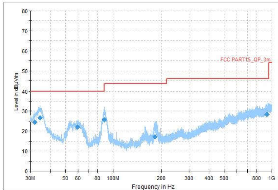
Fig. 39 Radiated Spurious Emission (All Channels, 30MHz ~1GHz)
