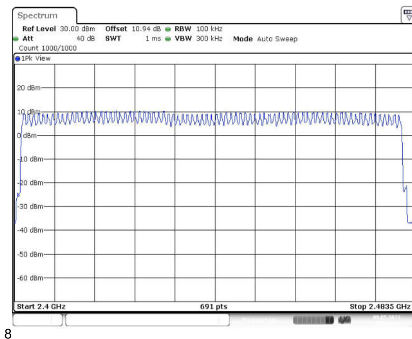
Fig. 57 Number of Hopping Channels ( \pi/4 DQPSK, Hopping)
