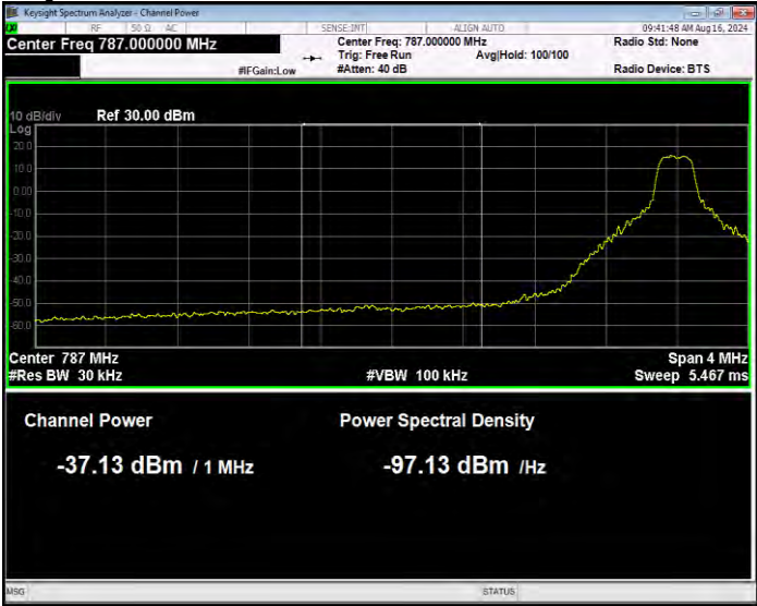
Band14 16QAM BW=10MHz Channel=23330 RB Size=1 Position=#0 Normal
