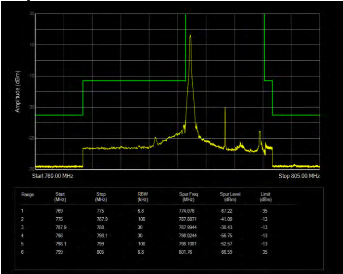
Band14 16QAM BW=10MHz Channel=23330 RB Size=1 Position=#Max Extended
