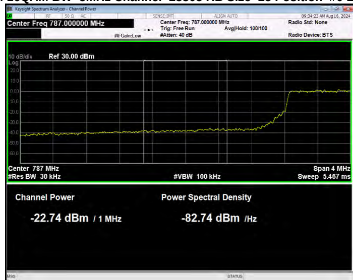
Band14 16QAM BW=5MHz Channel=23305 RB Size=25 Position=#0 Normal
