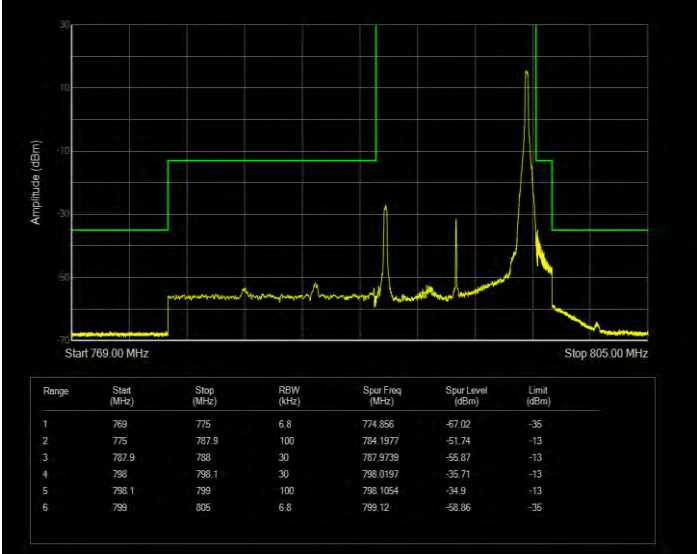
Band14 16QAM BW=10MHz Channel=23330 RB Size=50 Position=#0 Extended
