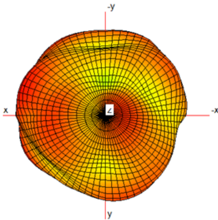
Antenna 2440MHz 3D Pattern
