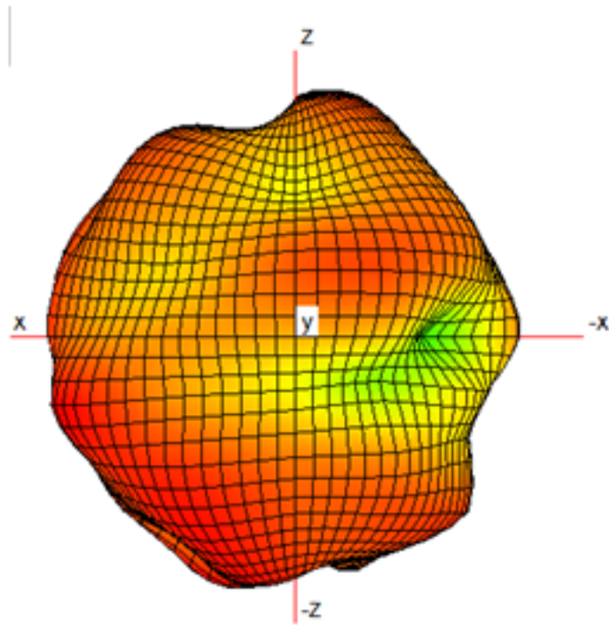
Antenna 2440MHz 3D Pattern
