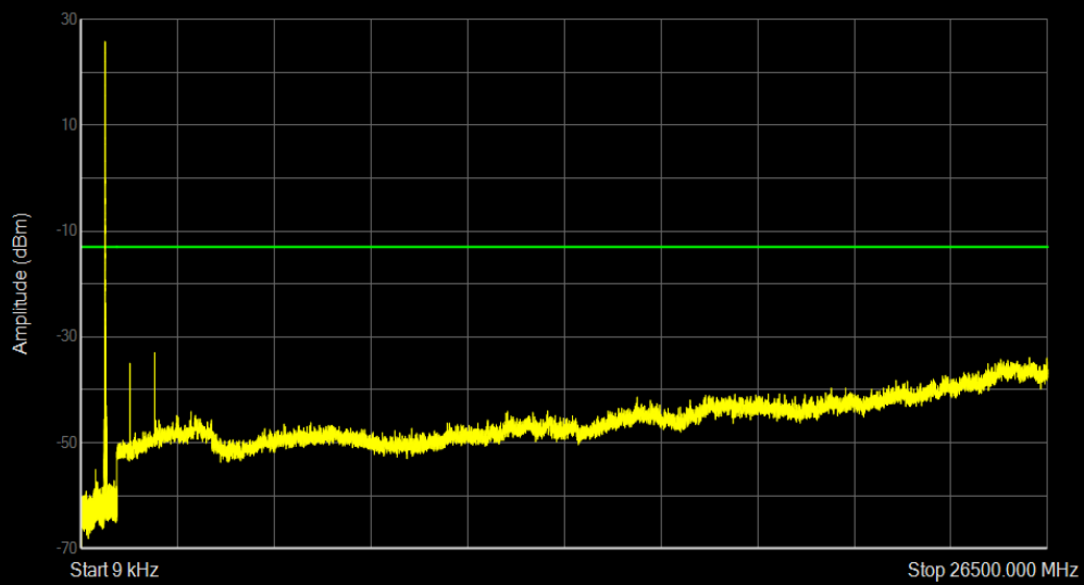
Band71 QAM16 BW=20MHz Channel=133372 RB Size=1 Position=#0
