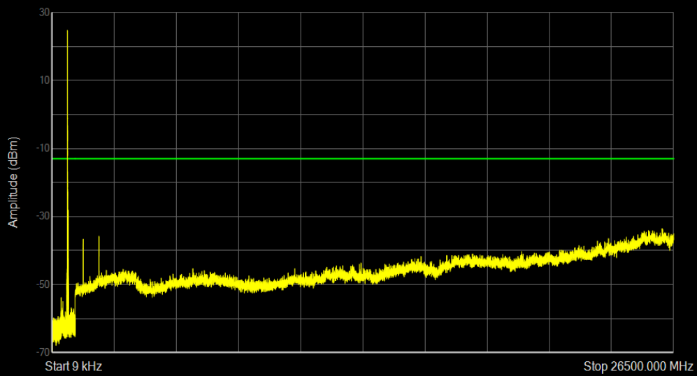
Band71 QAM16 BW=20MHz Channel=133297 RB Size=1 Position=#0
