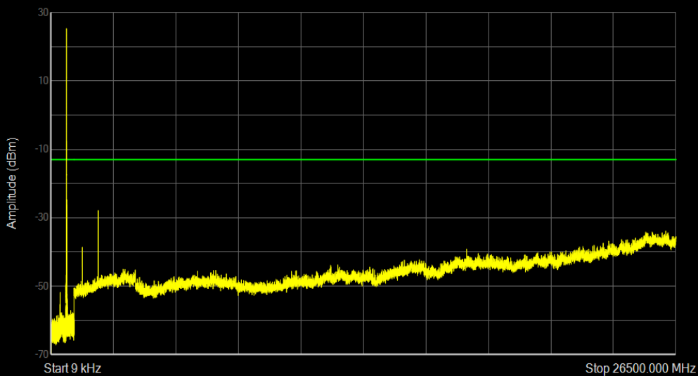
Band71 QPSK BW=15MHz Channel=133297 RB Size=1 Position=#0
