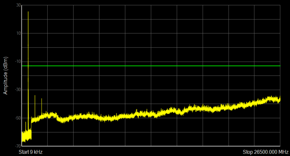
Band71 QAM16 BW=10MHz Channel=133422 RB Size=1 Position=#0
