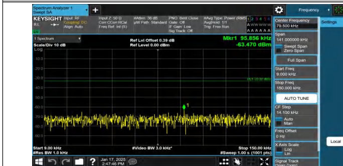
Band5-4233-3-0.009~0.15MHz-PASS
