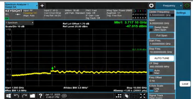
Band5-4233-2-1000~10000MHz-PASS
