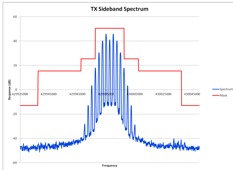
E1-5.13 Occupied Bandwidth, Analog, 25 kHz Channels, 429.9875 MHz
