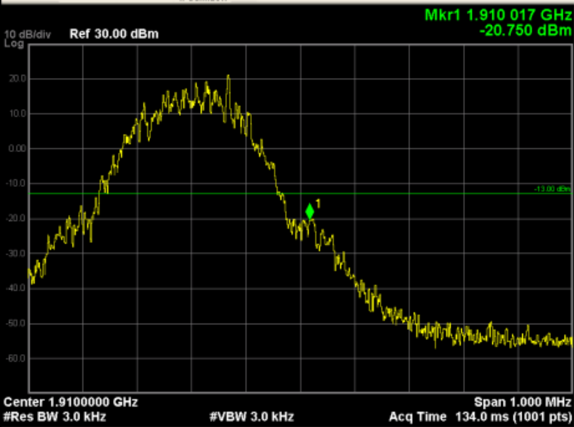
GSM 1900 (GSM Link), Channel 810
