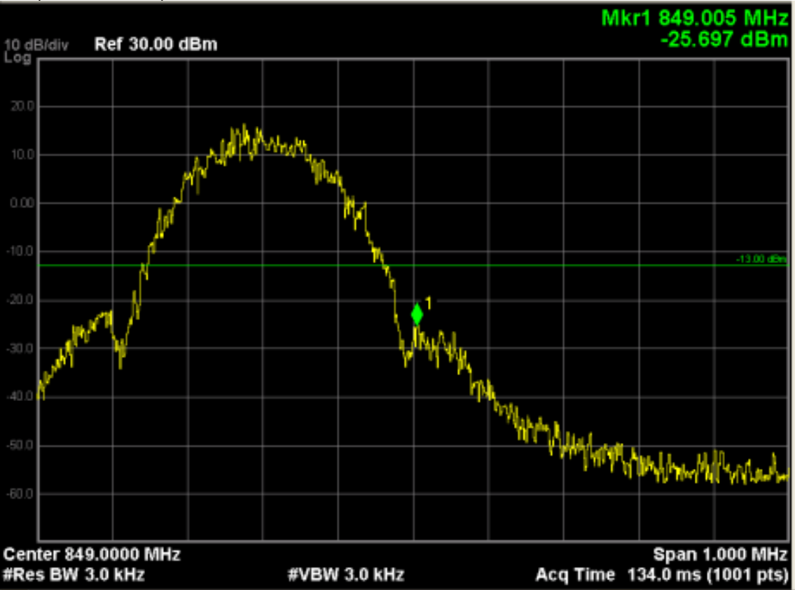
GSM850 (EDGE 8 Link), Channel 251
