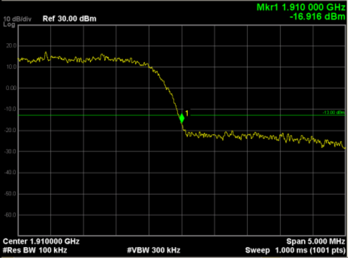
WCDMA Band II, Channel 9538
