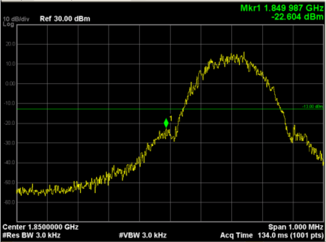
GSM1900 (EDGE 8 Link), Channel 512
