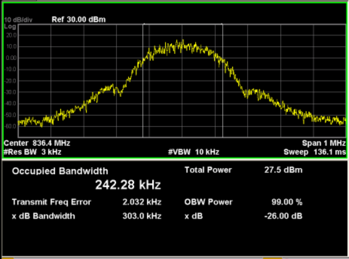
GSM850 (EDGE 8 Link), Channel 189
