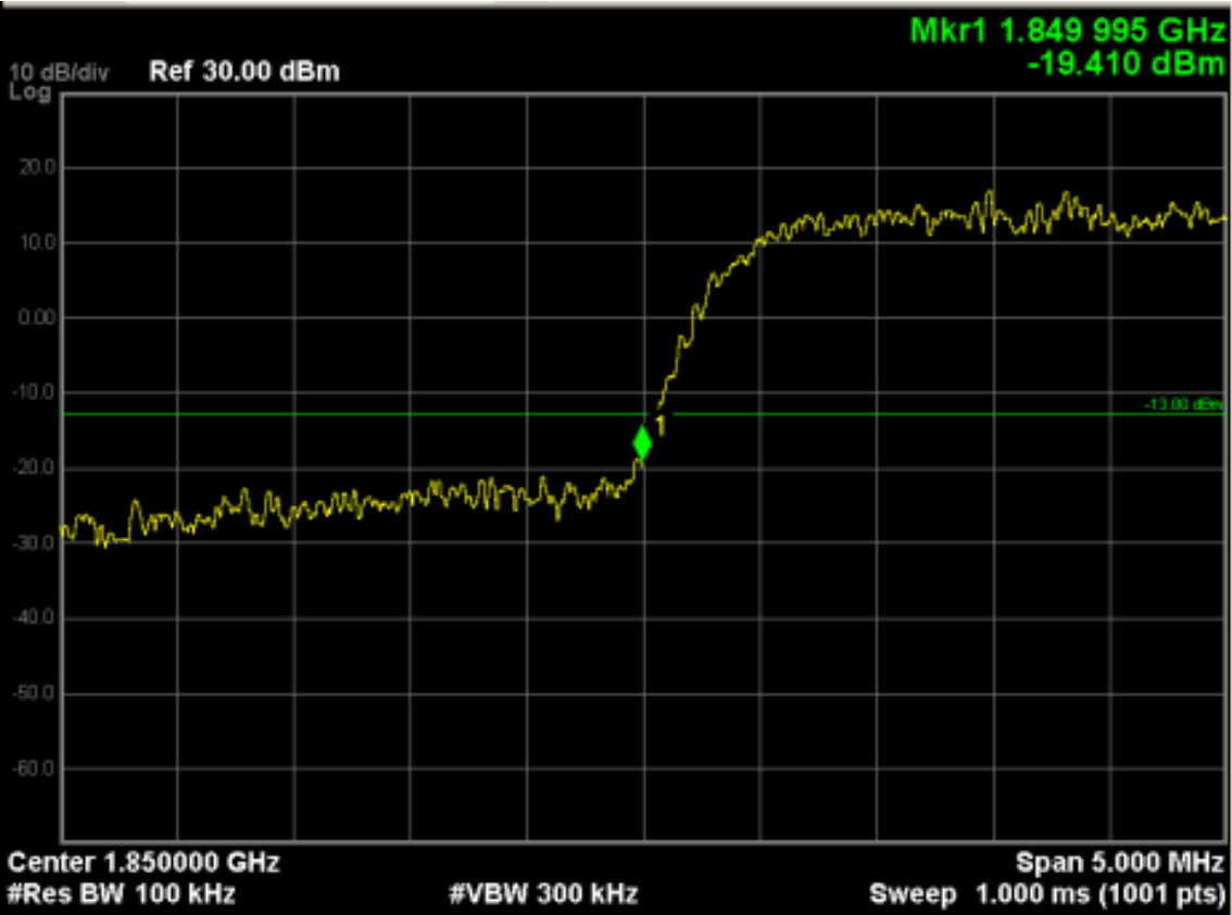
WCDMA Band II, Channel 9262
