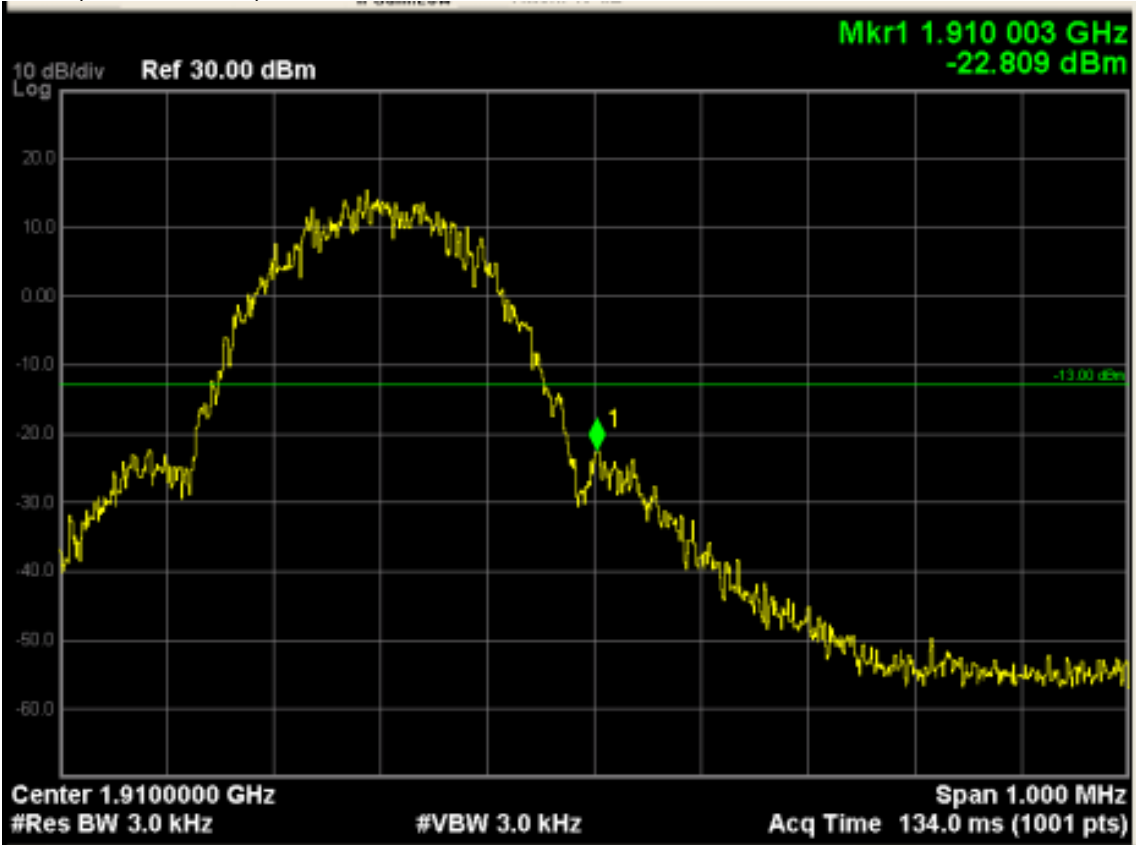
GSM1900 (EDGE 8 Link), Channel 810
