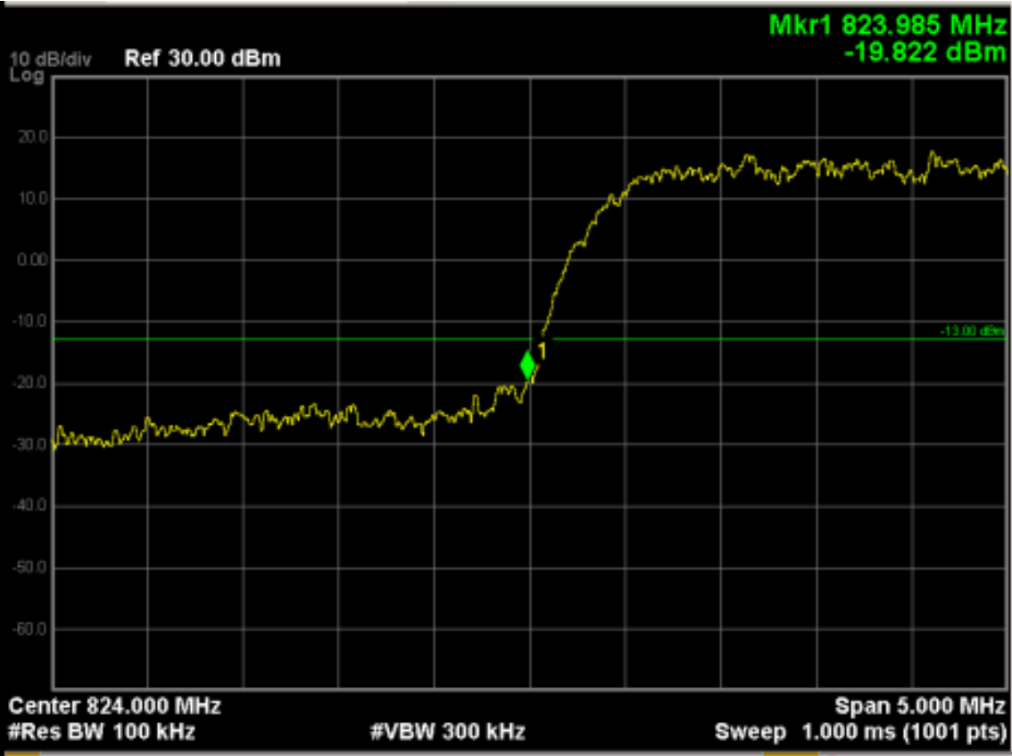
WCDMA Band V, Channel 4132
