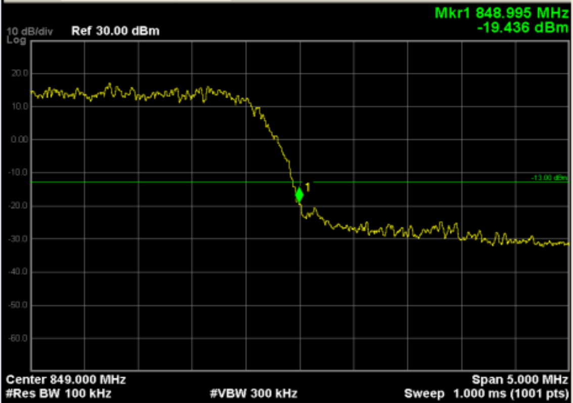
WCDMA Band V, Channel 4233
