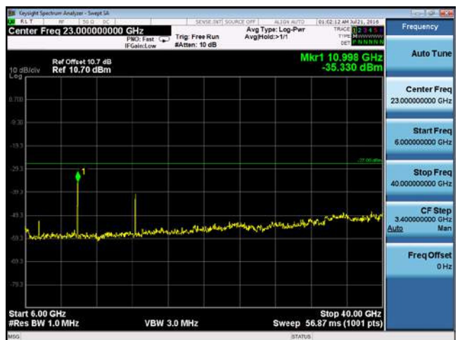
CUE-802.11a-5500M-chain3(6GHz-40GHz)
