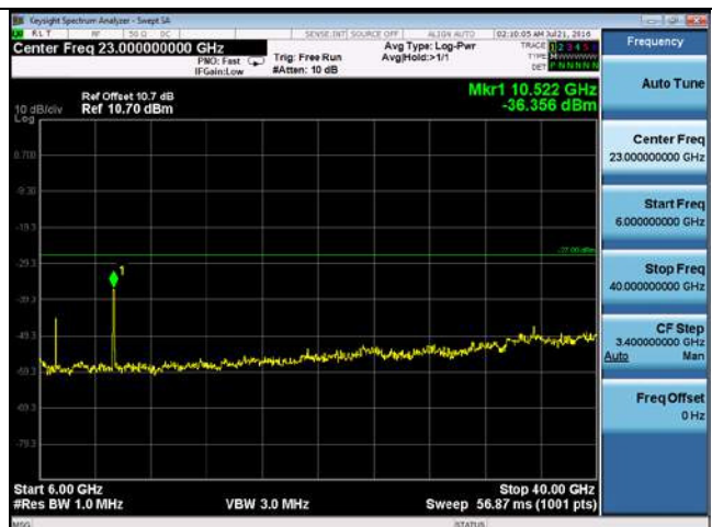
CUE-802.11n-40-5270M-chain4(6GHz-40GHz)
