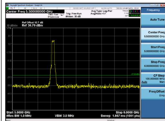
CUE-802.11n-20-5320M-chain 4(5GHz-6GHz)
