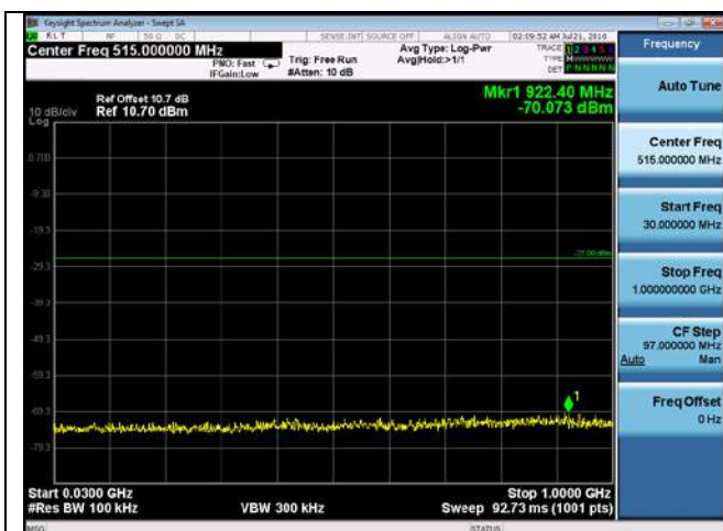
CUE-802.11n-40-5270M-chain4(30MHz-1GHz)
