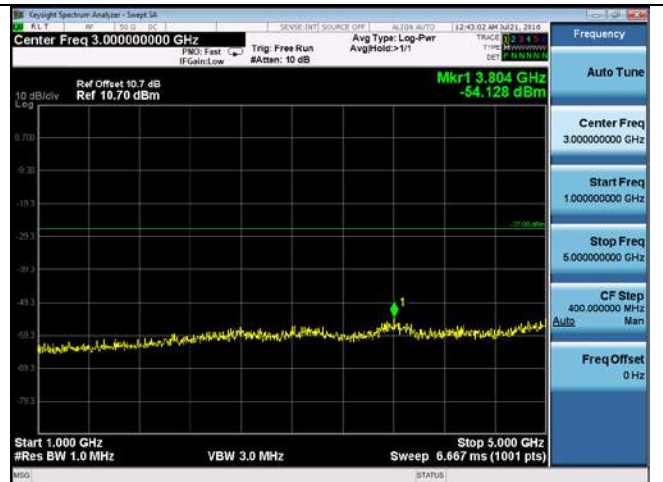
CUE-802.11ac-80-5290M-chain 2(1GHz-5GHz)
