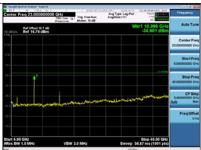
CUE-802.11a-5500M-chain4(6GHz-40GHz)
