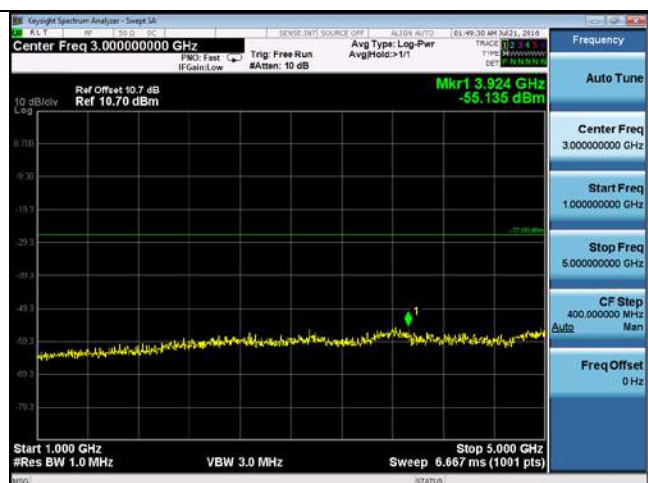
CUE-802.11n-20-5500M-chain4(1GHz-5GHz)
