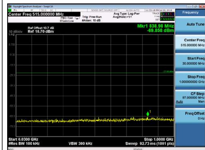
CUE-802.11a-5580M-chain1(30MHz-1GHz)
