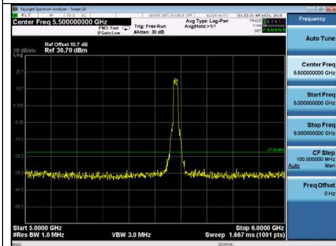
CUE-802.11a-5580M -chain3(5GHz-6GHz)
