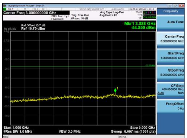
CUE-802.11a-5580M -chain4(1GHz-5GHz)
