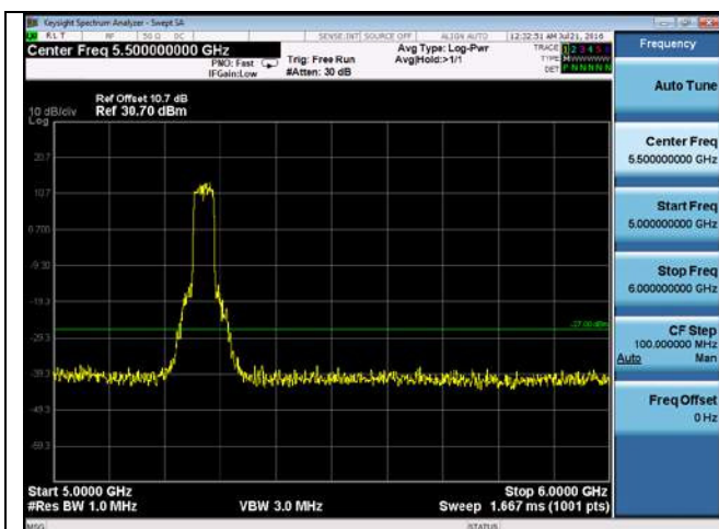
CUE-802.11n-40-5270M-chain2(5GHz-6GHz)
