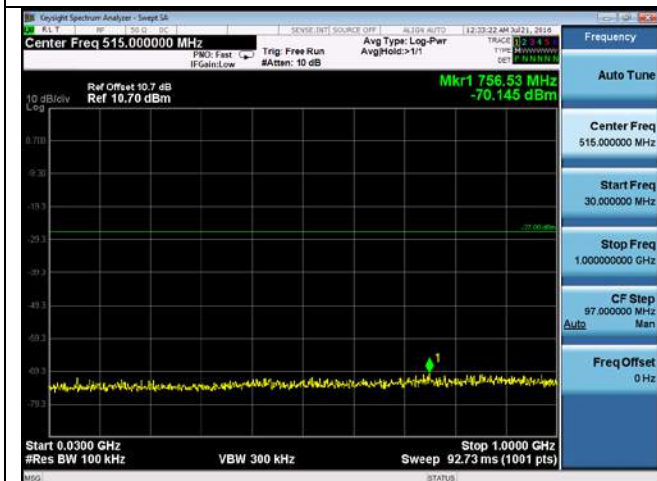
CUE-802.11n-40-5310M -chain2(30MHz-1GHz)
