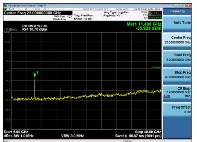
CUE-802.11a-5700M-chain 4(6GHz-40GHz)
