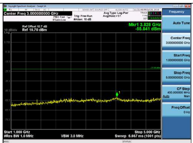
CUE-802.11a-5500M-chain1(1GHz-5GHz)
