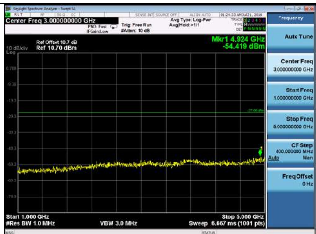
CUE-802.11n-40-5270M-chain3(1GHz-5GHz)
