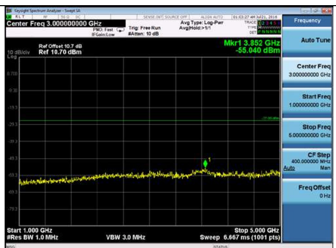
CUE-802.11a-5580M -chain3(1GHz-5GHz)
