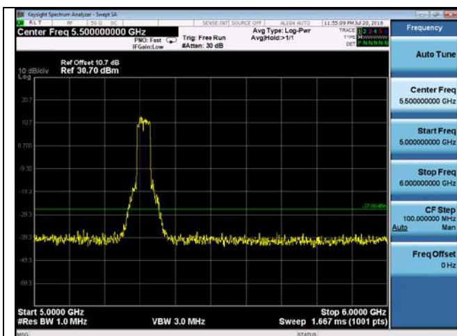
CUE-802.11n-40-5310M -chain1(5GHz-6GHz)
