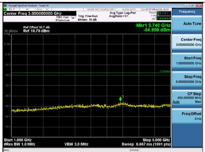
CUE-802.11n-20-5700M-chain 1(1GHz-5GHz)
