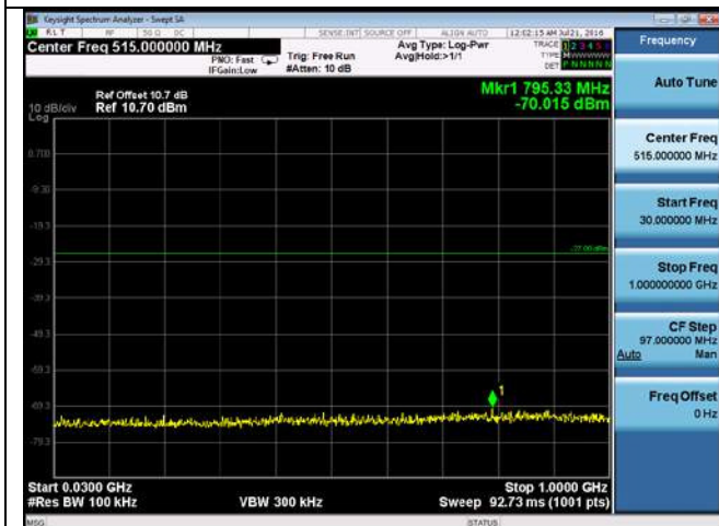
CUE-802.11ac-80-5290M-chain 1(30MHz-1GHz)
