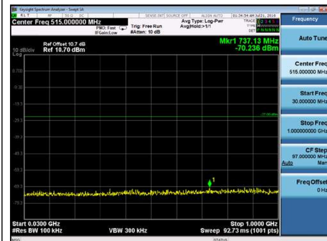
CUE-802.11ac-80-5290M-chain 3(30MHz-1GHz)
