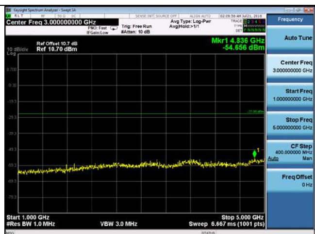
CUE-802.11n-40-5270M-chain4(1GHz-5GHz)
