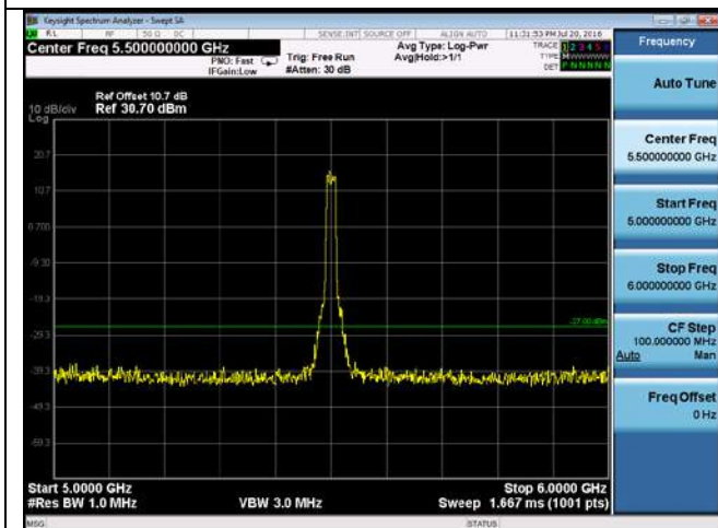
CUE-802.11a-5500M-chain1(5GHz-6GHz)
