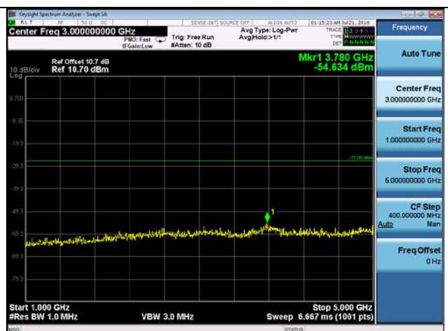
CUE-802.11n-20-5580M-chain3(1GHz-5GHz)
