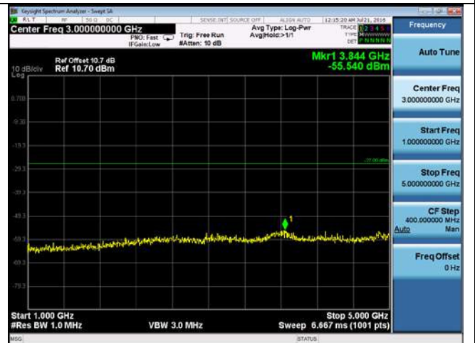
CUE-802.11a-5580M--chain2(1GHz-5GHz)
