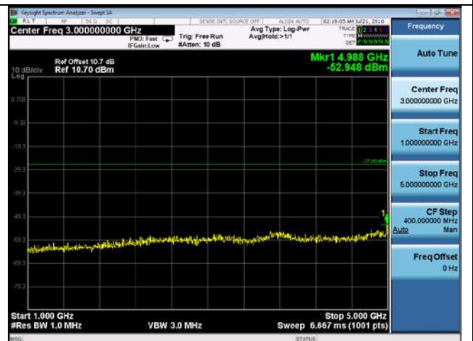
CUE-802.11ac-80-5290M-chain 4(1GHz-5GHz)
