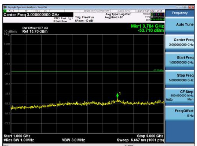
CUE-802.11n-20-5500M-chain2(1GHz-5GHz)
