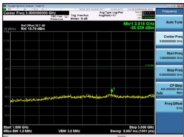
CUE-802.11n-20-5580M-chain1(1GHz-5GHz)
