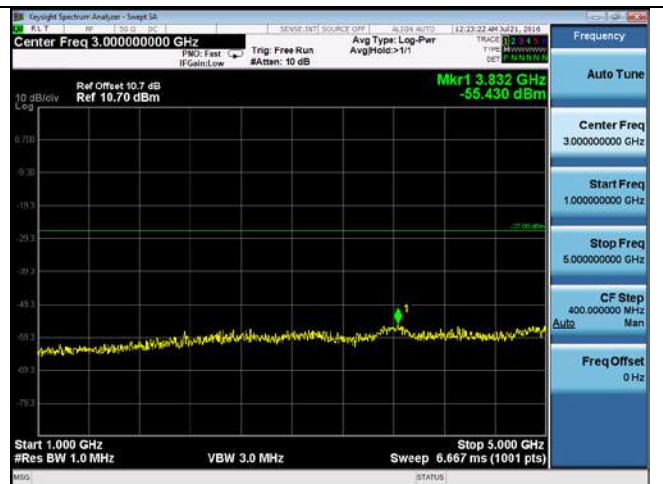
CUE-802.11n-20-5320M-chain 2(1GHz-5GHz)
