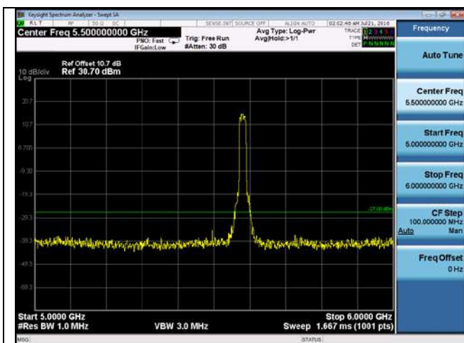
CUE-802.11n-20-5580M-chain 4(5GHz-6GHz)
