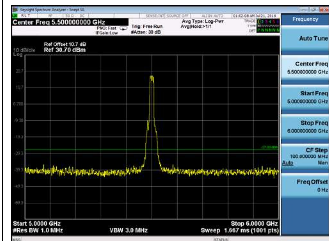
CUE-802.11n-20-5500M-chain3(5GHz-6GHz)
