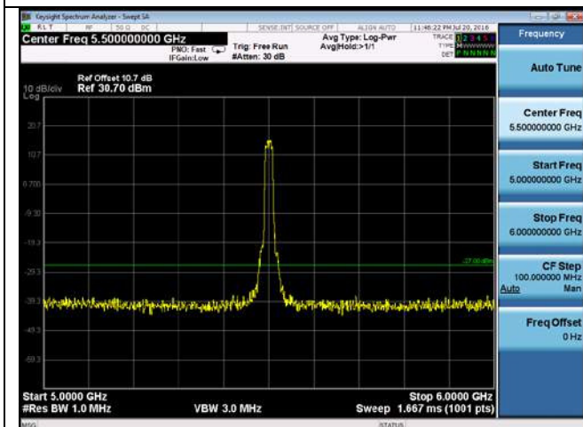
CUE-802.11n-20-5500M-chain1(5GHz-6GHz)
