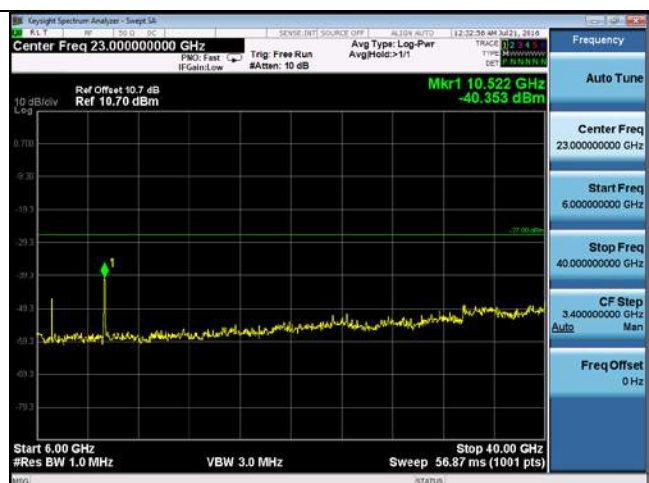
CUE-802.11n-40-5270M-chain2(6GHz-40GHz)
