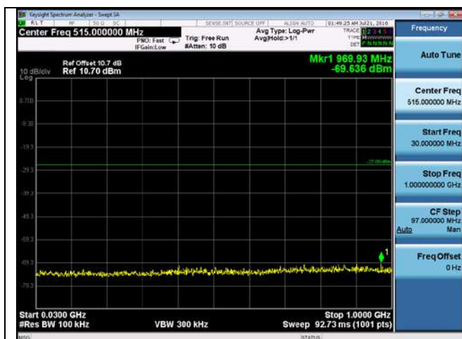
CUE-802.11n-20-5500M-chain4(30MHz-1GHz)
