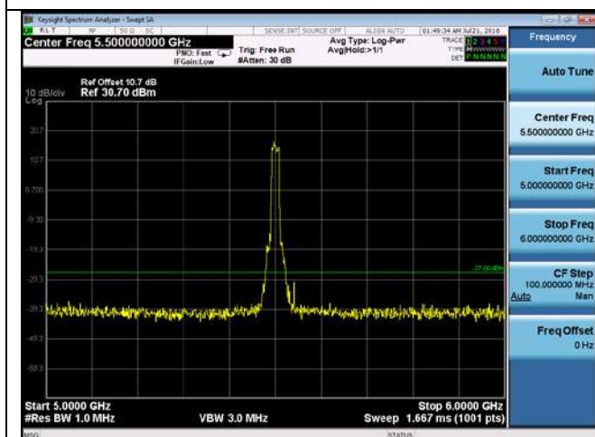
CUE-802.11a-5500M-chain4(5GHz-6GHz)
