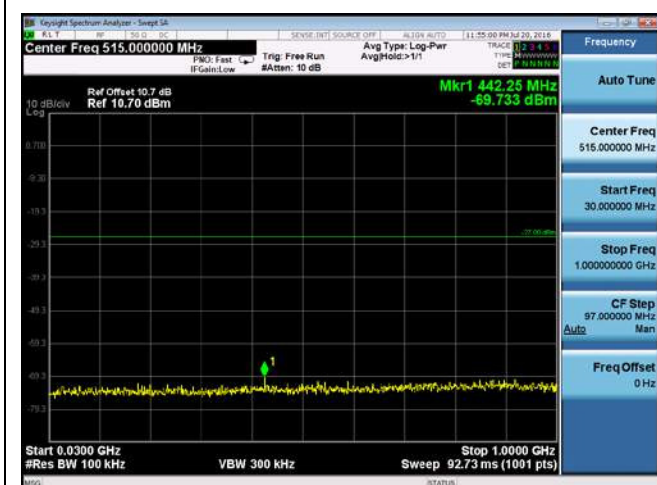
CUE-802.11n-40-5310M-chain1(30MHz-1GHz)
