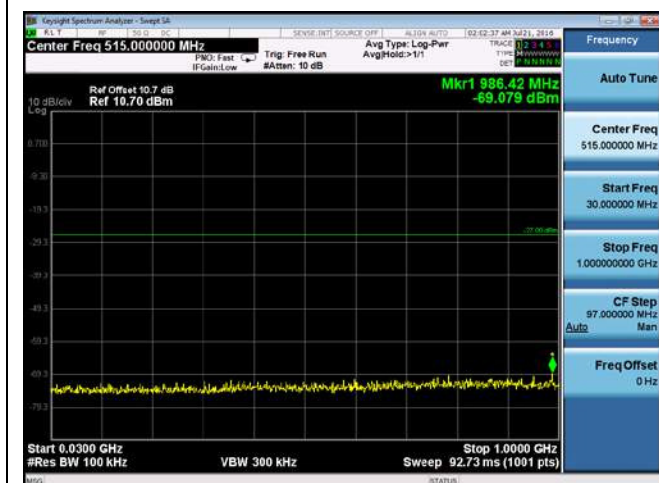
CUE-802.11n-20-5580M-chain4(30MHz-1GHz)
