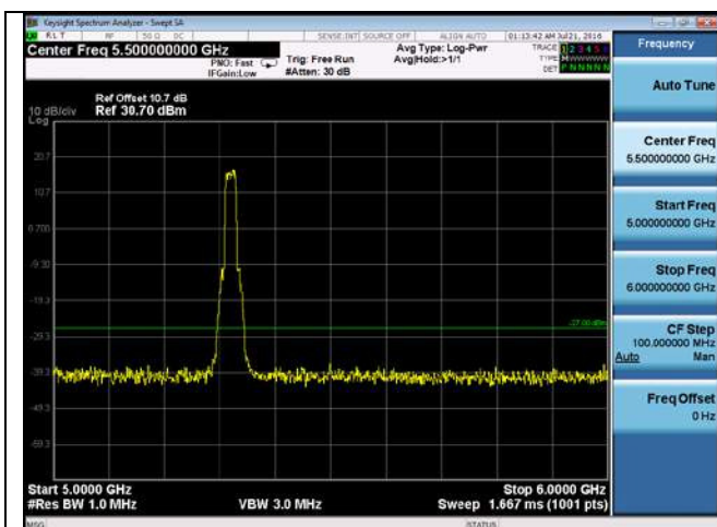
CUE-802.11n-20-5320M-chain 3(5GHz-6GHz)
