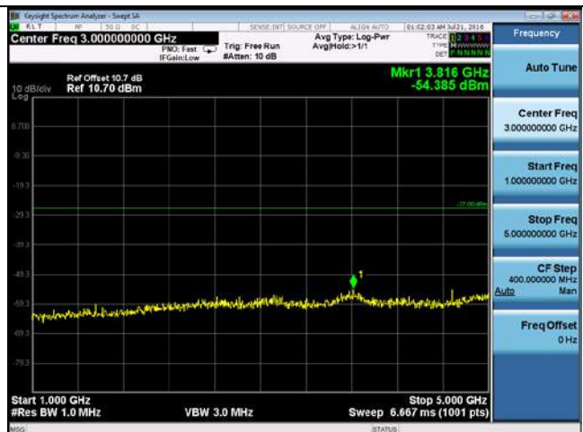
CUE-802.11n-20-5500M-chain3(1GHz-5GHz)
