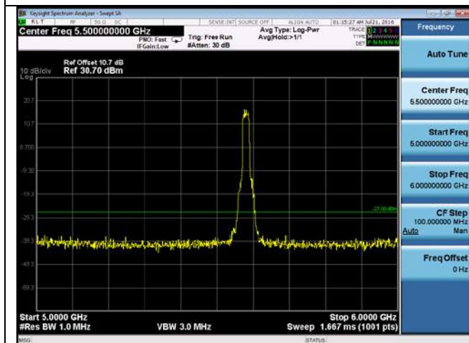
CUE-802.11n-20-5580M-chain3(5GHz-6GHz)
