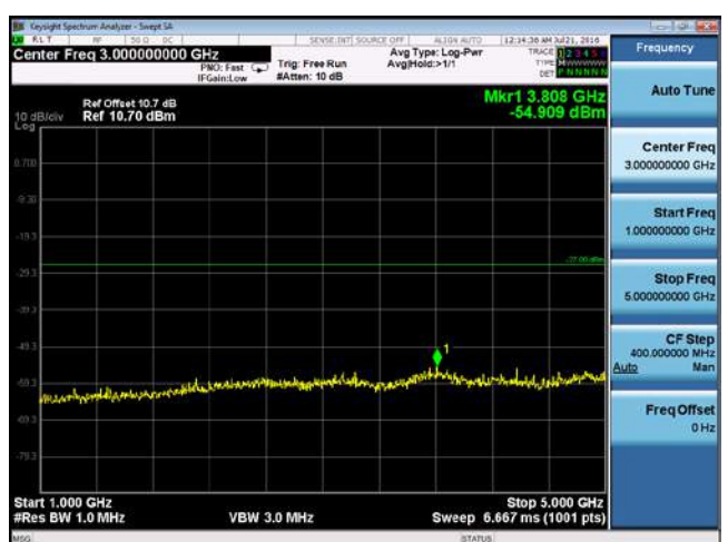
CUE-802.11a-5500M-chain2(1GHz-5GHz)
