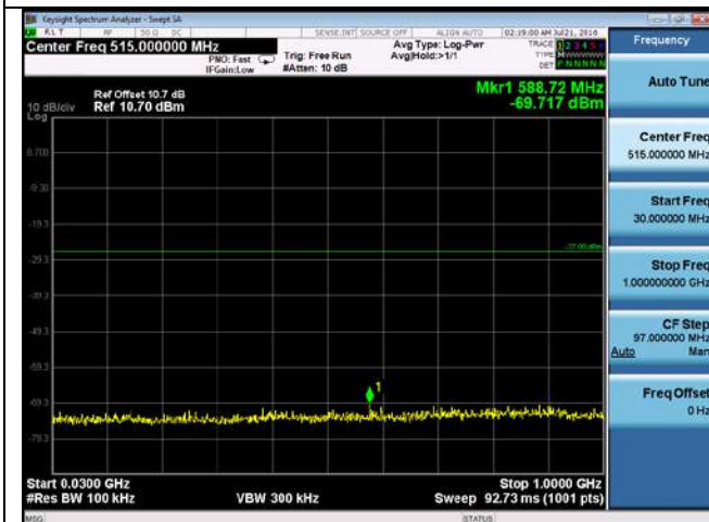
CUE-802.11ac-80-5290M-chain 4(30MHz-1GHz)
