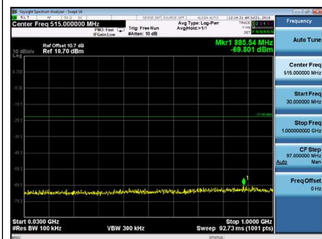
CUE-802.11a-5500M-chain2(30MHz-1GHz)
