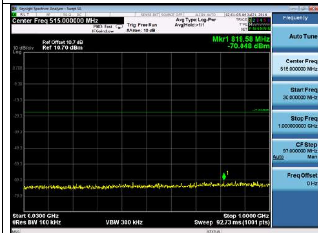
CUE-802.11n-20-5320M-chain 4(30MHz-1GHz)
