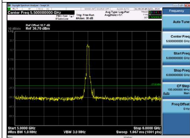
CUE-802.11n-20-5500M-chain4(5GHz-6GHz)
