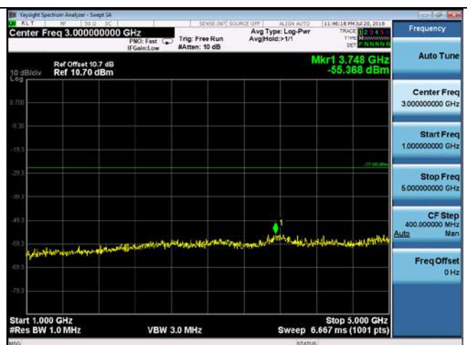
CUE-802.11n-20-5500M-chain1(1GHz-5GHz)
