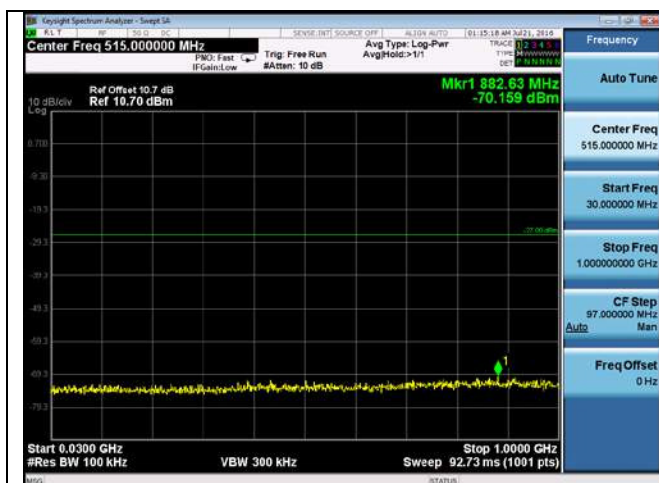
CUE-802.11n-20-5580M-chain3(30MHz-1GHz)
