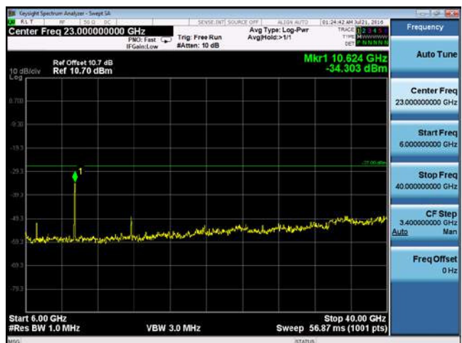
CUE-802.11n-40-5270M-chain3(6GHz-40GHz)
