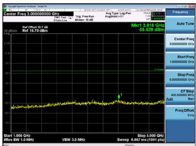
CUE-802.11a-5580M-chain1(1GHz-5GHz)
