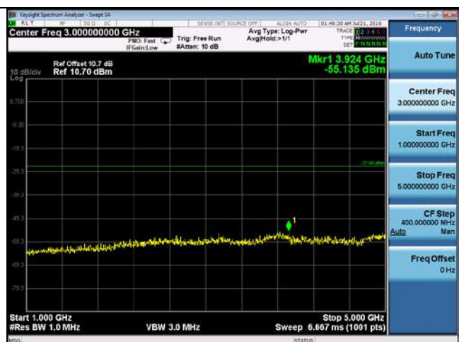
CUE-802.11a-5500M-chain4(1GHz-5GHz)
