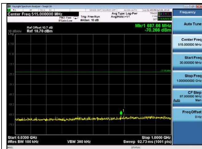
CUE-802.11a-5500M-chain1(30MHz-1GHz)
