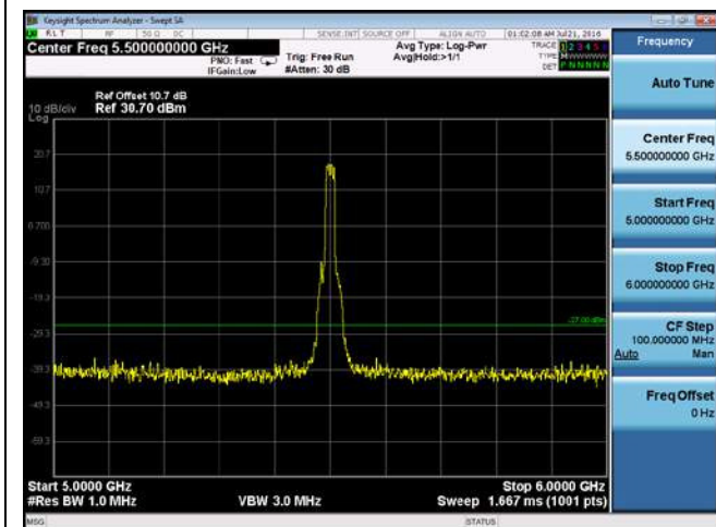
CUE-802.11a-5500M -chain3(5GHz-6GHz)
