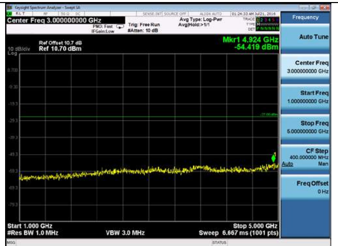
CUE-802.11n-40-5310M-chain3(1GHz-5GHz)
