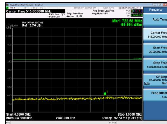
CUE-802.11n-20-5700M -chain 3(30MHz-1GHz)
