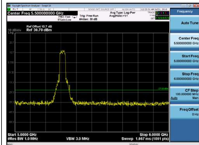
CUE-802.11n-40-5310M-chain2(5GHz-6GHz)
