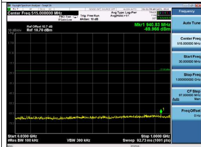
CUE-802.11n-20-5500M-chain3(30MHz-1GHz)
