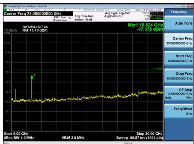
CUE-802.11n-40-5310M-chain 4(6GHz-40GHz)
