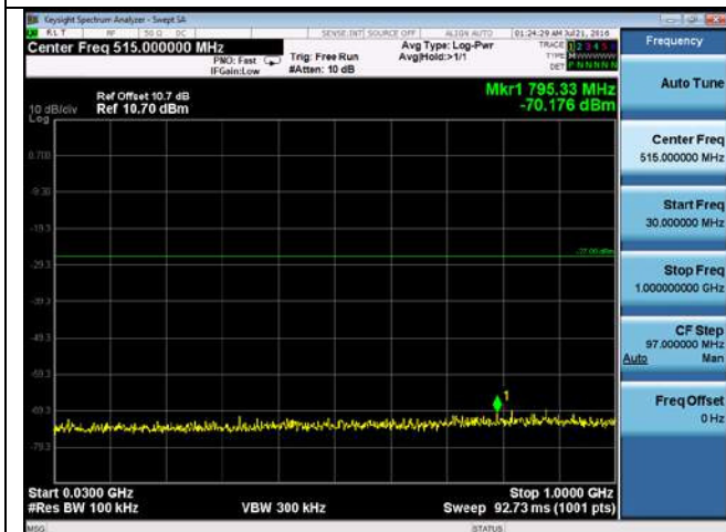
CUE-802.11n-40-5270M-chain3(30MHz-1GHz)
