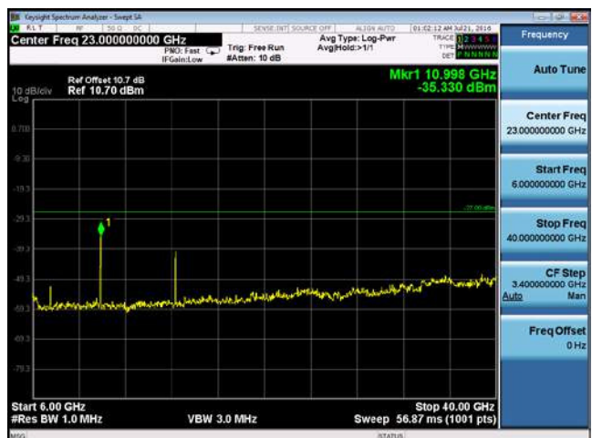
CUE-802.11n-20-5500M-chain3(6GHz-40GHz)
