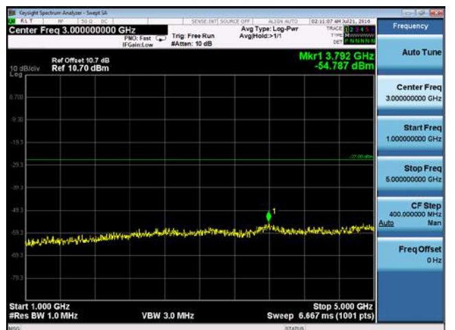
CUE-802.11n-40-5310M-chain4(1GHz-5GHz)
