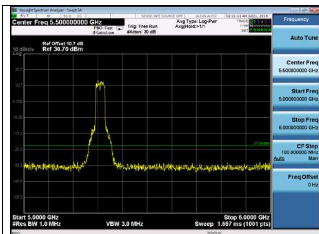
CUE-802.11n-40-5310M-chain 4(5GHz-6GHz)
