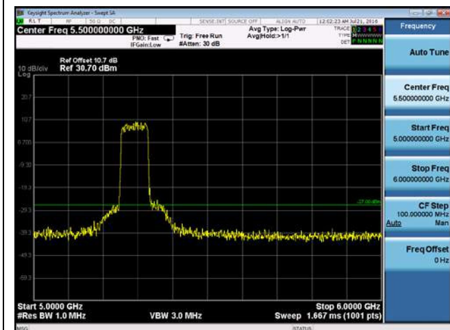
CUE-802.11ac-80-5290M-chain 1(5GHz-6GHz)
