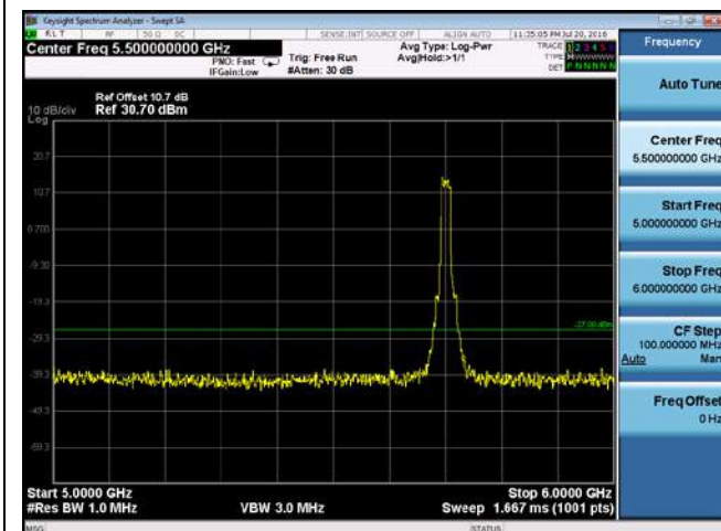
CUE-802.11a-5700M-chain 1(5GHz-6GHz)
