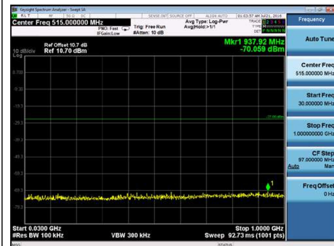
CUE-802.11a-5700M-chain 3(30MHz-1GHz)
