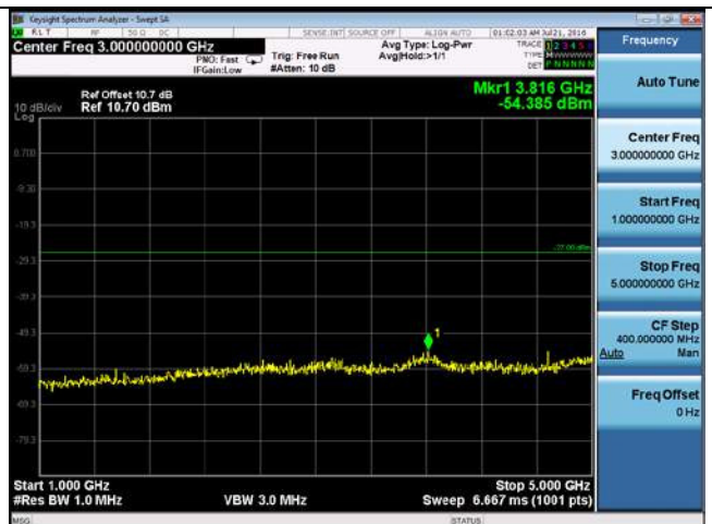
CUE-802.11a-5500M -chain3(1GHz-5GHz)
