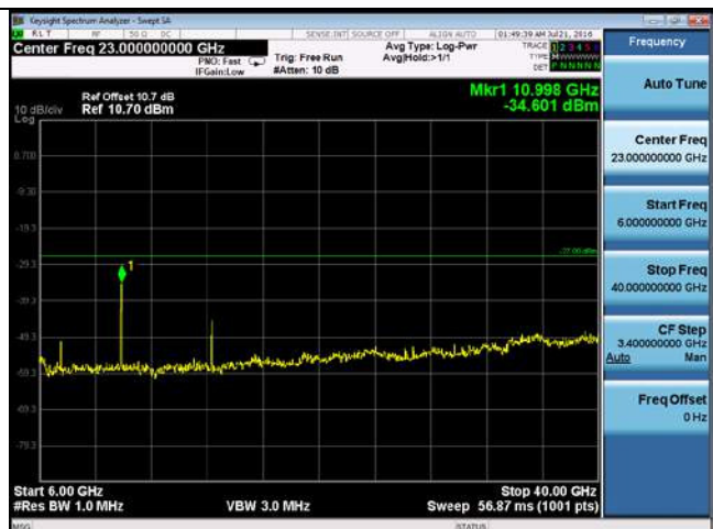
CUE-802.11n-20-5500M-chain4(6GHz-40GHz)
