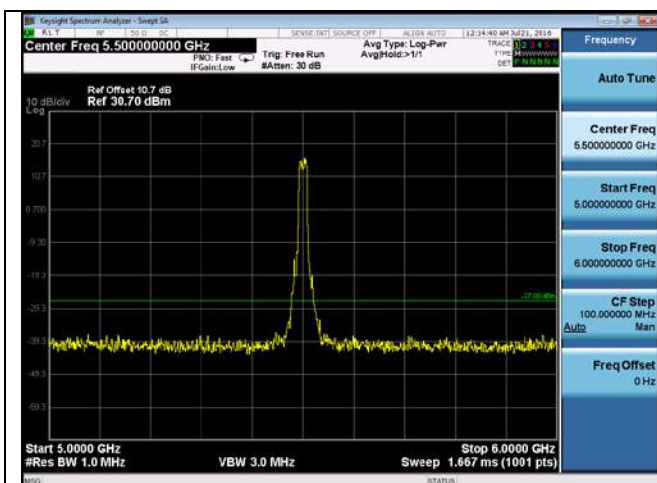
CUE-802.11a-5500M -chain2(5GHz-6GHz)
