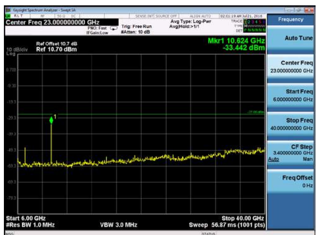
CUE-802.11n-20-5320M-chain 4(6GHz-40GHz)
