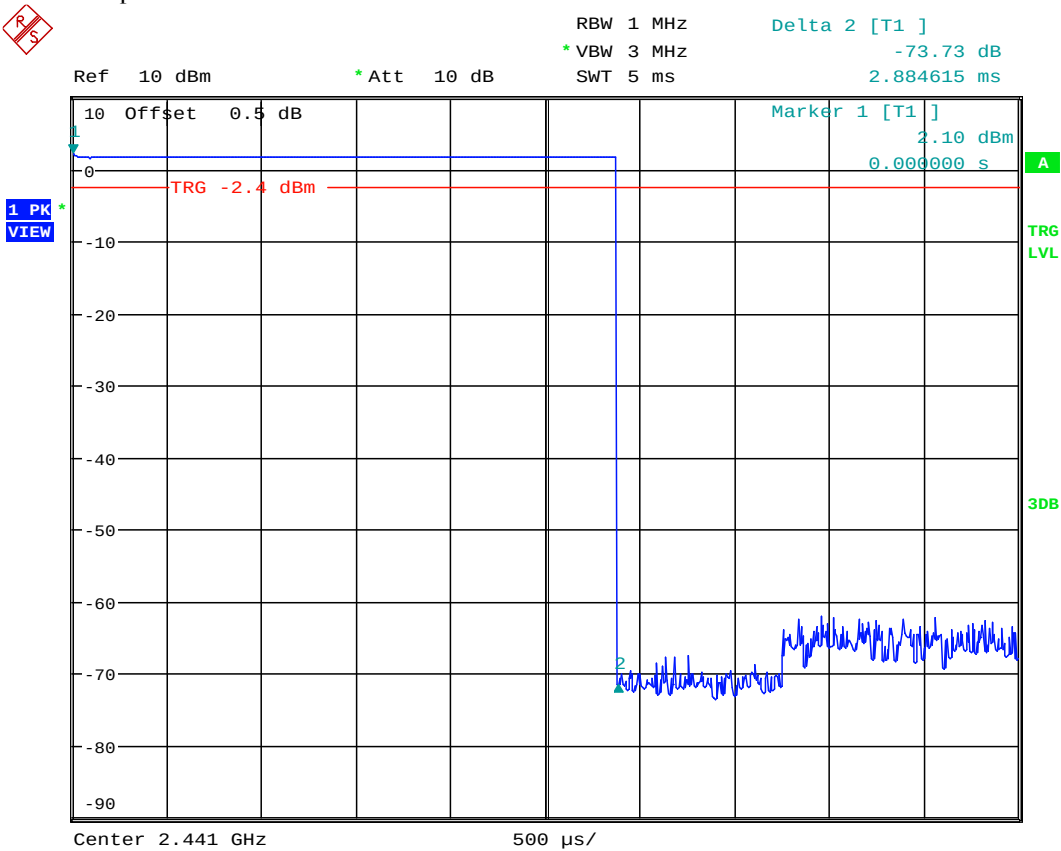
DH5 pulse's on time: 2.885ms
