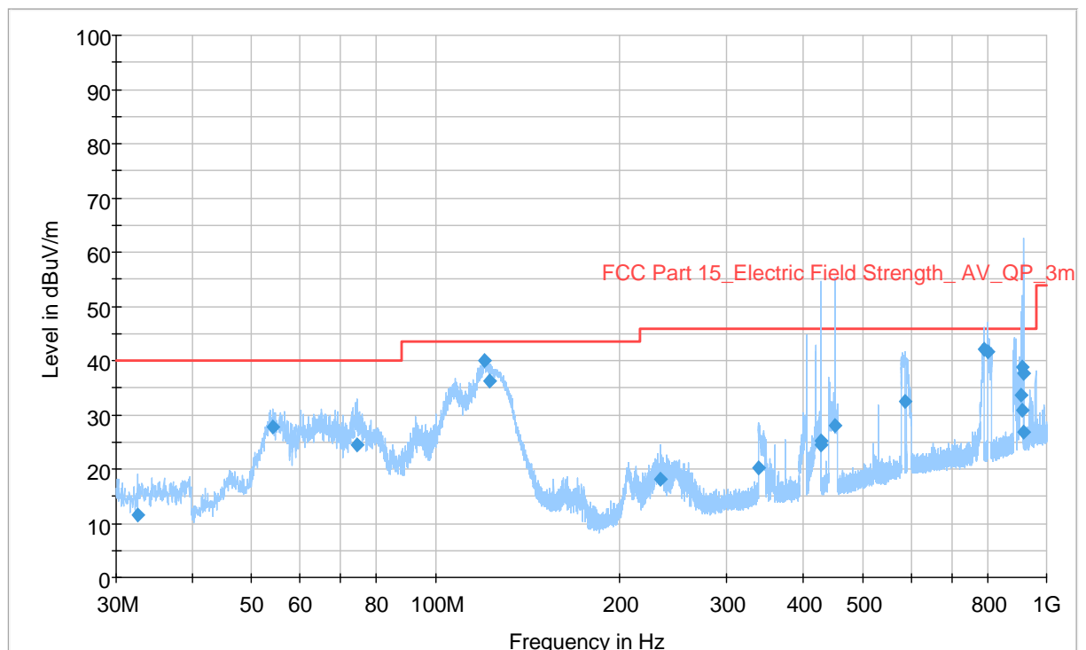
Plot 3.8.3 Radiated emission measurements in (30 – 1000) MHz range, vertical and horizontal polarization (460 MHz)
