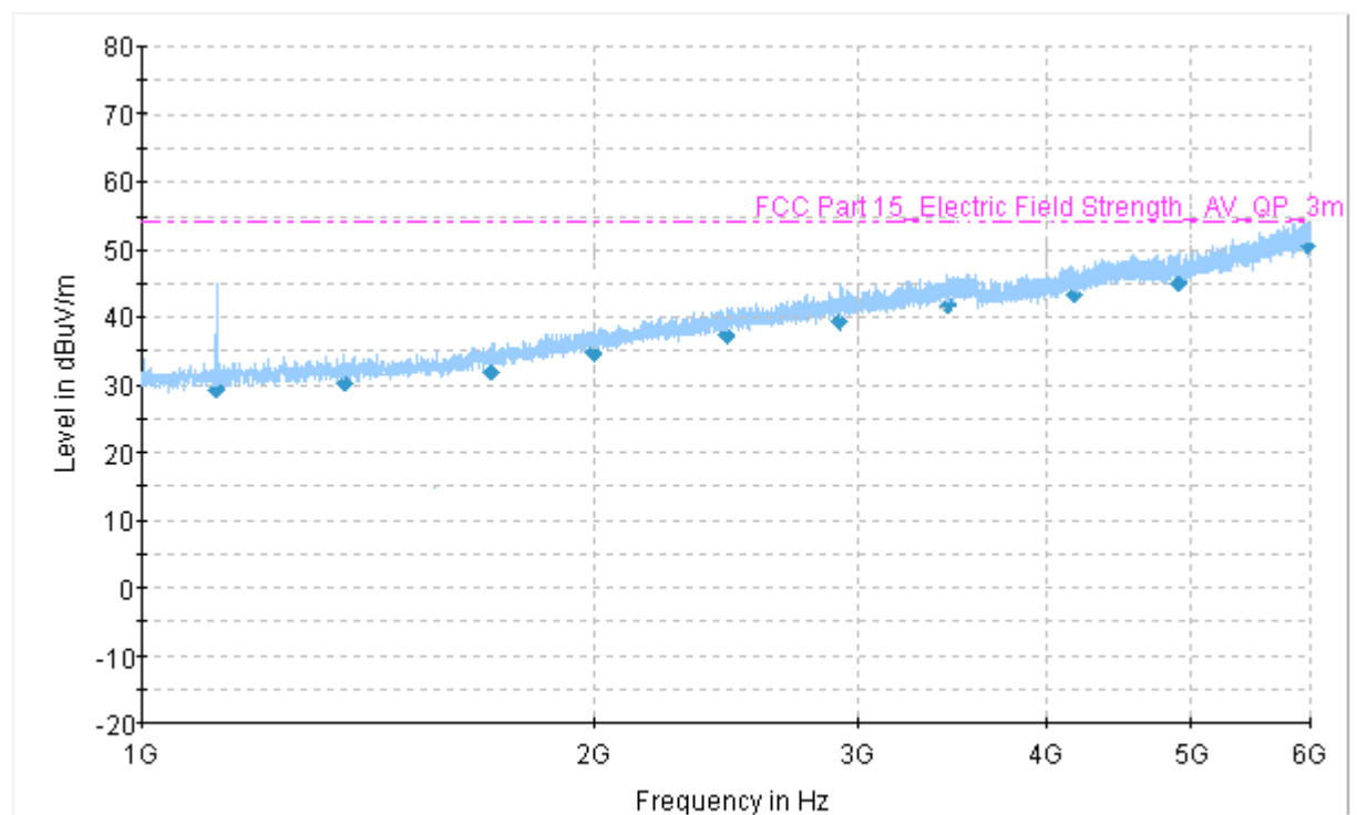
Plot 3.8.4 Radiated emission measurements in (1000 – 6000) MHz range, vertical and horizontal polarization (460 MHz)
