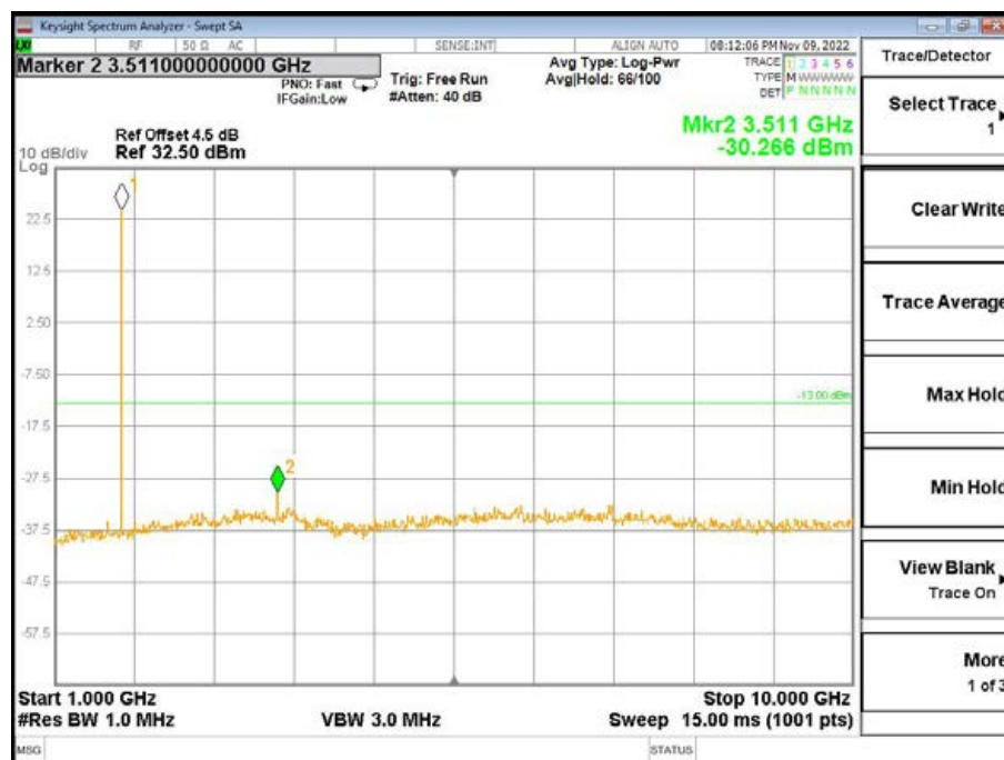
Band4-High Channel-15MHz Bandwidth-1RB-QPSK-1GHz to 10GHz
