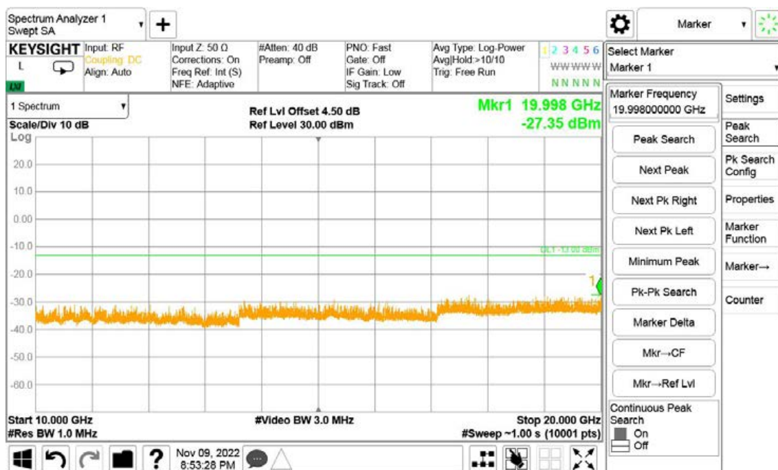
Band2-Low Channel-20MHz Bandwidth-1RB-QPSK-10GHz to 20GHz
