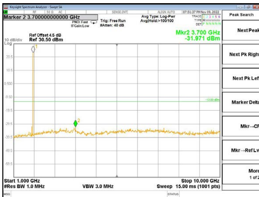
Band2-Low Channel-20MHz Bandwidth-1RB-QPSK-1GHz to 10GHz
