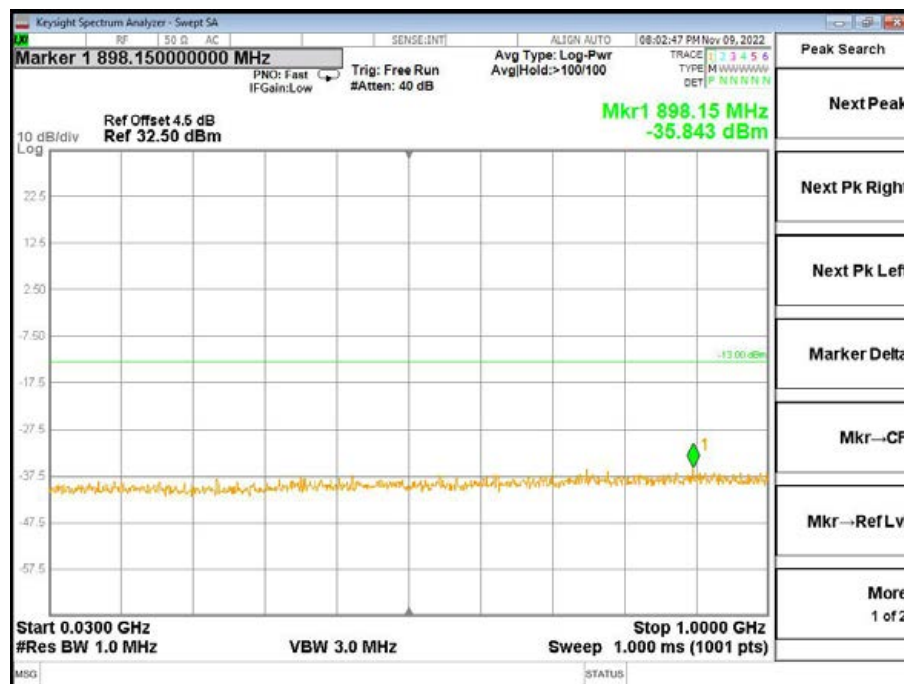
Band4-Low Channel-1.4MHz Bandwidth-1RB-QPSK-30MHz to 1GHz
