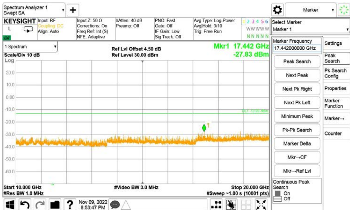
Band4-High Channel-1.4MHz Bandwidth-1RB-QPSK-10GHz to 20GHz
