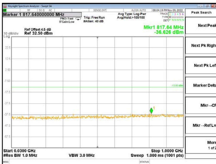
Band4-Middle Channel-10MHz Bandwidth-1RB-QPSK-30MHz to 1GHz
