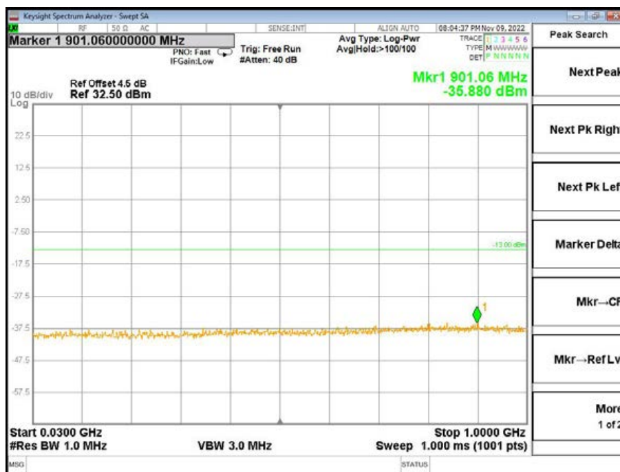
Band4-Middle Channel-3MHz Bandwidth-1RB-QPSK-30MHz to 1GHz
