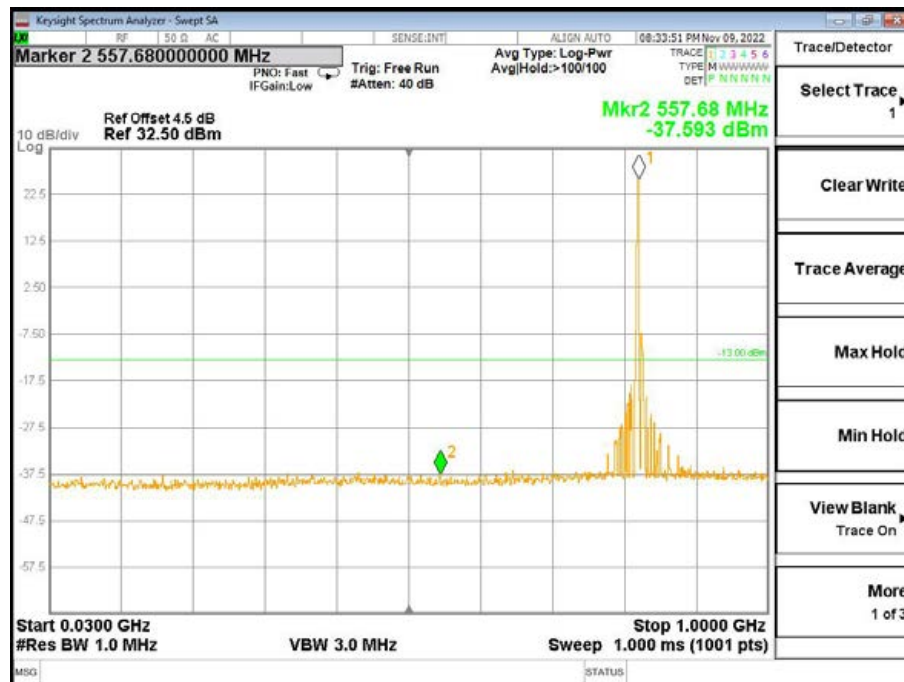
High Channel-1.4MHz Bandwidth-1RB-QPSK-30MHz to 1GHz
