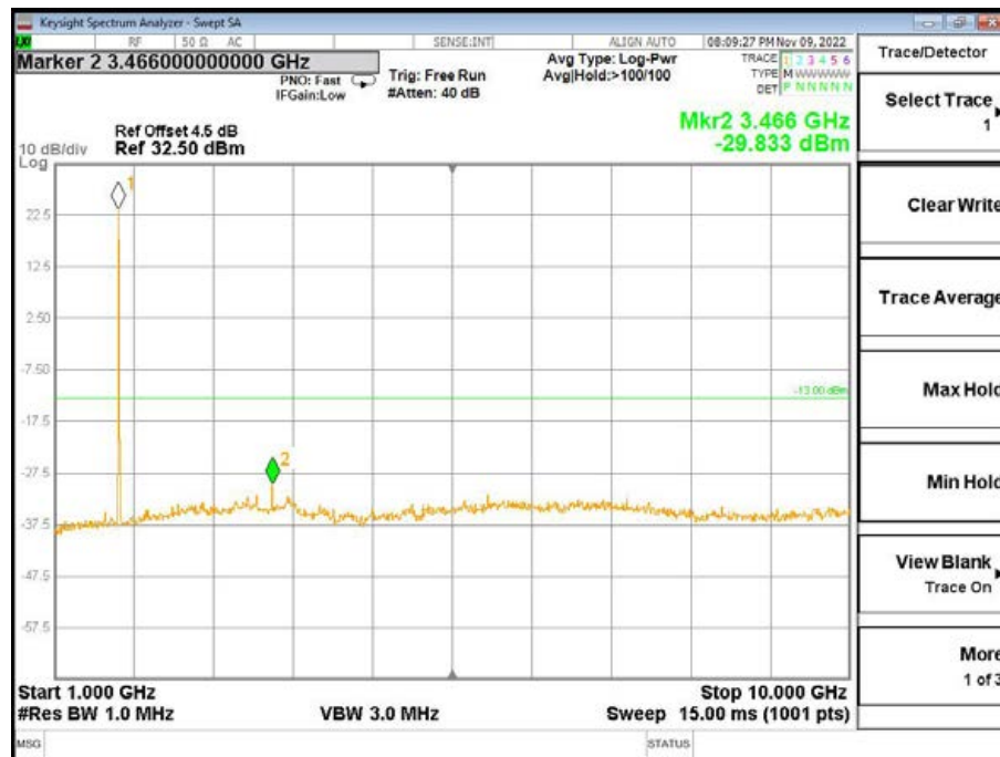
Band4-Middle Channel-3MHz Bandwidth-1RB-QPSK-1GHz to 10GHz
