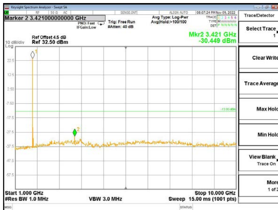
Band4-Low Channel-5MHz Bandwidth-1RB-QPSK-1GHz to 10GHz
