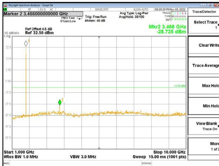
Band4-Middle Channel-5MHz Bandwidth-1RB-QPSK-1GHz to 10GHz
