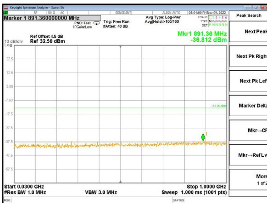
Band4-Middle Channel-20MHz Bandwidth-1RB-QPSK-30MHz to 1GHz
