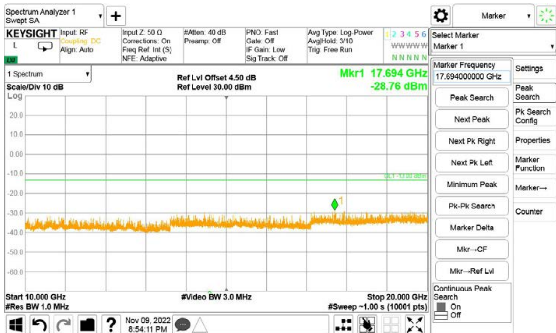
Band4-High Channel-5MHz Bandwidth-1RB-QPSK-10GHz to 20GHz
