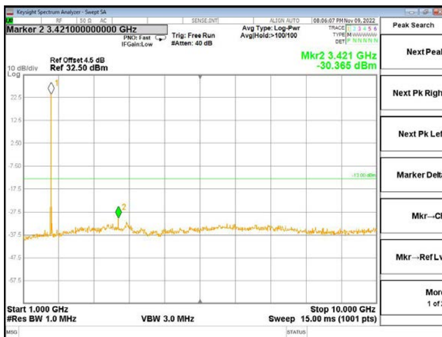
Band4-Low Channel-20MHz Bandwidth-1RB-QPSK-1GHz to 10GHz
