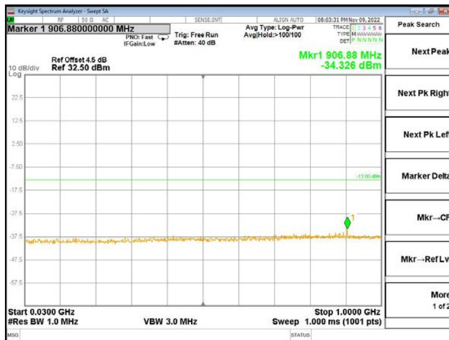
Band4-Low Channel-15MHz Bandwidth-1RB-QPSK-30MHz to 1GHz
