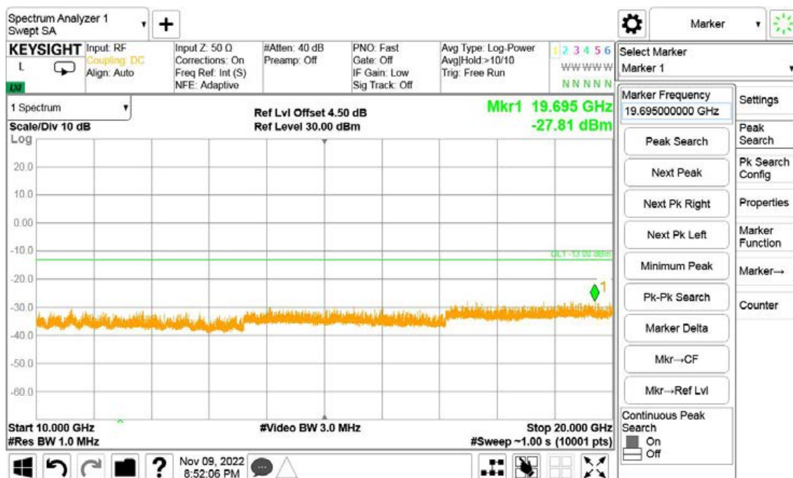
Band4-High Channel-15MHz Bandwidth-1RB-QPSK-10GHz to 20GHz
