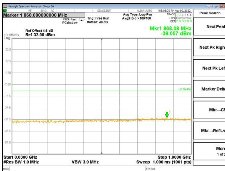
Band4-High Channel-20MHz Bandwidth-1RB-QPSK-30MHz to 1GHz
