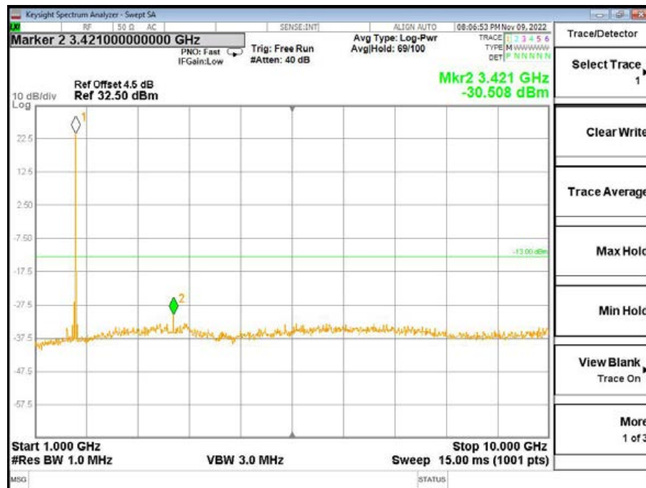
Band4-Low Channel-10MHz Bandwidth-1RB-QPSK-1GHz to 10GHz
