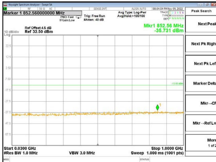
Band4-High Channel-1.4MHz Bandwidth-1RB-QPSK-30MHz to 1GHz
