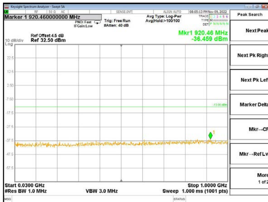
Band4-High Channel-5MHz Bandwidth-1RB-QPSK-30MHz to 1GHz
