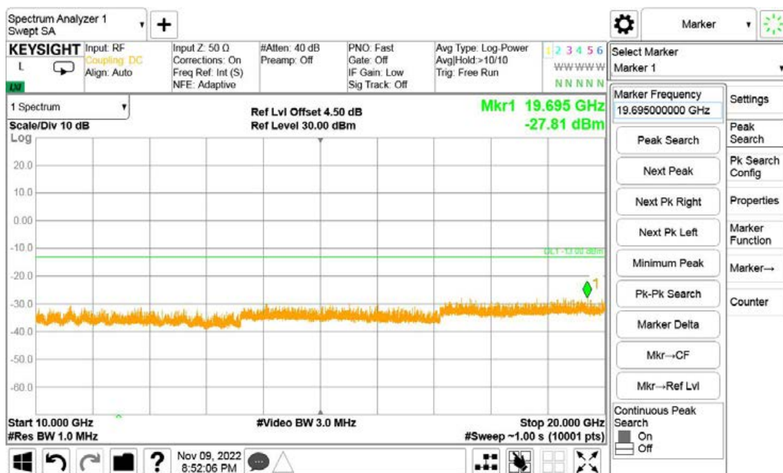
High Channel-3MHz Bandwidth-1RB-QPSK-10GHz to 20GHz
