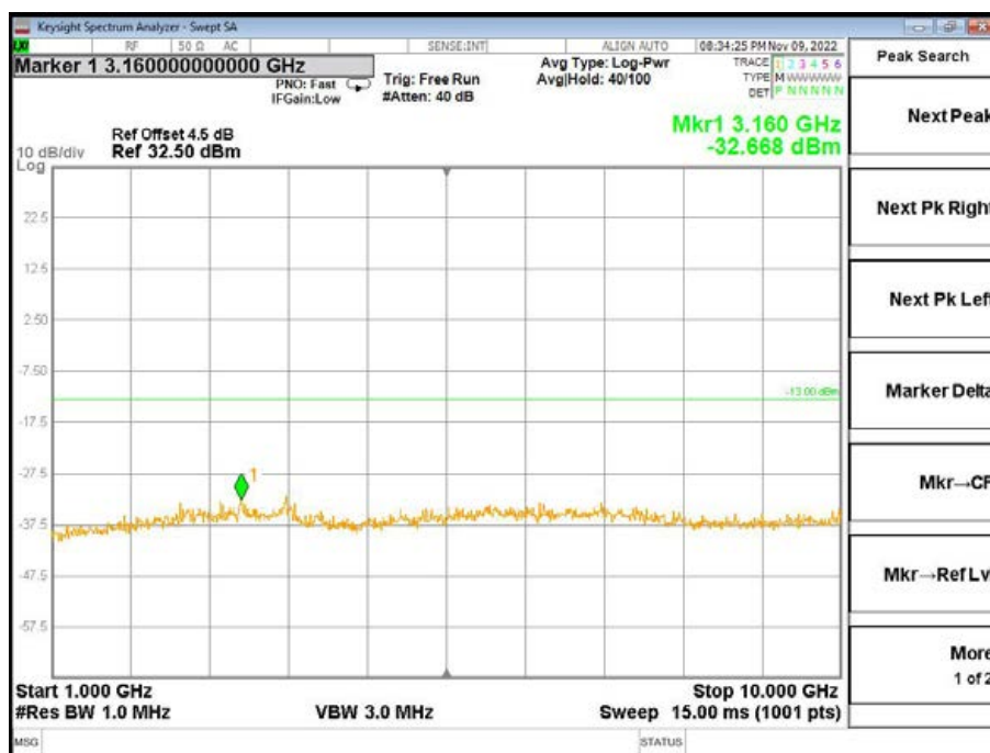
High Channel-3MHz Bandwidth-1RB-QPSK-1GHz to 10GHz
