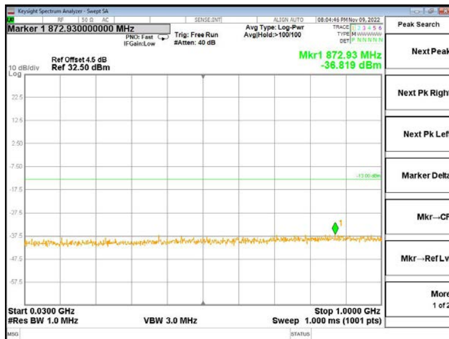
Band4-Middle Channel-1.4MHz Bandwidth-1RB-QPSK-30MHz to 1GHz
