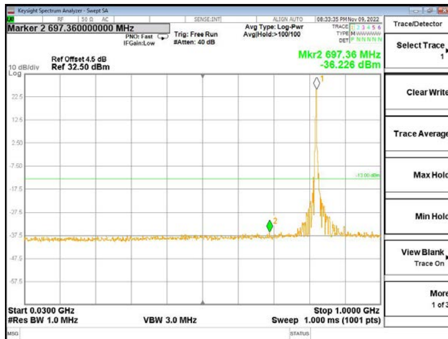
High Channel-3MHz Bandwidth-1RB-QPSK-30MHz to 1GHz
