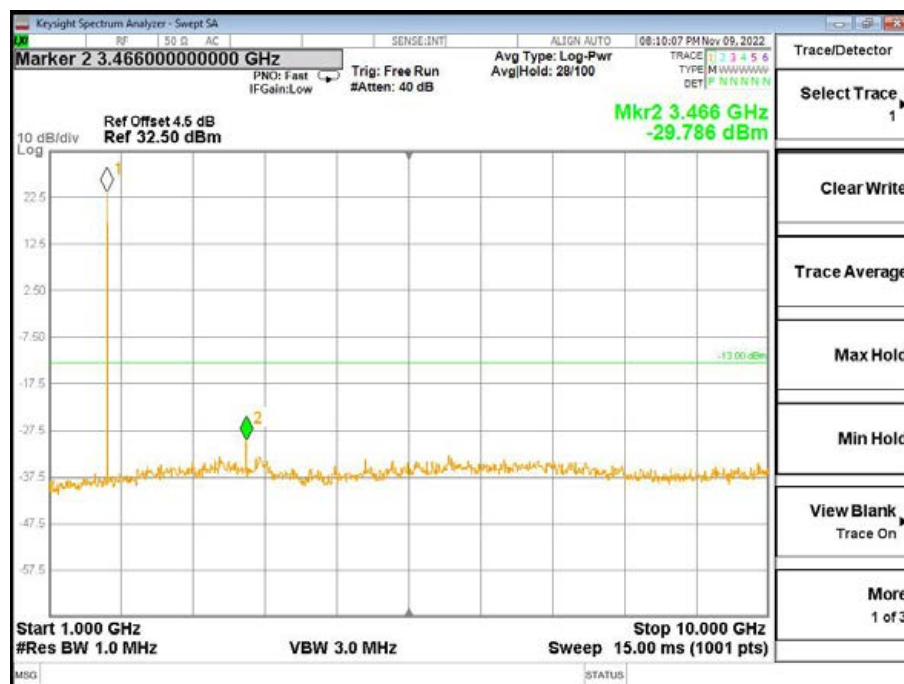
Band4-Middle Channel-15MHz Bandwidth-1RB-QPSK-1GHz to 10GHz
