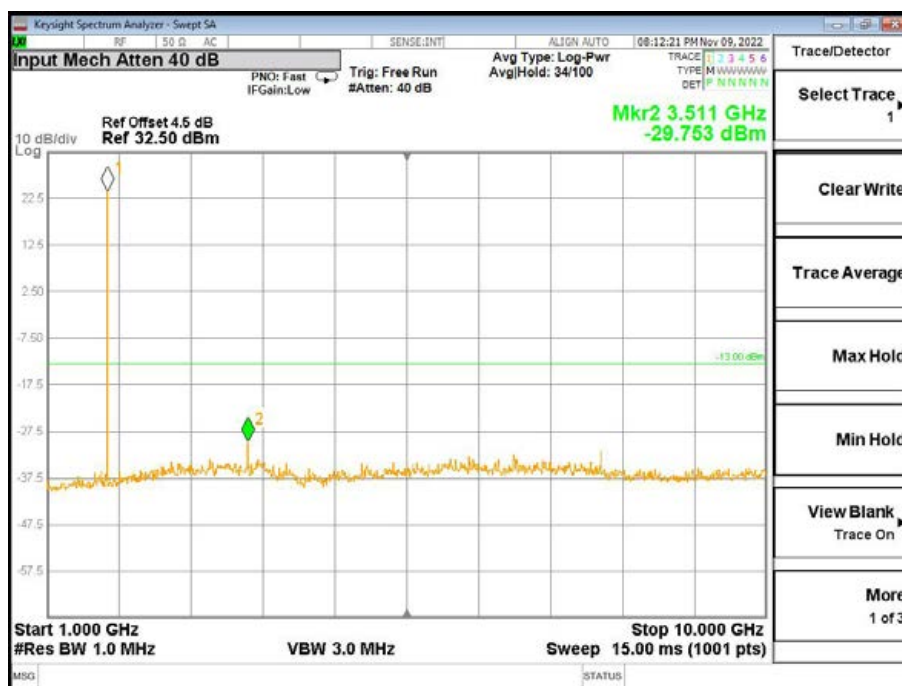
Band4-High Channel-10MHz Bandwidth-1RB-QPSK-1GHz to 10GHz
