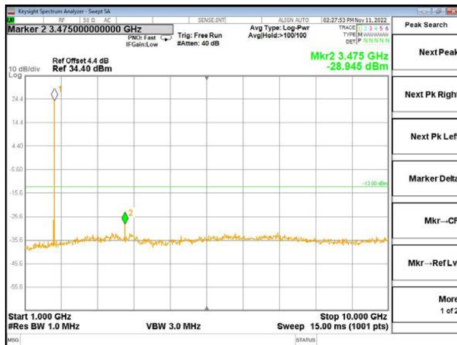
Band4-High Channel-20MHz Bandwidth-1RB-QPSK-1GHz to 10GHz
