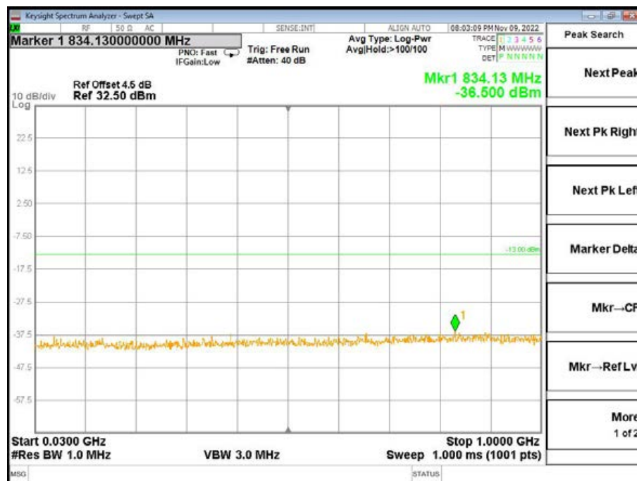
Band4-Low Channel-5MHz Bandwidth-1RB-QPSK-30MHz to 1GHz
