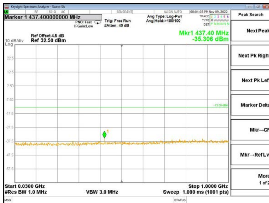
Band4-Middle Channel-15MHz Bandwidth-1RB-QPSK-30MHz to 1GHz
