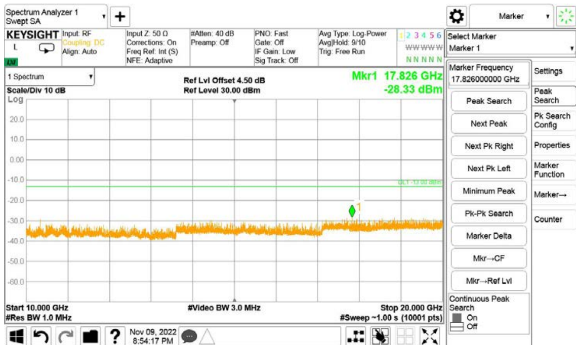
High Channel-1.4MHz Bandwidth-1RB-QPSK-10GHz to 20GHz
