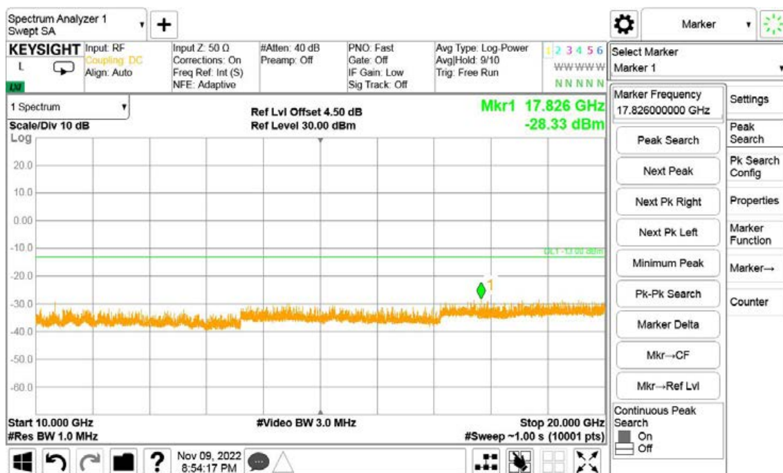
Band4-High Channel-10MHz Bandwidth-1RB-QPSK-10GHz to 20GHz
