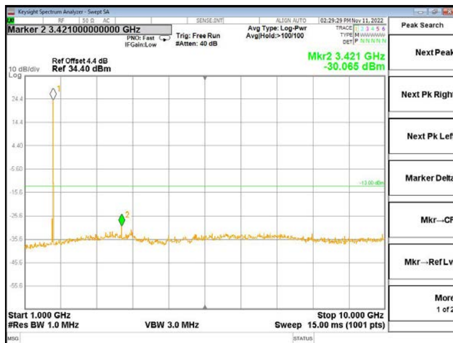
Band4-Middle Channel-1.4MHz Bandwidth-1RB-QPSK-1GHz to 10GHz
