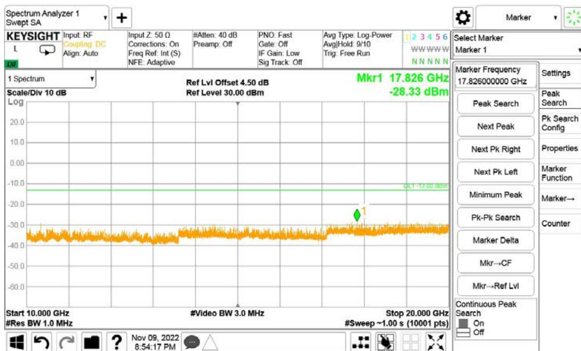
Band4-Low Channel-5MHz Bandwidth-1RB-QPSK-10GHz to 20GHz
