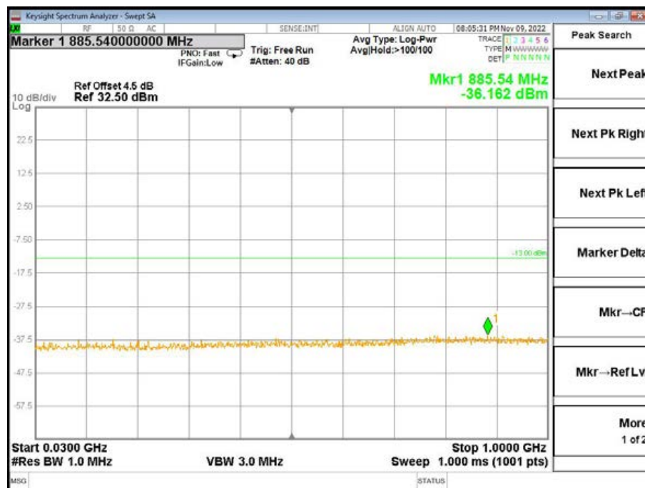
Band4-High Channel-15MHz Bandwidth-1RB-QPSK-30MHz to 1GHz
