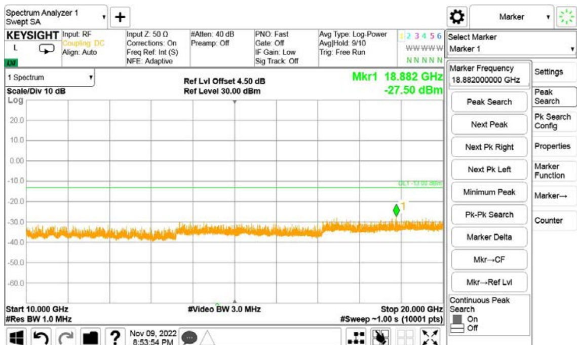
Band4-High Channel-3MHz Bandwidth-1RB-QPSK-10GHz to 20GHz
