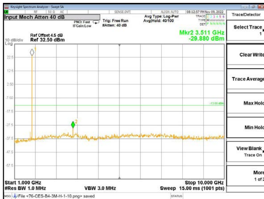
Band4-High Channel-1.4MHz Bandwidth-1RB-QPSK-1GHz to 10GHz
