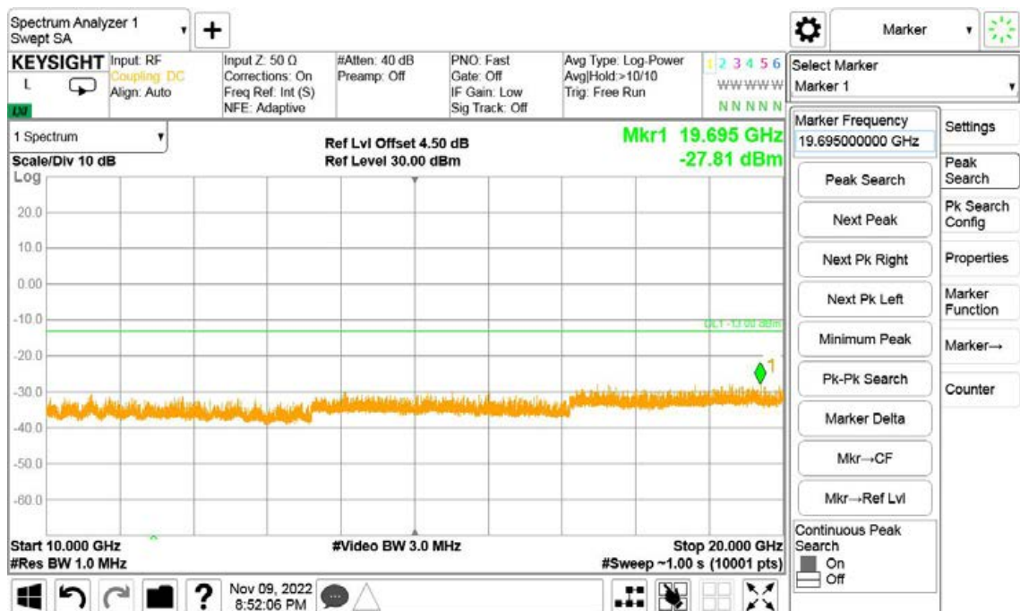
Band4-Low Channel-10MHz Bandwidth-1RB-QPSK-10GHz to 20GHz
