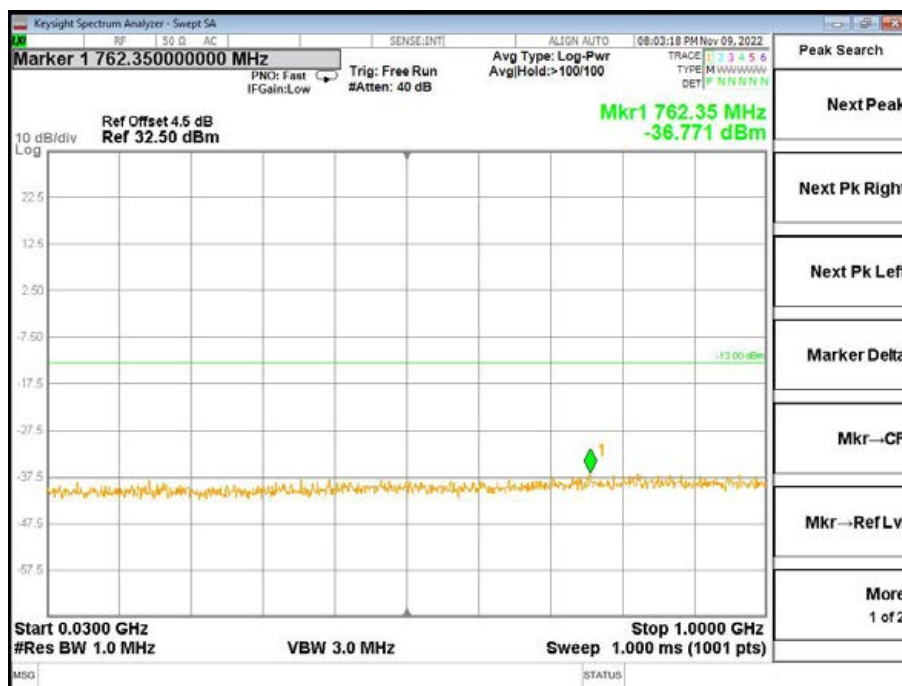
Band4-Low Channel-10MHz Bandwidth-1RB-QPSK-30MHz to 1GHz
