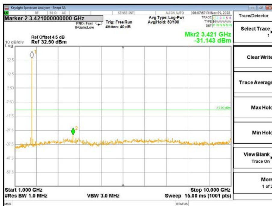
Band4-Low Channel-1.4MHz Bandwidth-1RB-QPSK-1GHz to 10GHz
