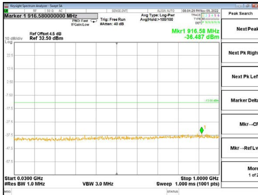
Band4-Middle Channel-5MHz Bandwidth-1RB-QPSK-30MHz to 1GHz
