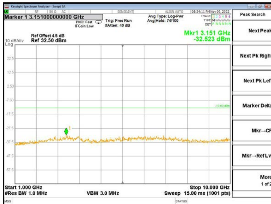
High Channel-1.4MHz Bandwidth-1RB-QPSK-1GHz to 10GHz
