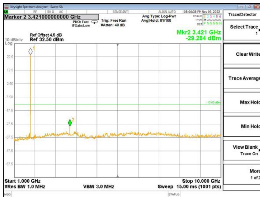
Band4-Low Channel-15MHz Bandwidth-1RB-QPSK-1GHz to 10GHz
