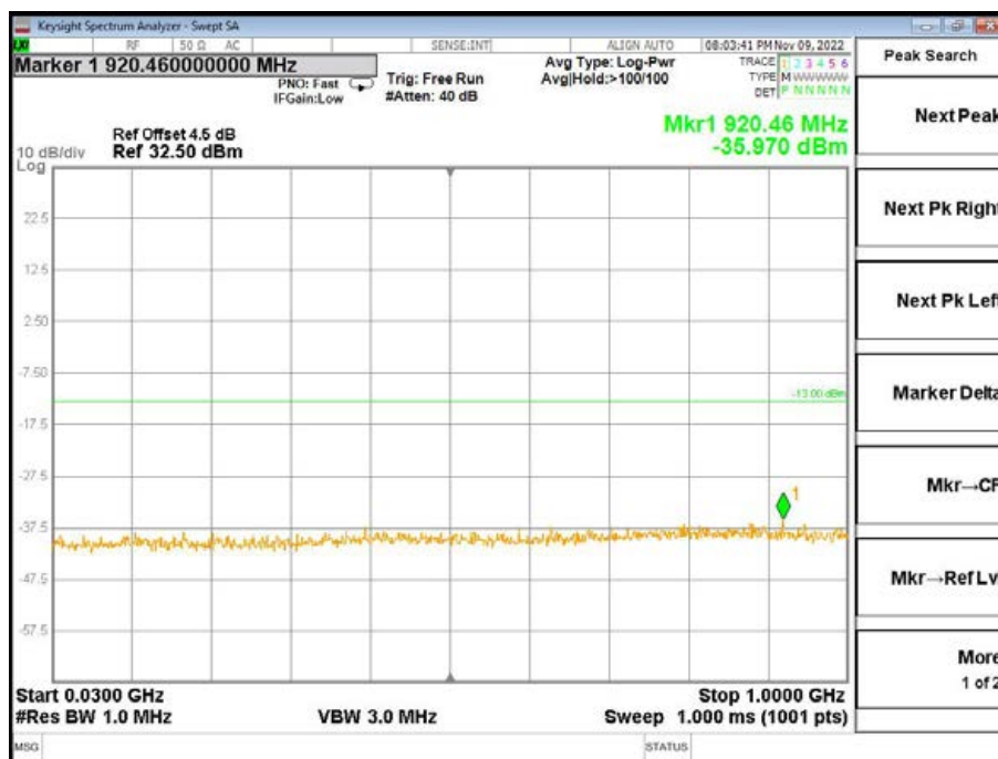
Band4-Low Channel-20MHz Bandwidth-1RB-QPSK-30MHz to 1GHz
