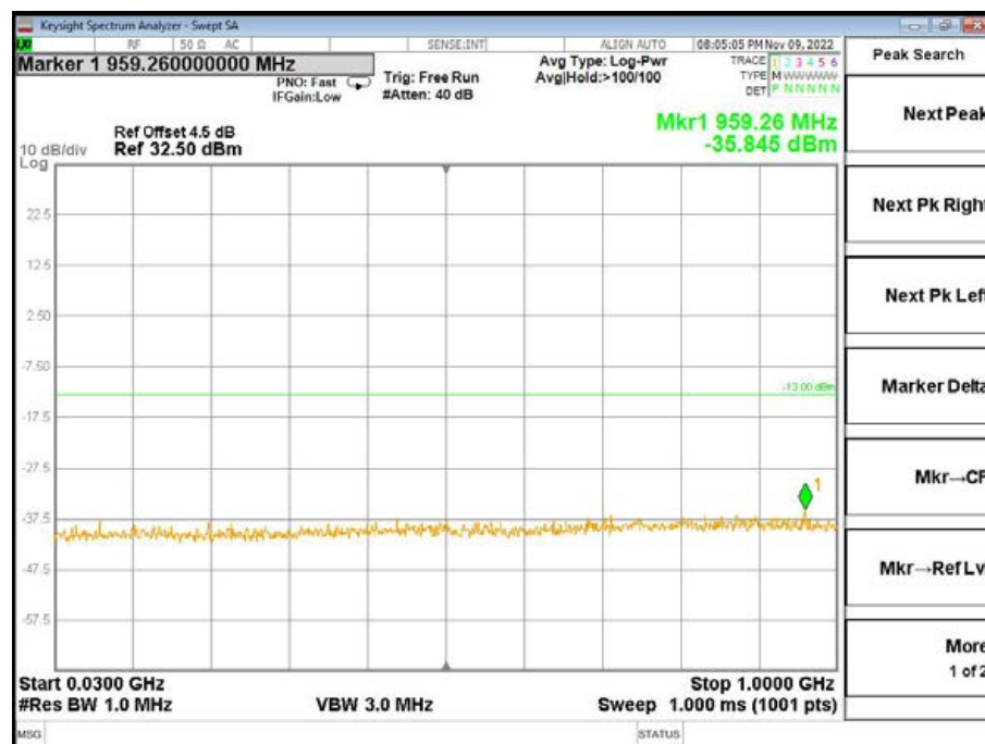
Band4-High Channel-3MHz Bandwidth-1RB-QPSK-30MHz to 1GHz
