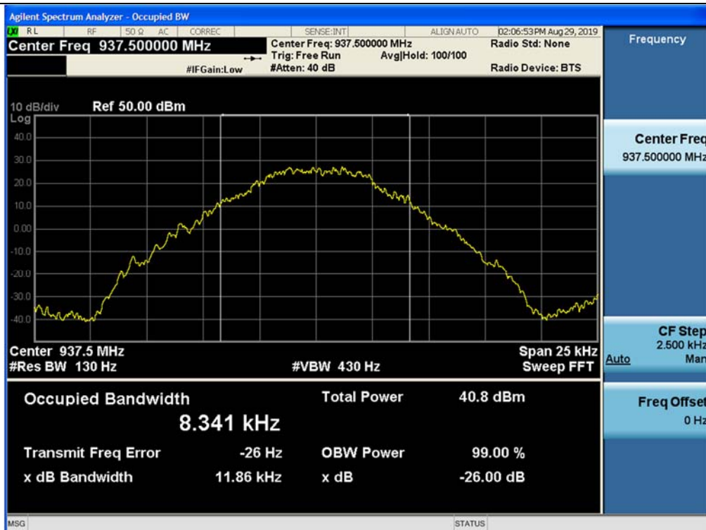
Output / 900I_PA(935 ~ 940 MHz) / Downlink
