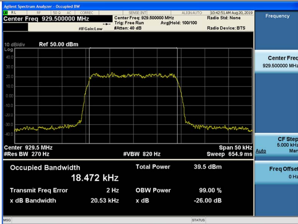
Output / 900I_PA(929 ~ 930 MHz) / Downlink
