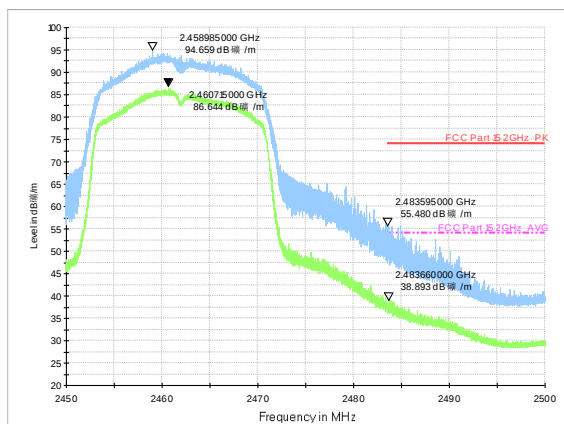
Test Mode: IEEE 802.11n20-High MIMO
