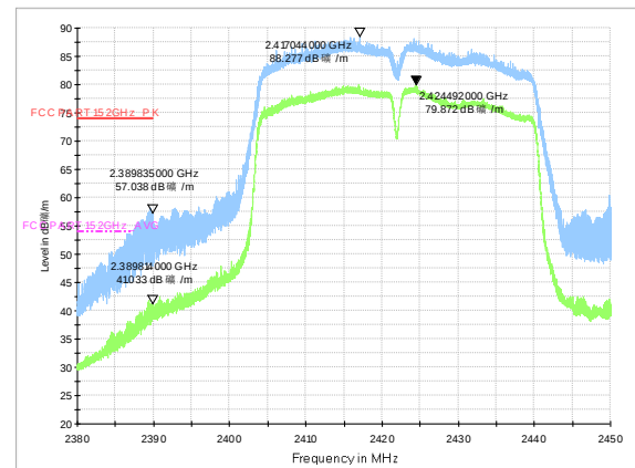
Test Mode: IEEE 802.11n40-Low MIMO
