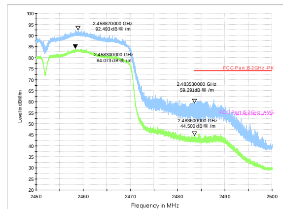
Test Mode: IEEE 802.11n40-High MIMO
