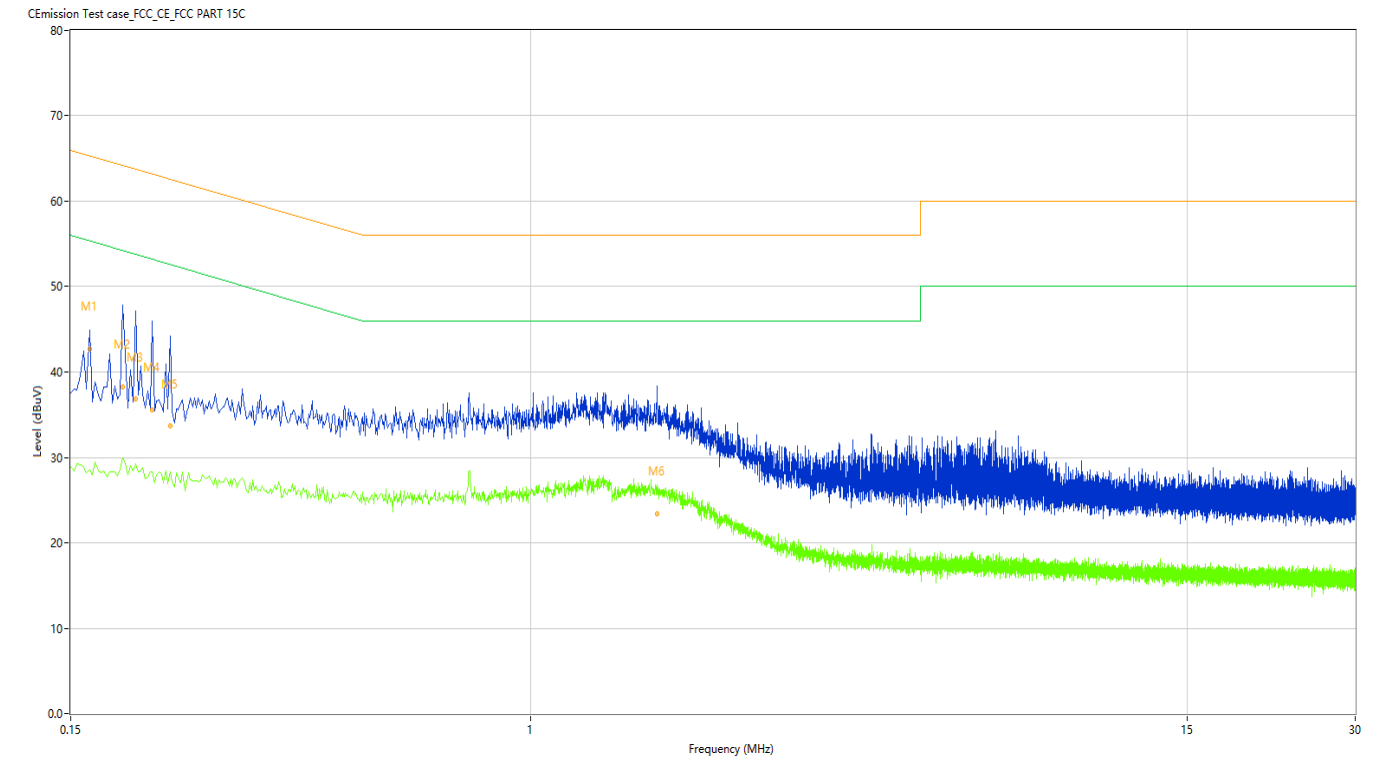
Figure 33: Conducted Emission on AC Mains, N Phase
