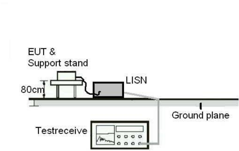
Diagram of Measurement Configuration for Conduction Test
