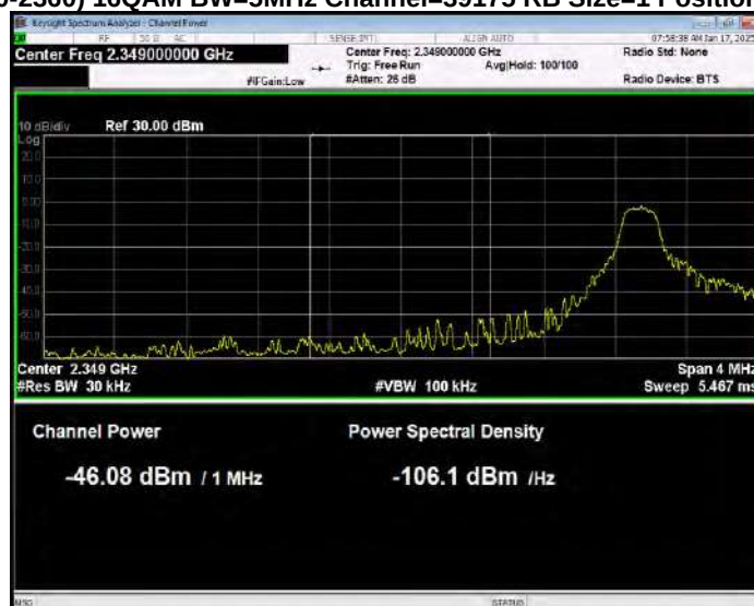
Band40(2350-2360) 16QAM BW=5MHz Channel=39175 RB Size=1 Position=#0 Normal
