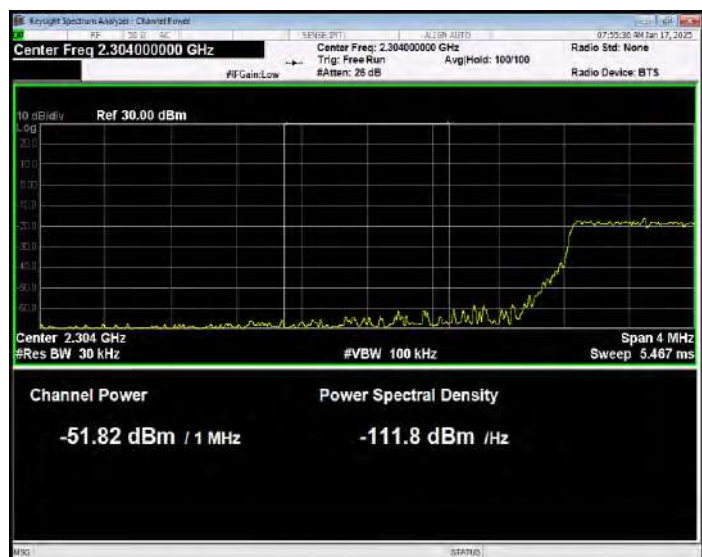
Band40(2305-2315) QPSK BW=5MHz Channel=38725 RB Size=25 Position=#0 Normal
