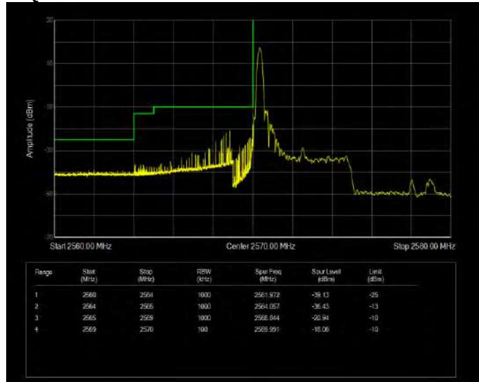
Band38 QPSK BW=5MHz Channel=37775 RB Size=1 Position=#Max Extended
