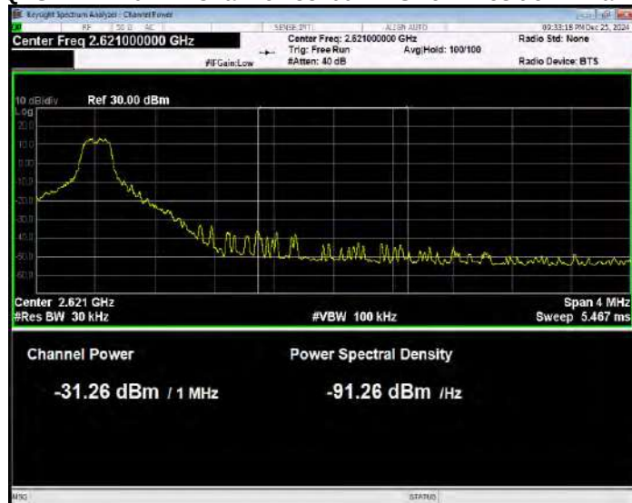
Band38 QPSK BW=10MHz Channel=38200 RB Size=1 Position=#Max Normal
