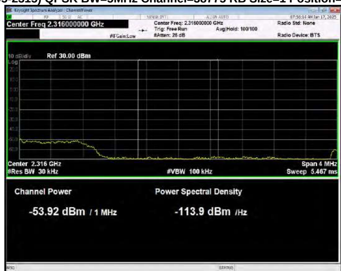
Band40(2305-2315) QPSK BW=5MHz Channel=38775 RB Size=1 Position=#0 Normal
