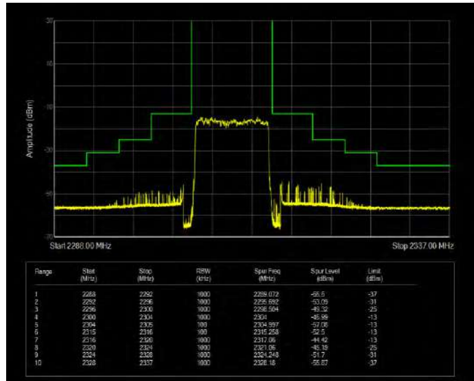
Band40(2305-2315) 16QAM BW=5MHz Channel=38725 RB Size=1 Position=#0 Extended
