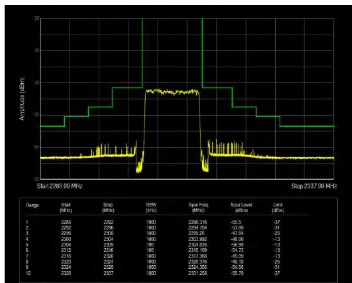
Band40(2305-2315) QPSK BW=5MHz Channel=38725 RB Size=1 Position=#0 Extended
