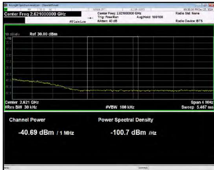
Band38 QPSK BW=20MHz Channel=38150 RB Size=1 Position=#0 Normal
