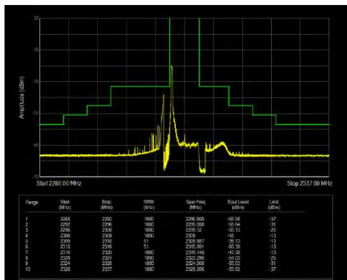
Band40(2305-2315) QPSK BW=5MHz Channel=38775 RB Size=25 Position=#0 Extended
