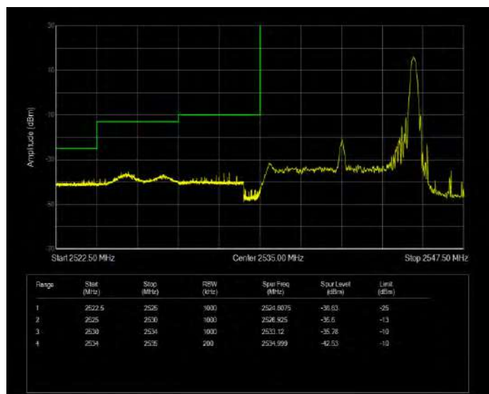
Band41(2535-2655) 16QAM BW=10MHz Channel=40090 RB Size=50 Position=#0 Extended
