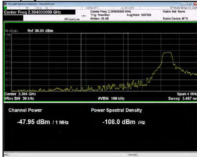
Band40(2305-2315) 16QAM BW=5MHz Channel=38725 RB Size=1 Position=#0 Normal
