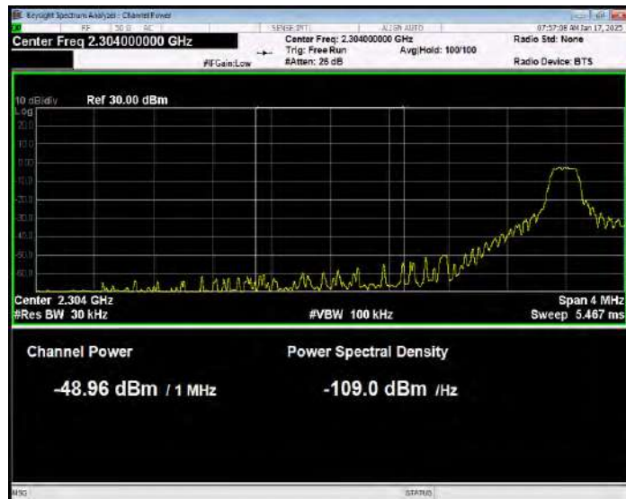
Band40(2305-2315) QPSK BW=10MHz Channel=38750 RB Size=1 Position=#0 Normal
