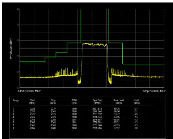
Band40(2350-2360) QPSK BW=5MHz Channel=39175 RB Size=1 Position=#0 Extended
