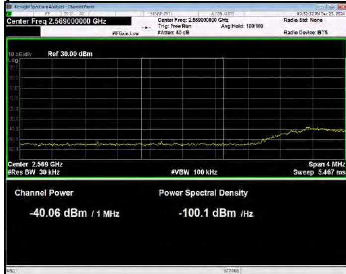
Band38 QPSK BW=10MHz Channel=37800 RB Size=1 Position=#Max Normal
