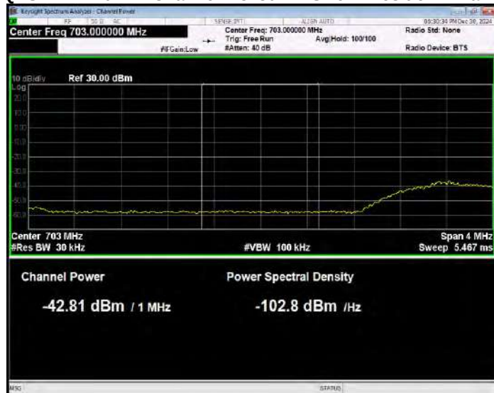
Band17 QPSK BW=10MHz Channel=23780 RB Size=1 Position=#Max Normal
