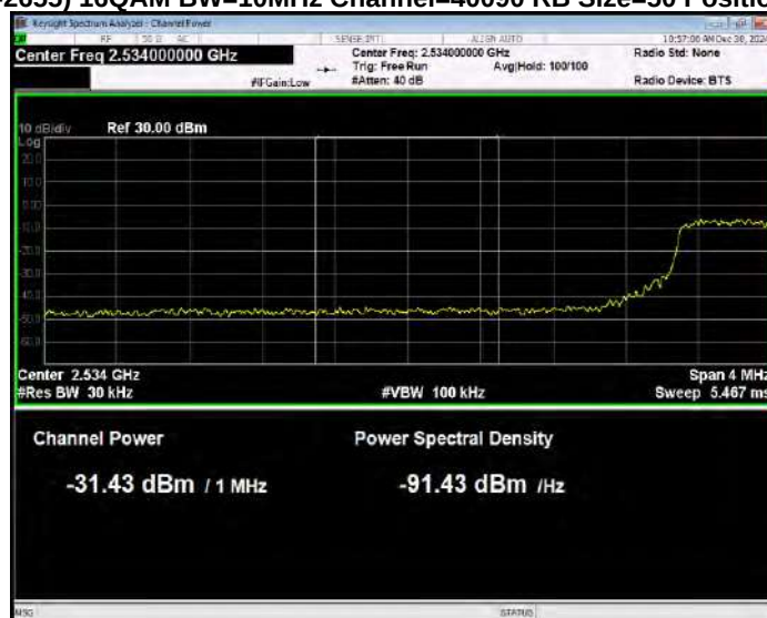
Band41(2535-2655) 16QAM BW=10MHz Channel=40090 RB Size=50 Position=#0 Normal
