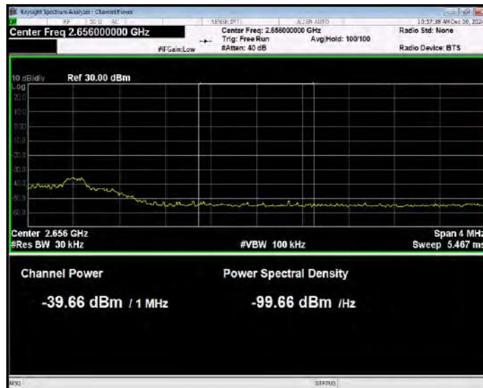
Band41(2535-2655) 16QAM BW=10MHz Channel=41190 RB Size=1 Position=#0 Normal
