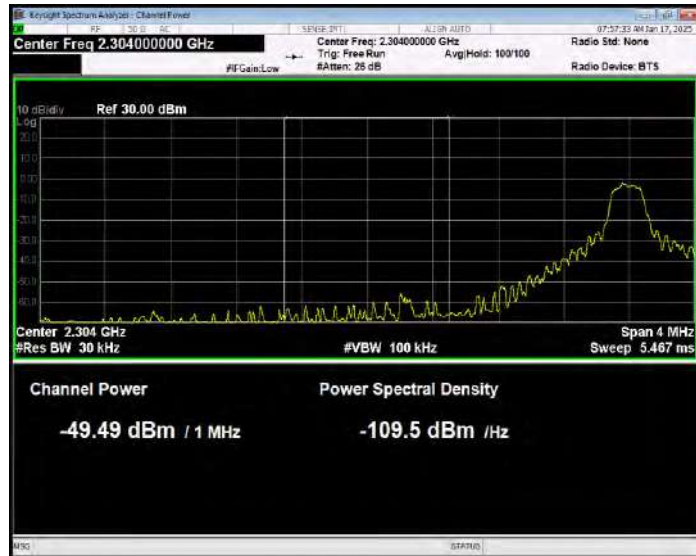
Band40(2305-2315) 16QAM BW=10MHz Channel=38750 RB Size=1 Position=#0 Normal
