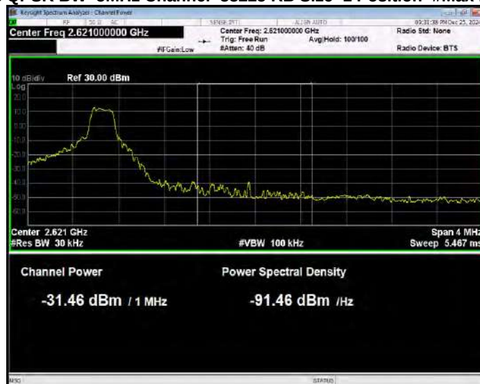
Band38 QPSK BW=5MHz Channel=38225 RB Size=1 Position=#Max Normal
