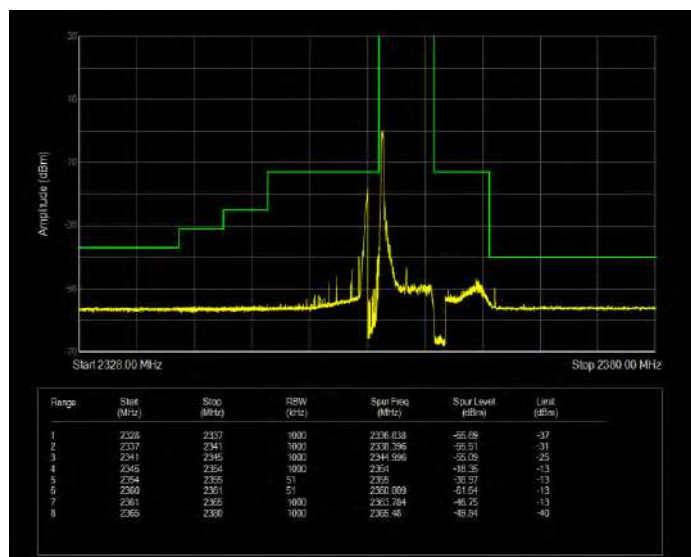
Band40(2350-2360) QPSK BW=5MHz Channel=39225 RB Size=25 Position=#0 Extended
