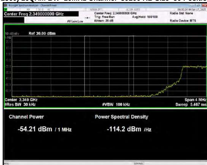
Band40(2350-2360) 16QAM BW=10MHz Channel=39200 RB Size=50 Position=#0 Normal
