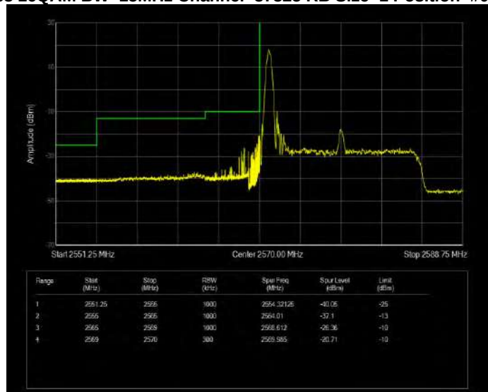
Band38 16QAM BW=15MHz Channel=37825 RB Size=1 Position=#Max Extended
