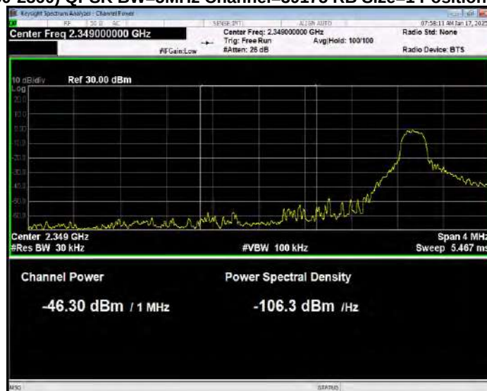
Band40(2350-2360) QPSK BW=5MHz Channel=39175 RB Size=1 Position=#0 Normal
