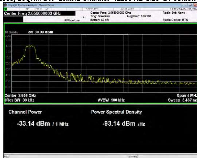
Band41(2535-2655) 16QAM BW=10MHz Channel=41190 RB Size=1 Position=#Max Normal
