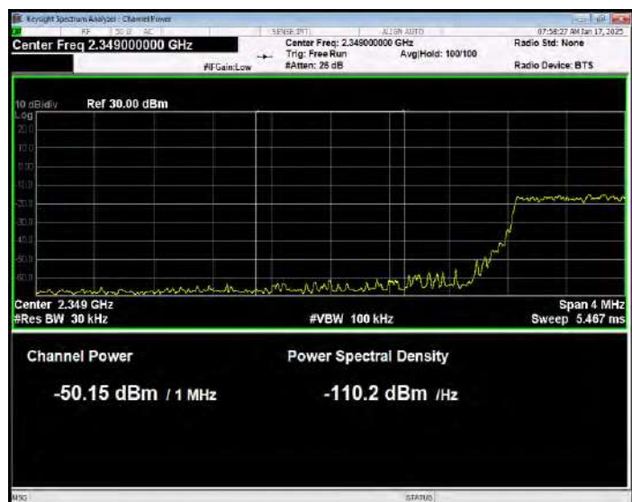
Band40(2350-2360) QPSK BW=5MHz Channel=39175 RB Size=25 Position=#0 Normal
