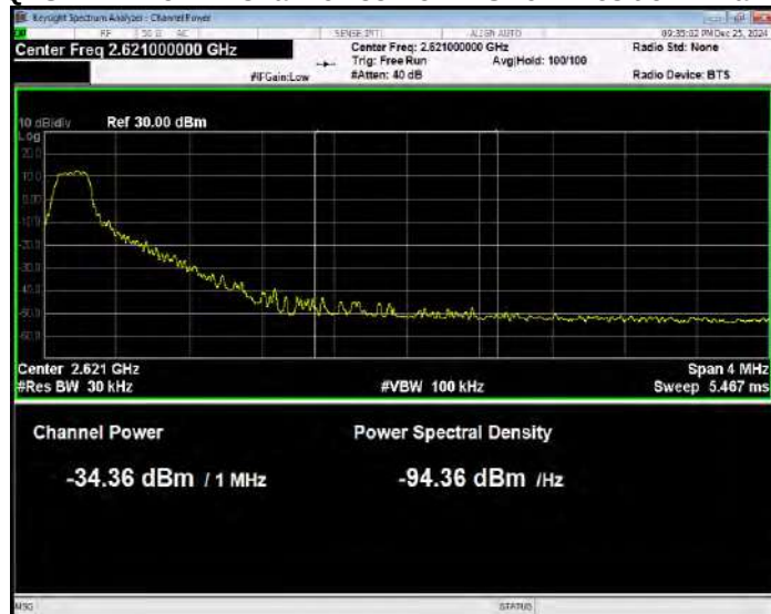
Band38 QPSK BW=15MHz Channel=38175 RB Size=1 Position=#Max Normal
