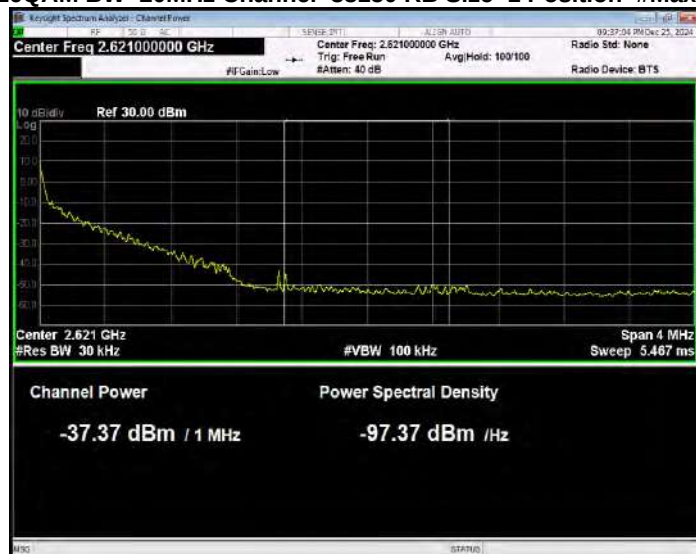
Band38 16QAM BW=20MHz Channel=38150 RB Size=1 Position=#Max Normal
