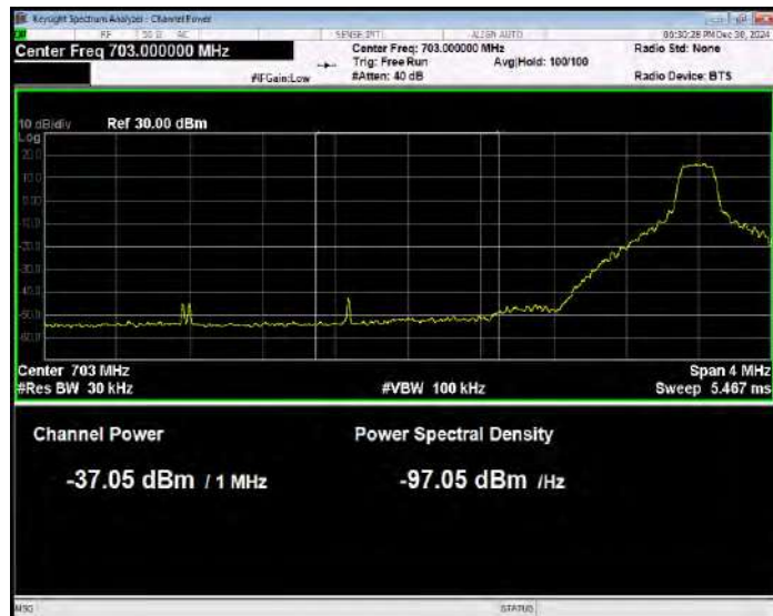
Band17 QPSK BW=10MHz Channel=23780 RB Size=1 Position=#0 Normal
