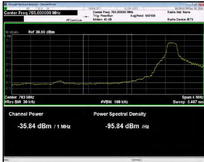
Band17 QPSK BW=5MHz Channel=23755 RB Size=1 Position=#0 Normal
