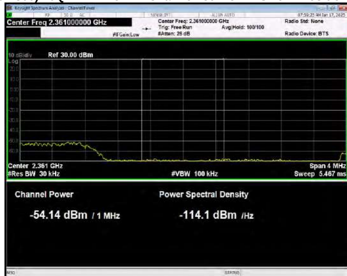
Band40(2350-2360) 16QAM BW=5MHz Channel=39225 RB Size=1 Position=#0 Normal
