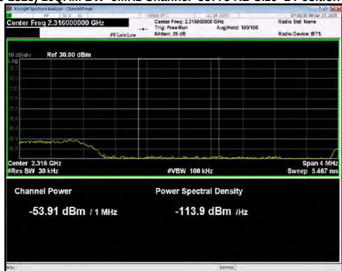
Band40(2305-2315) 16QAM BW=5MHz Channel=38775 RB Size=1 Position=#0 Normal
