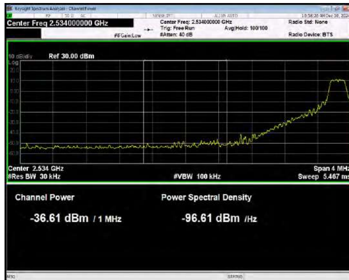
Band41(2535-2655) 16QAM BW=15MHz Channel=40115 RB Size=1 Position=#0 Normal
