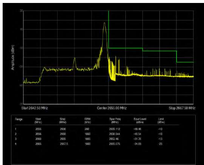
Band41(2535-2655) 16QAM BW=10MHz Channel=41190 RB Size=50 Position=#0 Extended
