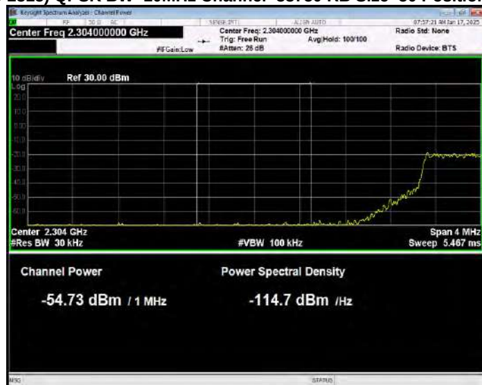
Band40(2305-2315) QPSK BW=10MHz Channel=38750 RB Size=50 Position=#0 Normal
