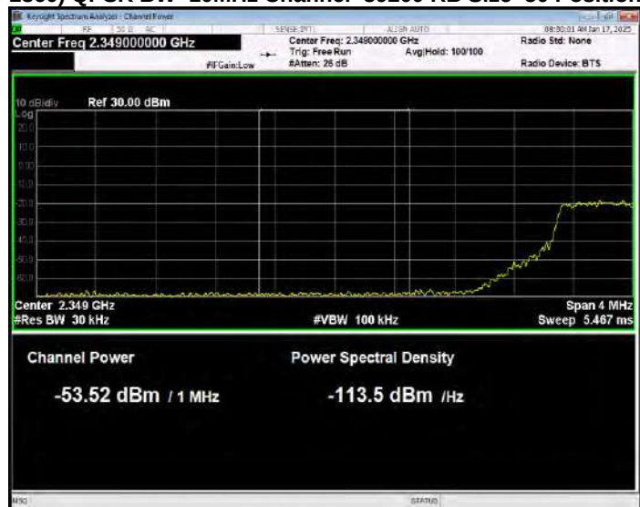
Band40(2350-2360) QPSK BW=10MHz Channel=39200 RB Size=50 Position=#0 Normal
