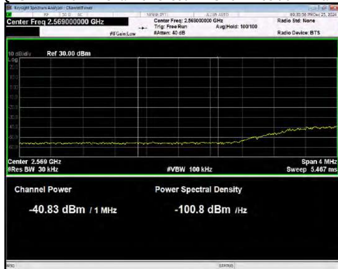
Band38 QPSK BW=20MHz Channel=37850 RB Size=1 Position=#Max Normal
