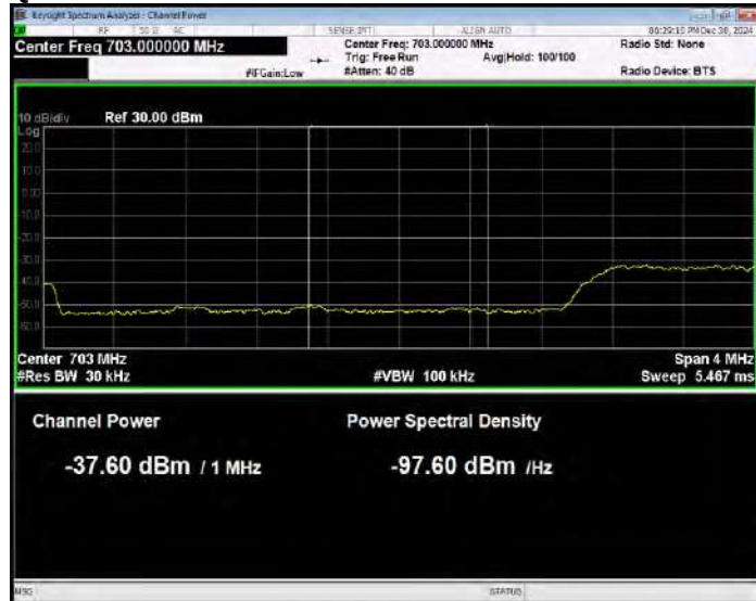
Band17 QPSK BW=5MHz Channel=23755 RB Size=1 Position=#Max Normal
