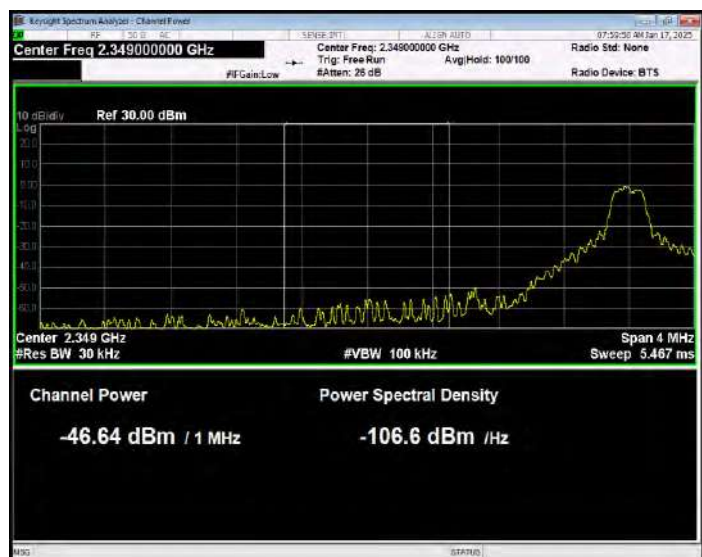
Band40(2350-2360) QPSK BW=10MHz Channel=39200 RB Size=1 Position=#0 Normal
