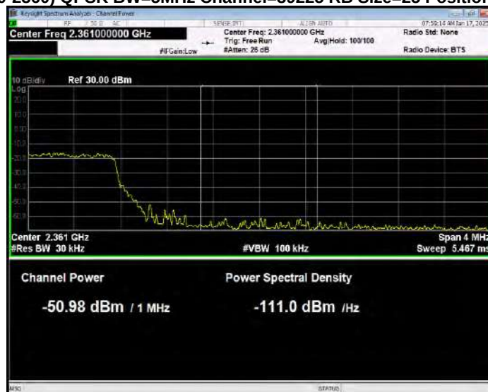
Band40(2350-2360) QPSK BW=5MHz Channel=39225 RB Size=25 Position=#0 Normal
