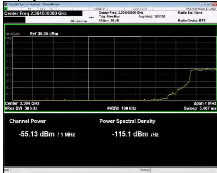
Band40(2305-2315) 16QAM BW=10MHz Channel=38750 RB Size=50 Position=#0 Normal
