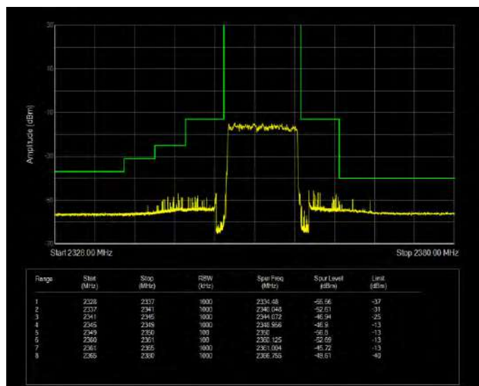
Band40(2350-2360) 16QAM BW=5MHz Channel=39175 RB Size=1 Position=#0 Extended
