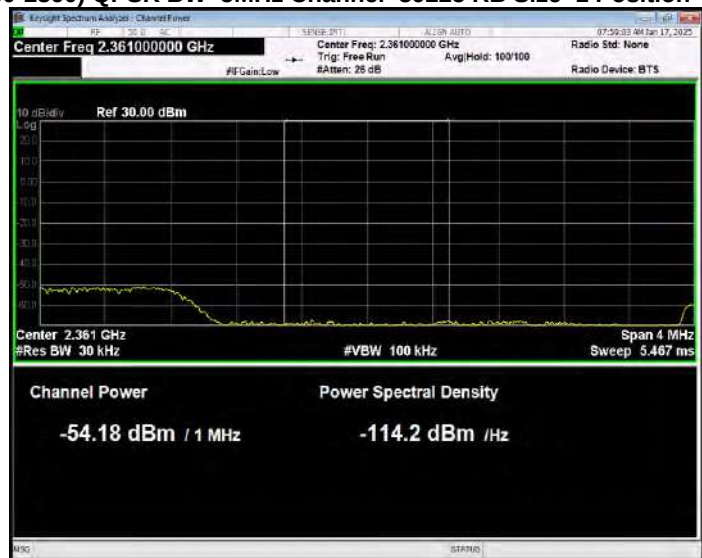
Band40(2350-2360) QPSK BW=5MHz Channel=39225 RB Size=1 Position=#0 Normal
