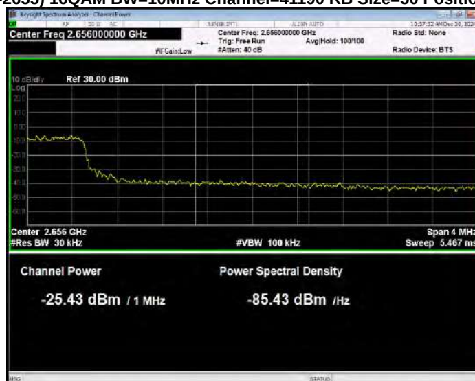
Band41(2535-2655) 16QAM BW=10MHz Channel=41190 RB Size=50 Position=#0 Normal
