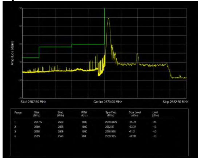
Band38 QPSK BW=10MHz Channel=37800 RB Size=1 Position=#Max Extended
