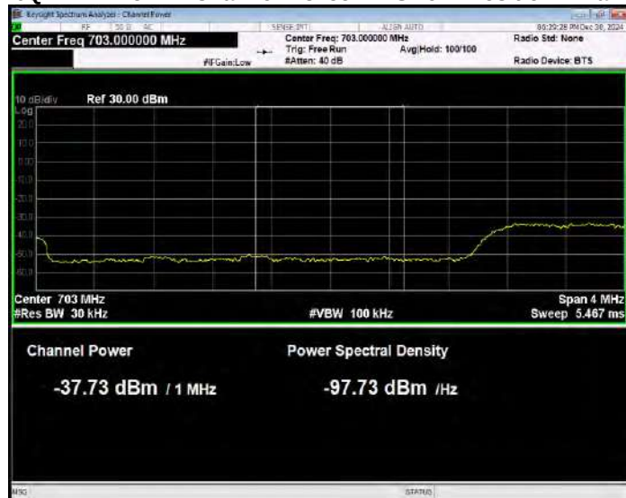
Band17 16QAM BW=5MHz Channel=23755 RB Size=1 Position=#Max Normal
