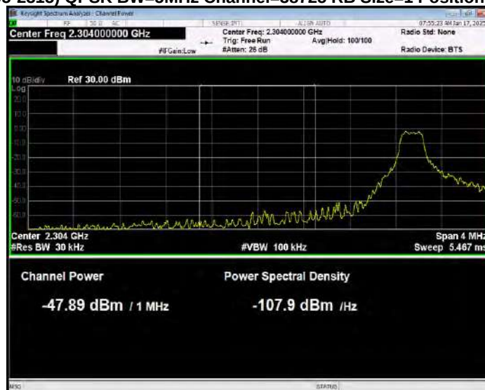
Band40(2305-2315) QPSK BW=5MHz Channel=38725 RB Size=1 Position=#0 Normal
