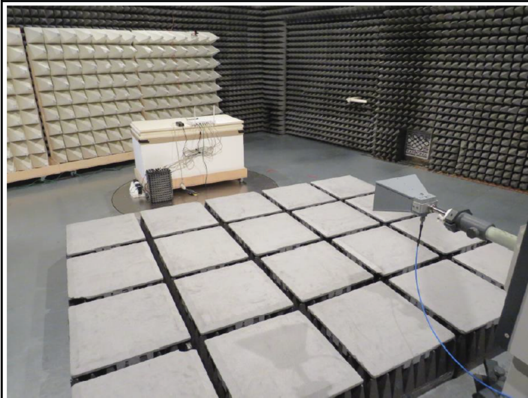
TEST SETUP 1-17GHz
