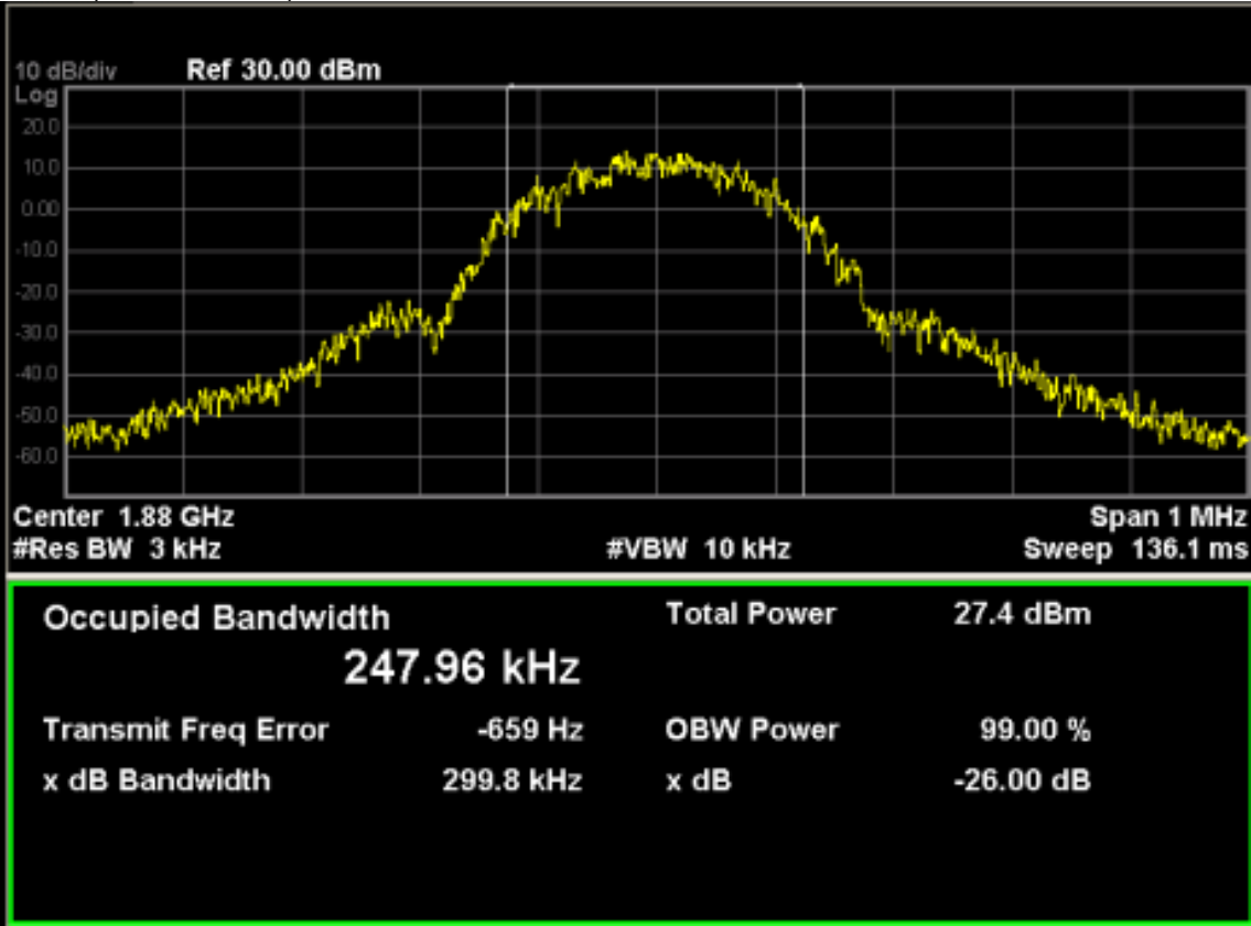
GSM1900 (EDGE 8 Link), Channel 661
