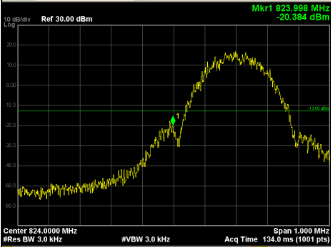
GSM850 (EDGE 8 Link), Channel 128
