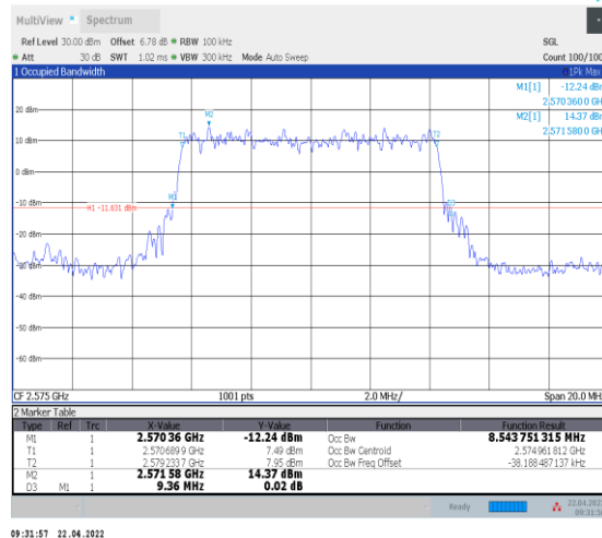
1-N38--30-10-L-2-DFT-PI2BPSK-Outer_Full-24@0-Ant0 -8.544-9.360-≤10-PASS
