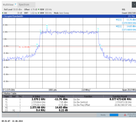
1-N38--30-10-L-1-DFT-QPSK-Outer_Full-24@0-Ant0 -8.577-9.400-≤10-PASS
