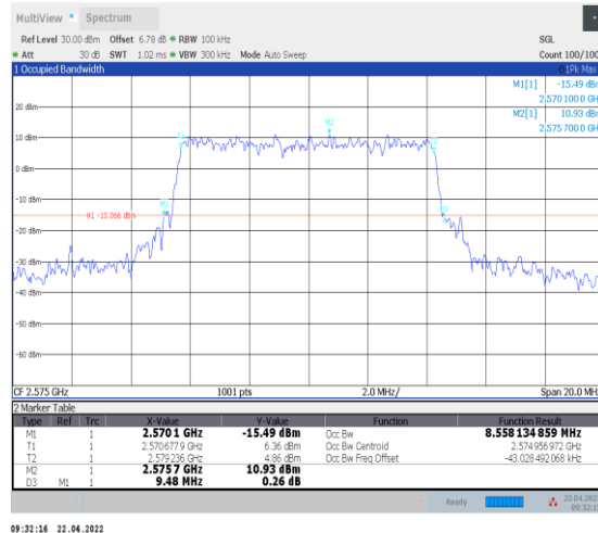
1-N38--30-10-L-4-DFT-64QAM-Outer_Full-24@0-Ant t0-8.558-9.480-≤10-PASS
