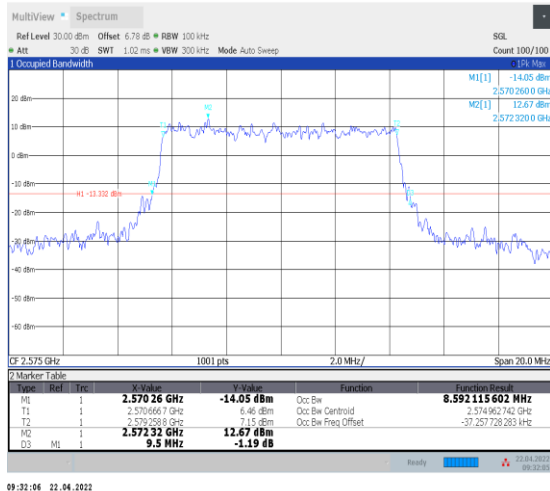
1-N38--30-10-L-3-DFT-16QAM-Outer_Full-24@0-Ant 0-8.592-9.500-≤10-PASS
