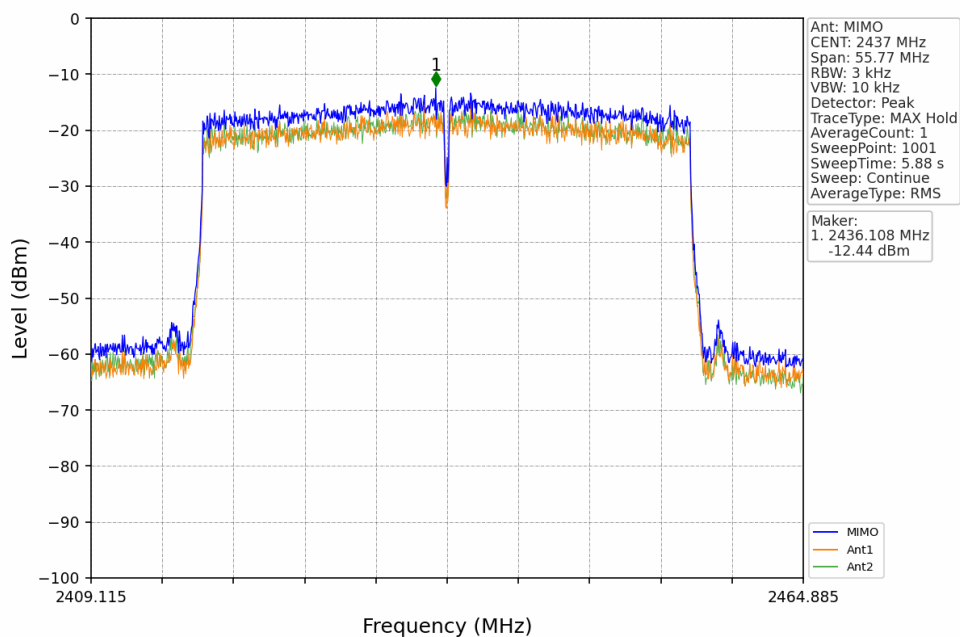
802.11ax(HEW40)_MCH_2437MHz_RU484_Left_MIMO_NTNV
