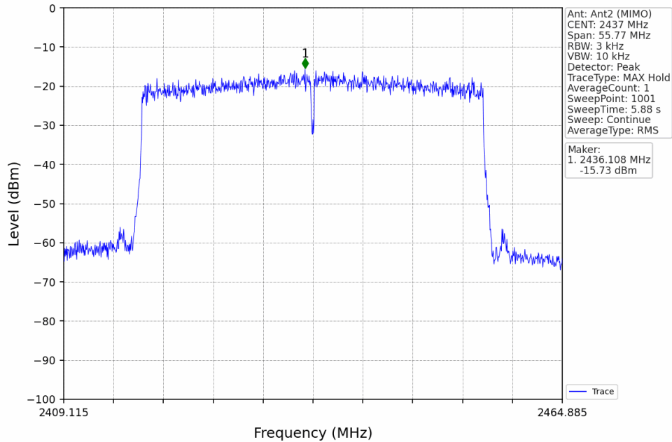
802.11ax(HEW40)_MCH_2437MHz_RU484_Left_MIMO_NTNV
