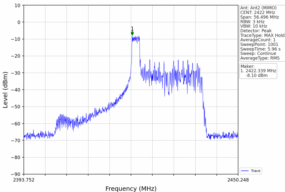
802.11ax(HEW40)_LCH_2422MHz_RU26_Mid_MIMO_NTNV
