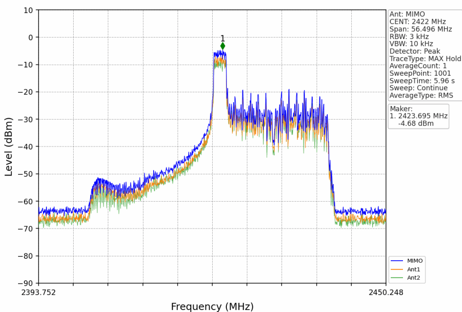
802.11ax(HEW40)_LCH_2422MHz_RU26_Mid_MIMO_NTNV
