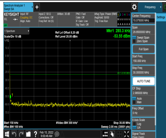
Band12-1.4MHz-16QAM-23017-1-0-Low-0.15-30--53.56-PASS
