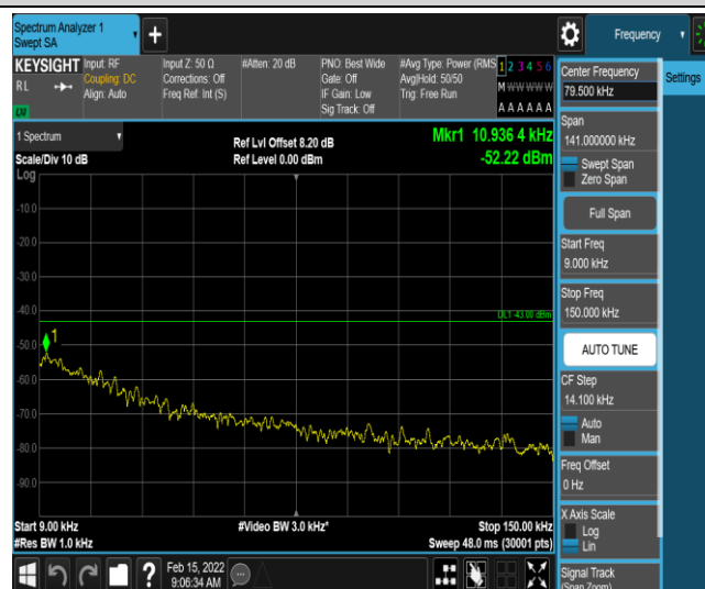
Band12-1.4MHz-16QAM-23173-1-0-High-0.009-0.15--52.22-PASS
