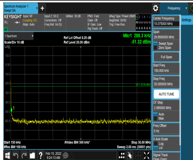
Band12-3MHz-16QAM-23095-1-0-Low-0.15-30--51.32-PASS
