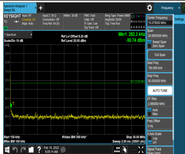
Band12-1.4MHz-QPSK-23173-1-0-High-0.15-30--50.74-PASS
