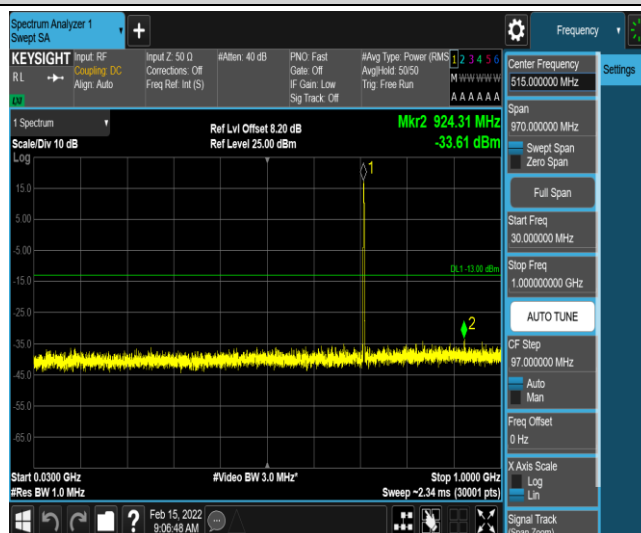
Band12-1.4MHz-16QAM-23173-1-0-High-30-1000--33.61-PASS
