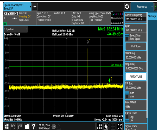
Band12-1.4MHz-16QAM-23017-1-0-Low-30-1000--34.39-PASS
