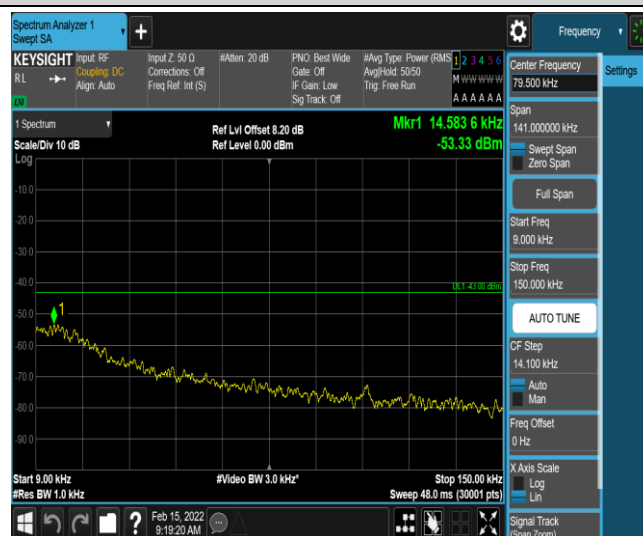
Band12-3MHz-QPSK-23025-1-0-Low-0.009-0.15--53.33-PASS
