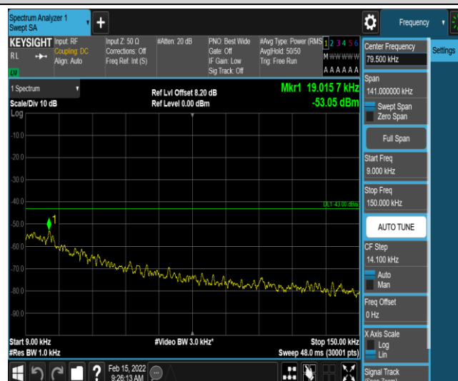
Band12-3MHz-QPSK-23165-1-0-High-0.009-0.15--53.05-PASS
