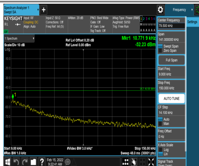
Band12-3MHz-QPSK-23095-1-0-Low-0.009-0.15--52.23-PASS
