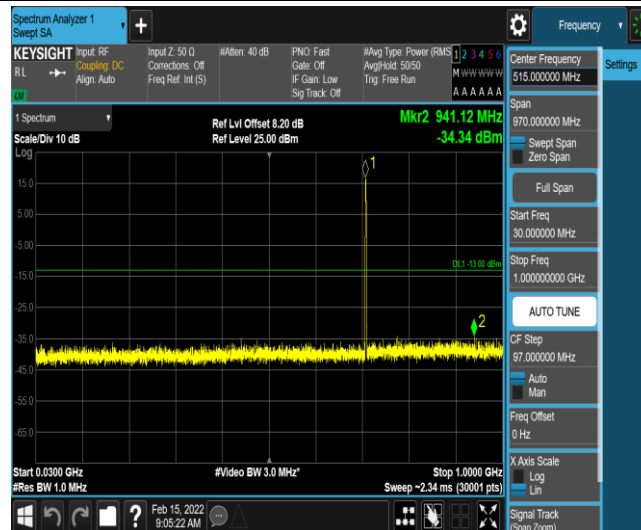
Band12-1.4MHz-QPSK-23173-1-0-High-30-1000--34.34-PASS
