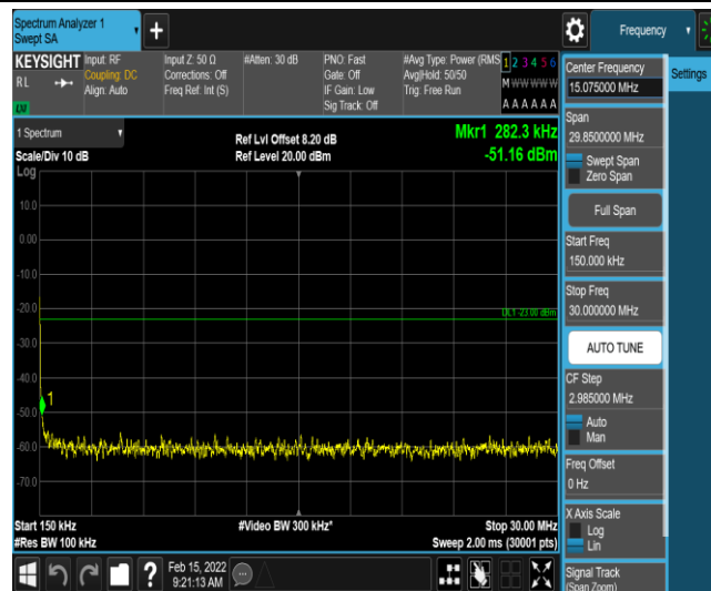
Band12-3MHz-16QAM-23025-1-0-Low-0.15-30--51.16-PASS
