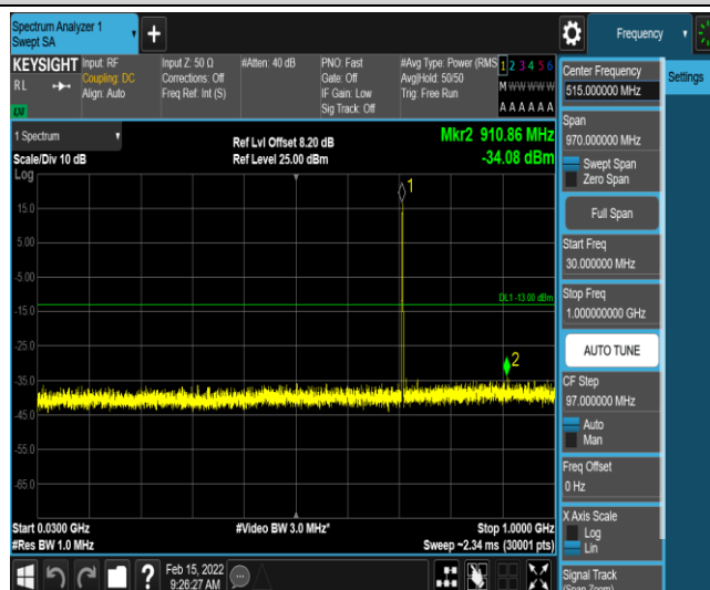
Band12-3MHz-QPSK-23165-1-0-High-30-1000--34.08-PASS
