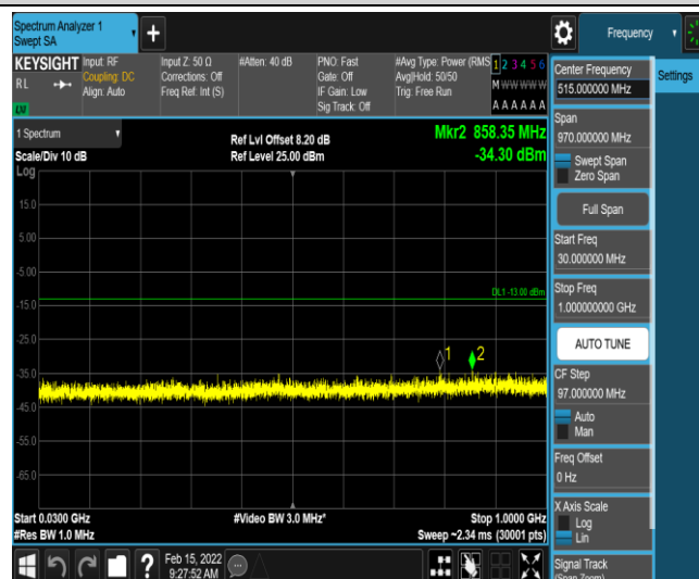
Band12-3MHz-16QAM-23165-1-0-High-30-1000--34.3-PASS
