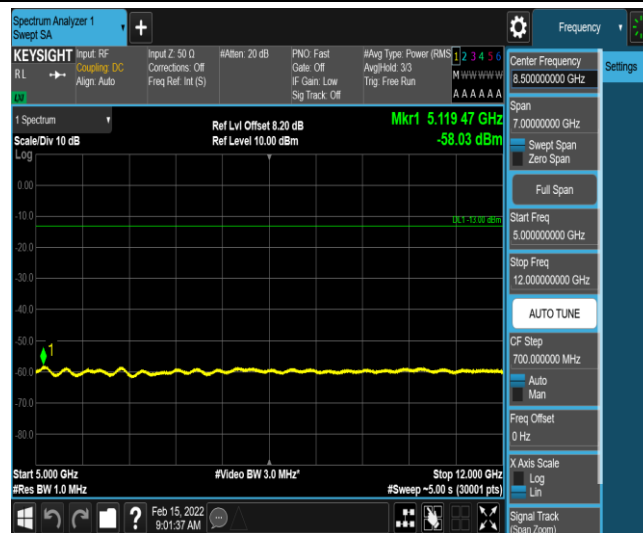
Band12-1.4MHz-16QAM-23017-1-0-Low-5000-12000--58.03-PASS
