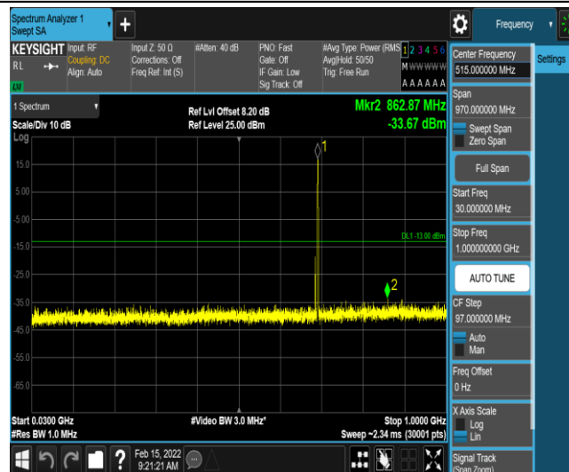
Band12-3MHz-16QAM-23025-1-0-Low-30-1000--33.67-PASS
