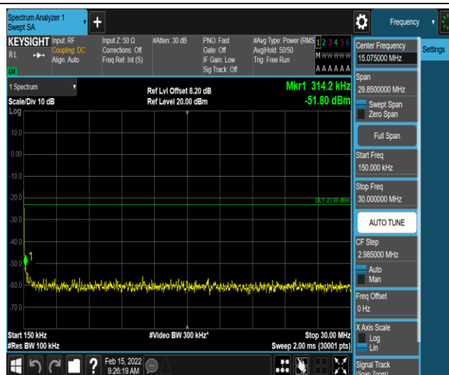
Band12-3MHz-QPSK-23165-1-0-High-0.15-30--51.8-PASS
