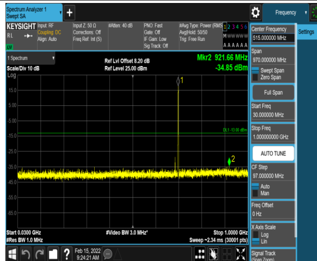
Band12-3MHz-16QAM-23095-1-0-Low-30-1000--34.85-PASS
