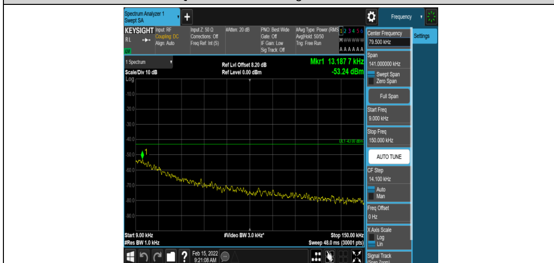
Band12-3MHz-16QAM-23025-1-0-Low-0.009-0.15--53.24-PASS
