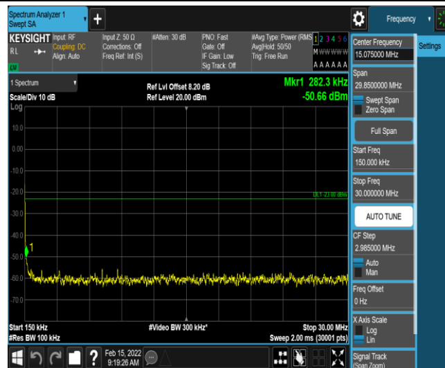
Band12-3MHz-QPSK-23025-1-0-Low-0.15-30--50.66-PASS
