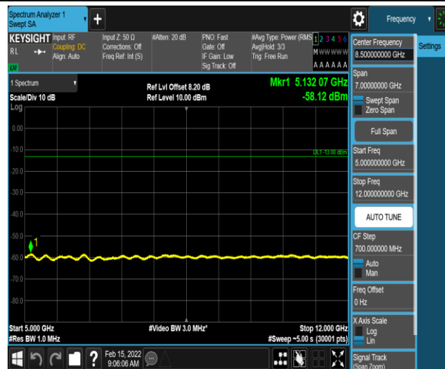
Band12-1.4MHz-QPSK-23173-1-0-High-5000-12000--58.12-PASS
