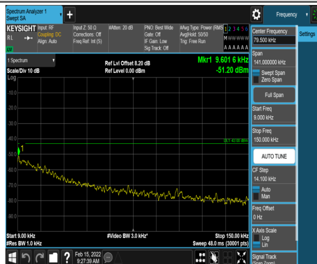
Band12-3MHz-16QAM-23165-1-0-High-0.009-0.15--51.2-PASS
