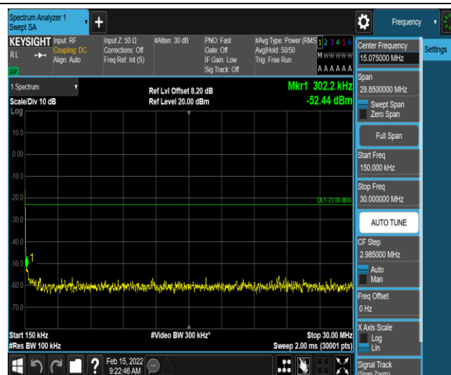
Band12-3MHz-QPSK-23095-1-0-Low-0.15-30--52.44-PASS
