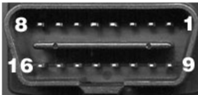
Connector on LMU-3040 side
